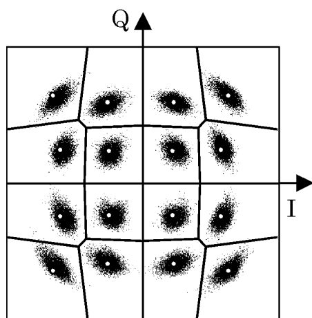
CONVENTIONAL DECISION AREA FOR 16QAM SIGNAL
