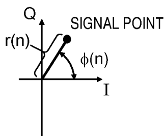
DEFINITION OF AMPLITUDE r(n) AND PHASE \phi(n)
