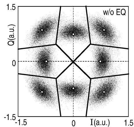
CONVENTIONAL DECISION AREA FOR 8QAM SIGNAL
