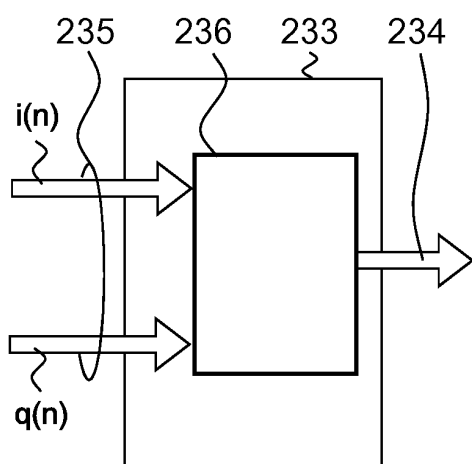
SYMBOL DECISION CIRCUIT IN THIS INVENTION
