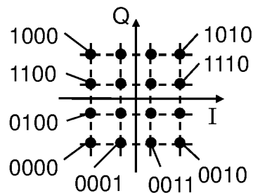
16-LEVEL QUATERNARY AMPLITUDE MODULATION (16QAM)
