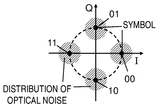
QUATERNARY PHASE SHIFT KEYING MODULATION (QPSK)
