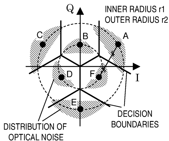
CONVENTIONAL DECISION AREA FOR 6QAM SIGNAL
