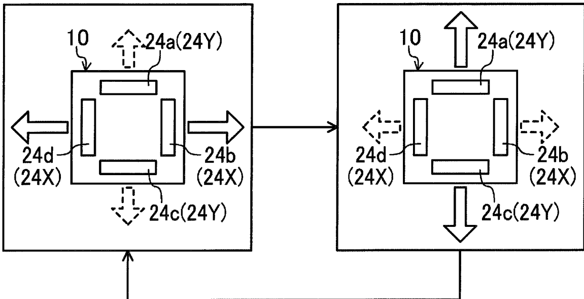
(a) FIRST PARTIAL BLOWOUT MODE
