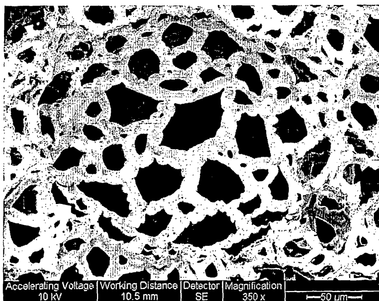
Figure 2(a) Acid form of sulphonated polymer with phase volume of 90%. Dosing time 5 minute at 300rpm, extra mixing time is 1 minute at 150 rpm. General structure showing a large coalescence pore (ca. 250 micron) surrounded by smaller primary pores (ca. 70 micron). Magnification=350
