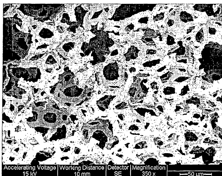
Figure 2(e). Sulphonated PolyHIPE Polymer (same as in Figure 2a) after neutralization with ammonium hydroxide showing a number of primary pores (ca. 70 micron) at Magnification= 350.
