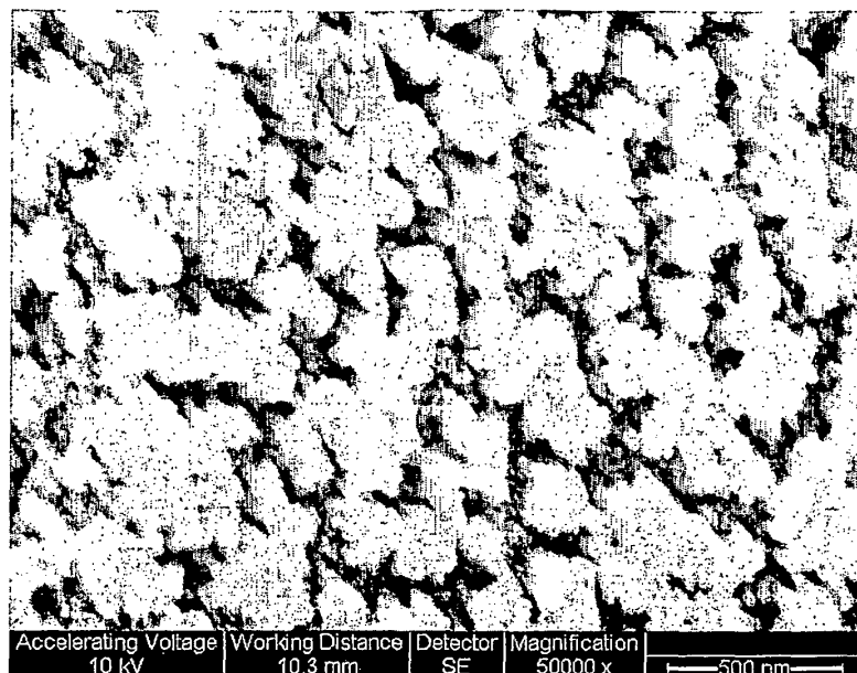
Figure 2 (d). Same as Figure 2(a) showing the nano-structure of the wall interior at Magnification= 50k.
