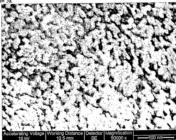
Figure2(c). Same as in Figure 2(a) showing the nano-porosity of the wall surface at Magnification= 50k
