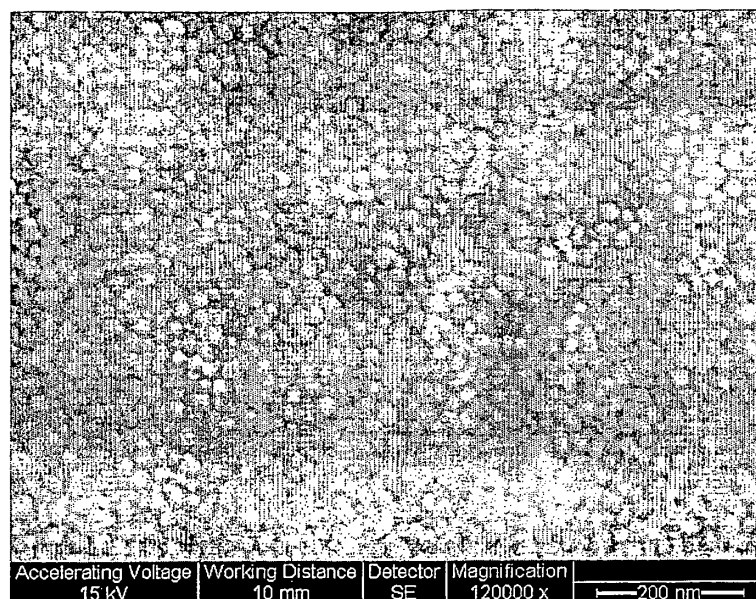
Figure 2(f). Same as in Figure 2(e), showing the nano-porosity of the surface. Note that the nano-structure is finer and porosity is reduced compared with the acid form. Magnification= 120k,
