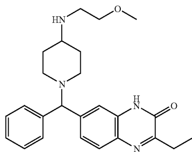
C 2 H 2 O 4 (2:5); Co. No. 2; Ex. [B2]; mp. 98° C.
