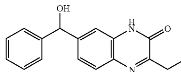
Co. No. 4; Ex. [B4]; mp. 202° C.
