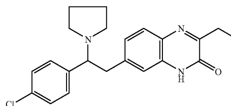
Co. No. 7; Ex. [B1]; mp. 176° C.
