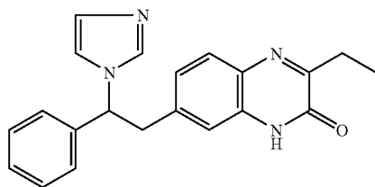
Co. No. 1; Ex. [B1]; mp. 166° C.
