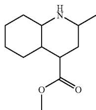
QUINOLINETRANSDECAHYDRO4METHOXYCARBONYL2METHYL
