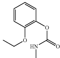
NMETHYL2ETHOXYPHENYLCARBAMATE
