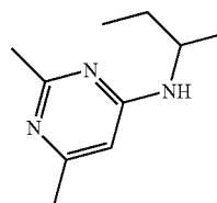
PYRIMIDINE4SECBUTYLAMINO26DIMETHYL
