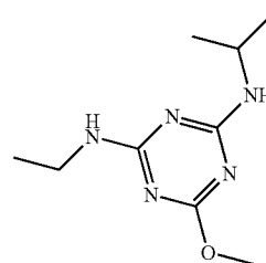
2METHOXY4ETAMINO6IPROPYLAMINOSTRIAZINE
