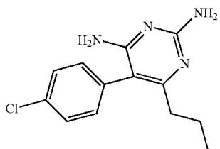
PYRIMIDINE24DIAMINO5PCHLOROPHENYL6PROPYL
