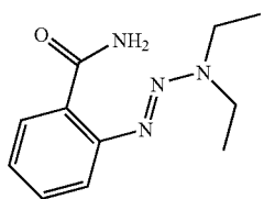
BENZAMIDE233DIETHYLTRIAZENYL
