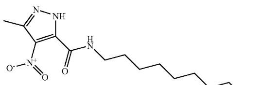
PYRAZOLE3METHYL4NITRO5NDECYLCARBOXAMIDO
