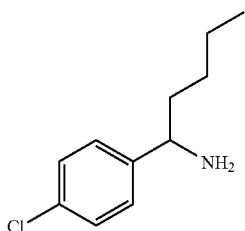
PENTYLAMINEAPCHLOROPHENYL
