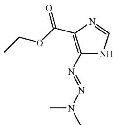
IMIDAZOLE4ETHOXYCARBONYL533DIMETHYLTRIAZENYL
