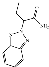
BENZOTRIAZOLE22BUTYRAMIDE
