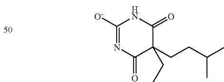
TETRABUTYLAMMONIUMAMOBARBITURATE
