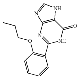
SKF96231
