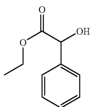
MANDELICACIDETHYLESTER
