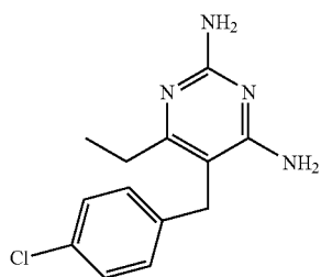
PYRIMIDINE24DIAMINO5PCHLOROBENZYL6ETHYL
