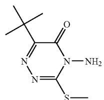
3METHIO4AMINO6TBU124TRIAZINE5ONE
