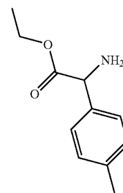
PMETHYLPHENYLGLYCINEETHYLESTER
