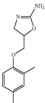
2OXAZOLINE2AMINO424DIMETHYLPHENOXYMETHYL
