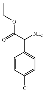
PCHLOROPHENYLGLYCINEETHYLESTER
