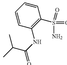
BENZENESULFONAMIDE2IBUTYROYLAMINO
