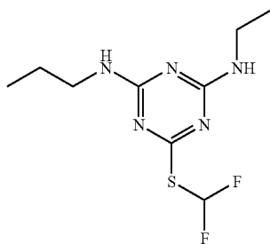
135TRIAZINE2DIFLUOROMETHIO4PROPYLAMINO6ETHYLAMINO
