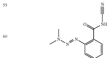
NCYANO233DIMETHYL1TRIAZENOBENZAMIDE
