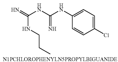
N1PCHLOROPHENYLN5PROPYLBIGUANIDE
