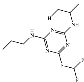
135TRIAZINE2DIFLUOROMETHIO41PROPYLAMINO6PROPYLAMINO
