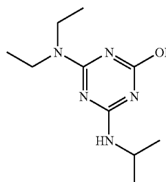
2OH4IPROPYLAMINO6DIETAMINOSTRIAZINE
