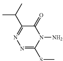
3METHIO4AMINO6IPRI124TRIAZINE5ONE
