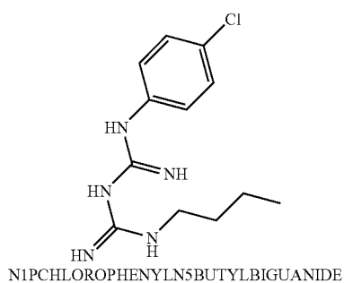
N1PCHLOROPHENYLN5BUTYLBIGUANIDE
