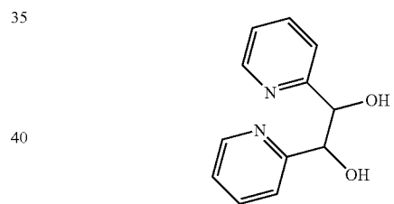
ETHYLENEGLYCOL12BIS2PYRIDYL
