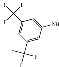
35BISTRIFLUOROMETHYLANILINE
