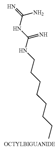
OCTYLBIGUANIDE
