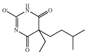
DIETPROTRIPTYLINESALTAMOBARBITAL
