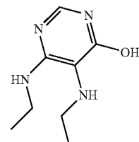
PYRIMIDINE45BIETHYLAMINO6HYDROXY
