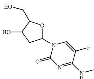
5FLUORONMETHYL2DEOXYCYTIDINE
