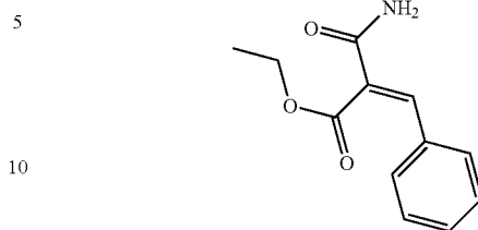
AAMIDOETHYLCINNAMATE
