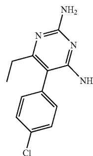
PYRIMETHAMINE
