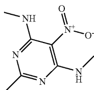
PYRIMIDINE2METHYL46BISMETHYLAMINO5NITRO
