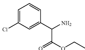
MCHLOROPHENYLGLYCINEETHYLESTER
