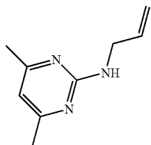
PYRIMIDINE2ALLYLAMINO46DIMETHYL
