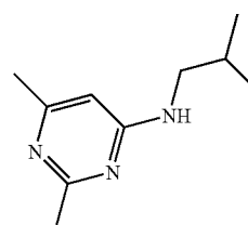
PYRIMIDINE41BUTYL26DIMETHYL
