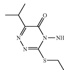
3ETHYLTHIO4AMINO6IPR124TRIAZINE5ONE
