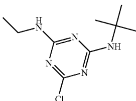
TERBUTHYLAZINE
