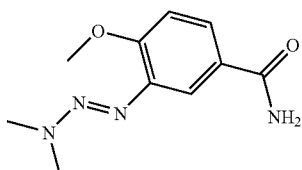
4METHOXY333DIMETHYLTRIAZENOBENZAMIDE
