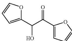
FURAN2CHOHCOFURYL
