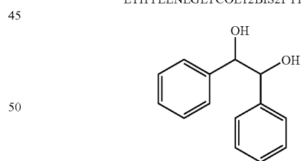
ETHYLENEGLYCOL12DIPHENYL
