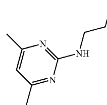
PYRIMIDINE46DIMETHYL2PROPYLAMINO
