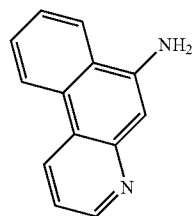
PHENANTHRIDINE6AMINO
