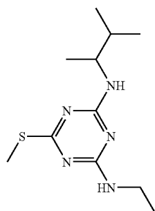
DIMETHAMETRYN
