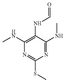
PYRIMIDINE5FORMAMIDO46BISMETHYLAMINO2METHYLTHIO
