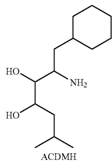
ACDMH
