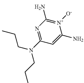
2,4DIAMINO6DIPROPYLAMINOPYRIMIDINE3OXIDE
