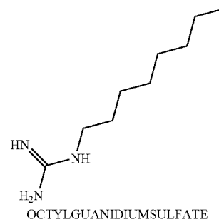
OCTYLGUANIDIUMSULFATE
