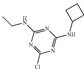
SIMAZINE2CYCLOBUTYLAMINEANALOG
