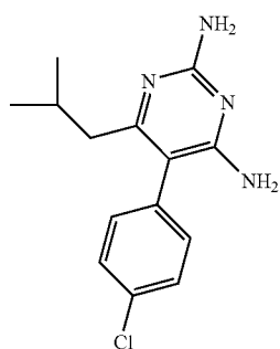
PYRIMIDINE24DIAMINO5PCHLOROPHENYL6IBUTYL
