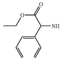
PHENYLGLYCINEETHYLESTER
