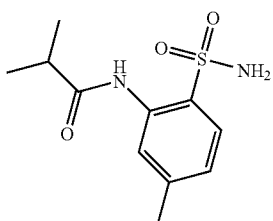
BENZENESULFONAMIDE2IBUTYLROYLAMINO4METHYL
