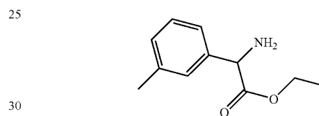
MMETHYLPHENYLGLYCINEETHYLESTER
