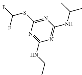
135TRIAZINE2DIFLUOROMETHIO41PROPYLAMINO6ETHYLAMINO
