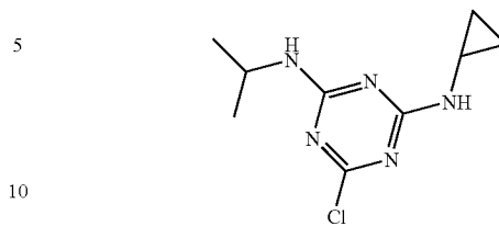
CYPRAZINE
