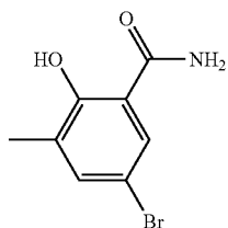
BENZAMIDE2HYDROXY3METHYL5BROMO
