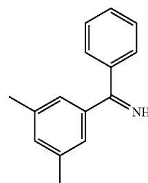
BENZENEMETHANIMINE35DIMETHYLAPHENYL
