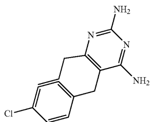
PYRIMIDINE24DIAMINO5PCHLOROBENZYL6PROPYL
