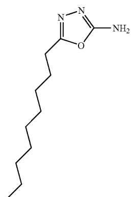
2AMINO5NONYL134OXADIAZOLE
