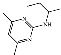
PYRIMIDINE2SECBUTYLAMINO46DIMETHYL
