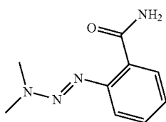
233DIMETHYL1TRIAZINOBENZAMIDE
