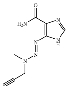
IMIDAZOLE5CARBOXAMIDE43METHYL3PROPYNYLTRIAZENYL
