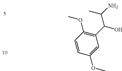
METHOXAMINE
