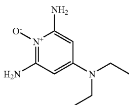
24DIAMINO6DIETHYLAMINOPYRIMIDINE3OXIDE
