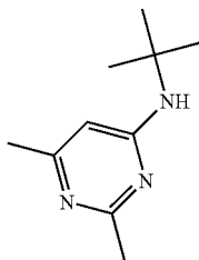
PYRIMIDINE4TBUTYLAMINO26DIMETHYL
