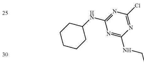
SIMAZINE2CYCLOHEXYLAMINEANALOG
