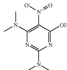
PYRIMIDINE24BISDIMETHYLAMINO6HYDROXY5NITRO
