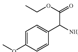
PMETHOXYPHENYLGLYCINEETHYLESTER
