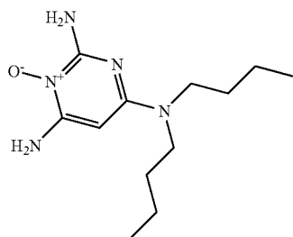
2,4DIAMINO6DIBUTYLAMINOPYRIMIDINE3OXIDE
