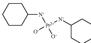
PLATINUMBISCYCLOHEXYLAMMONIODIAQUADINITRATE
