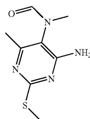
PYRIMIDINE4AMINO6METHYL5METHYL FORMAMIDO2METHYLTHIO
