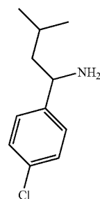
IPENTYLAMINE4CHLOROPHENYL
