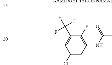
ACETANILIDE2FLUORO3TRIFLUOROMETHYL5CHLORO
