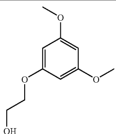
FLOVERINE
