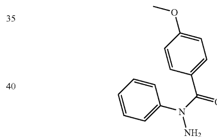
N1PHENYLN1PMETHOXYBENZOYLHYDRAZINE
