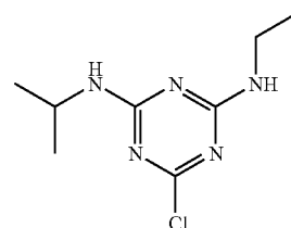
ATRAZINE
