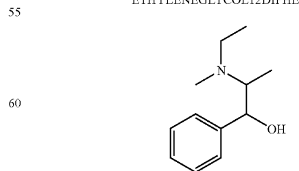
ETHYLEPHEDRINE
