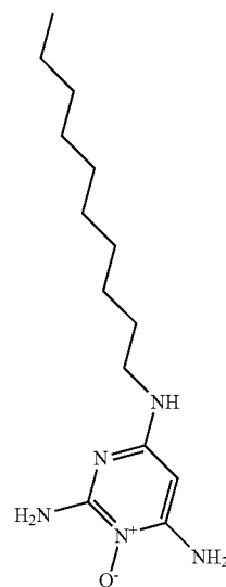
24DIAMINO6DECYLAMINOPYRIMIDINE3OXIDE
