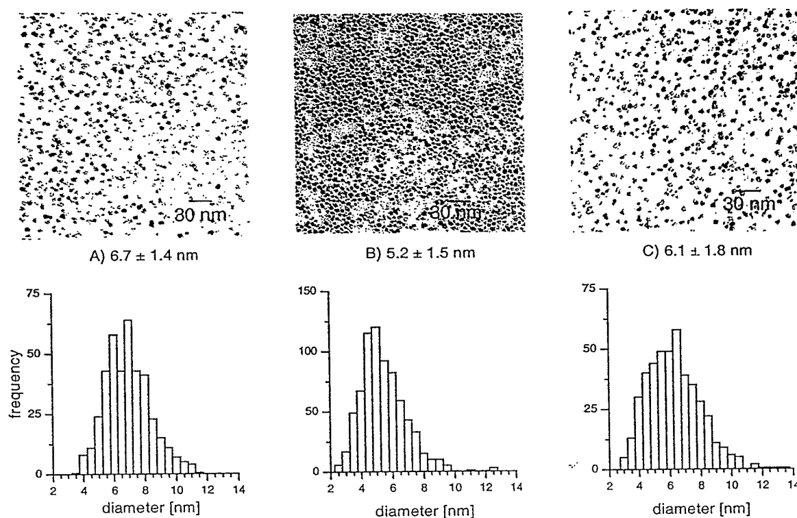
Figure 4 Low-resolution TEM images and respective diameter histograms of samples prepared under different conditions: A) Injection of 4 ml 0.3 M \text{FeCuP}_3 / octylamine into 7 g trioctylamine at 300 °C and refluxing at 225 °C for 30 min. B) Injection of 4 ml 0.3 M \text{FeCuP}_3 / octylamine into 7 g trioctylamine at 250 °C and refluxing at 200 °C for 30 min. C) Injection of 4 ml 0.3 M \text{FeCuP}_3 / octylamine into 7 g trioctylamine at 250 °C and refluxing at 200 °C for 5 min, then, additional injection of 2 ml stock solution and refluxing for 25 min at 200 °C.
