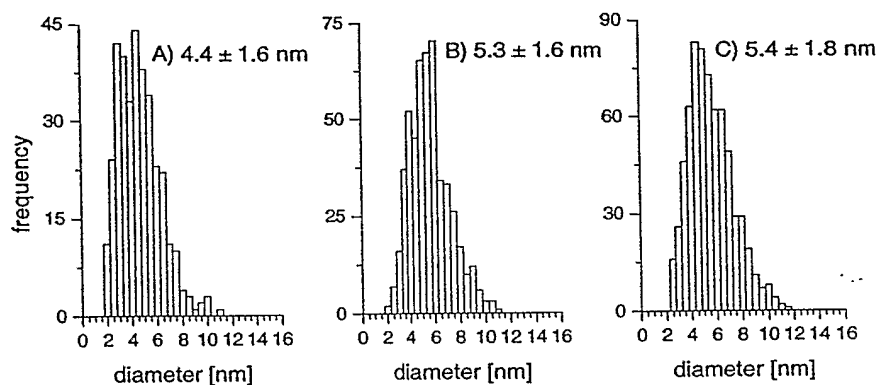
Figure 5 The time evolution of the particle size during refluxing at 200 °C as determined from low-resolution TEM imaging of aliquots taken at specific times from the reaction solution: A) 0 min after injection. B) 10 min after injection C) 30 min after injection of 4 ml 0.3 M FeCup 3 / octylamine into 7 g trioctylamine at 250 °C.
