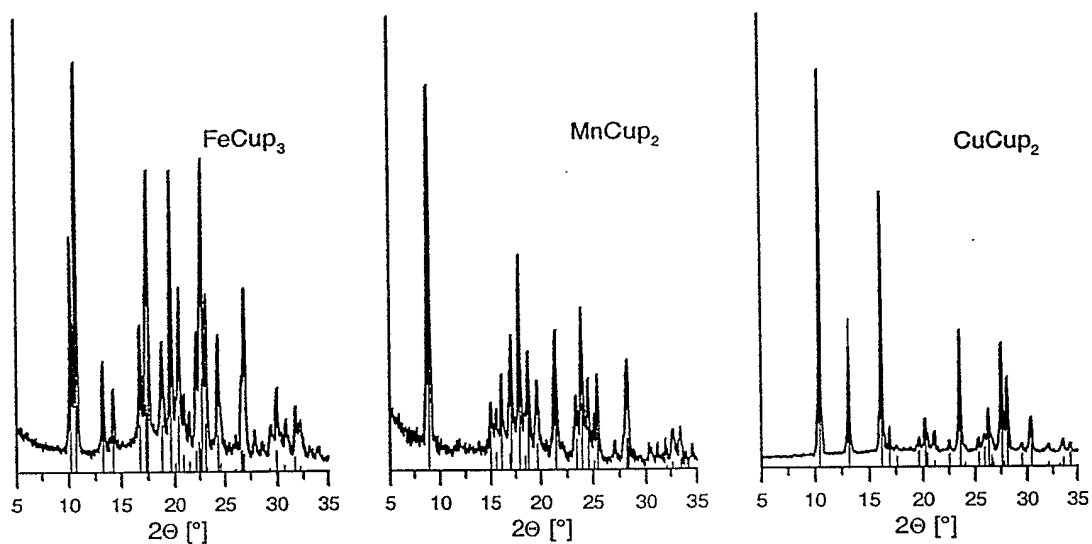
Figure 8 Powder XRDs ( \text{Cu K}\alpha radiation) of metal cupferronates.
