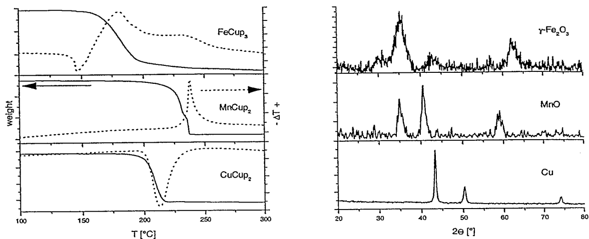
Figure 1 Left) Thermogravimetric analysis and Differential Thermal Analysis of powders of \text{FeCuP}_3 , \text{MnCuP}_2 and \text{CuCuP}_2 . Right) Powder x-ray diffraction patterns (Cu K_{\alpha} radiation) of the respective decomposition products.
