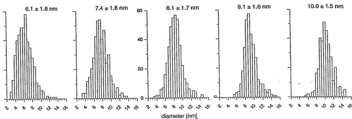
Figure 6 Size evolution of \gamma\text{-Fe}_2\text{O}_3 nanocrystals isolated by subsequent extractions of the reaction precipitate with toluene. The reaction conditions were as described in fig. 4C).
