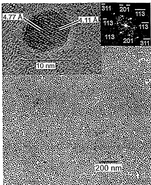
Figure 7 Low-resolution TEM image of a monolayer of individual \gamma\text{-Fe}_2\text{O}_3 nanocrystals ( 10.0 \pm 1.5 nm) covering an area bigger than 2 \mu\text{m}^2 . Top left: High-resolution TEM image of one of the nanocrystals in this sample. The indicated lattice plane distances correspond to the (113) and (201) lattice planes of tetragonal \gamma\text{-Fe}_2\text{O}_3 with ordered superlattice of the cation vacancies. Top right: FFT of the high-resolution TEM image looking down the [51-2] zone-axis.
