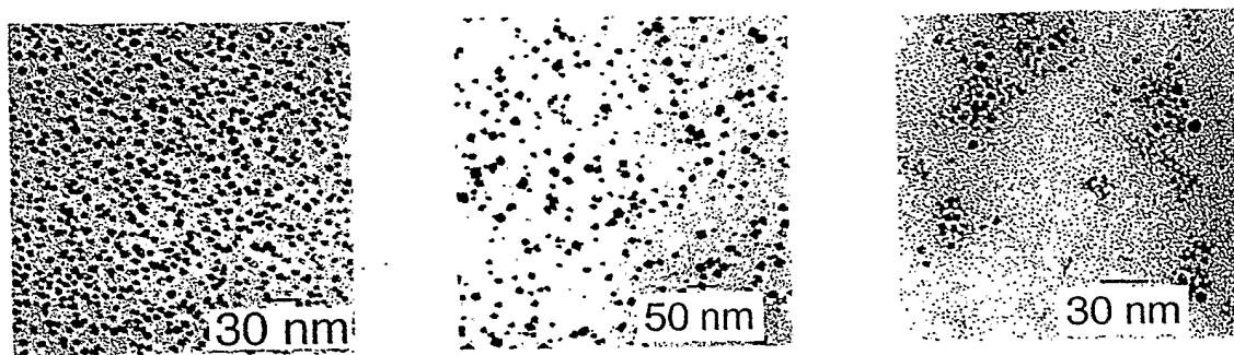
Figure 2 Low-resolution TEM images of \gamma\text{-Fe}_2\text{O}_3 (left), \text{Mn}_3\text{O}_4 (middle) and \text{Cu}_2\text{O} (right) nanocrystals. The average particle sizes and standard deviations are 6.7 \pm 1.4 nm for \gamma\text{-Fe}_2\text{O}_3 , 12.0 \pm 4.7 nm for \text{Mn}_3\text{O}_4 and 6.9 \pm 2.5 nm for \text{Cu}_2\text{O} .
