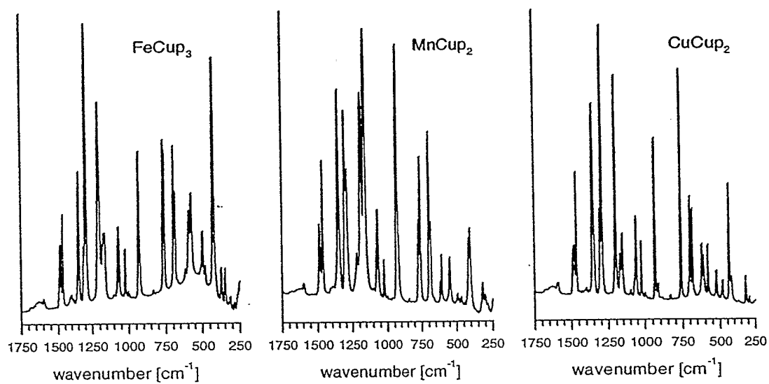
Figure 9 FT-IR spectra of metal cupferron complexes in KBr.
