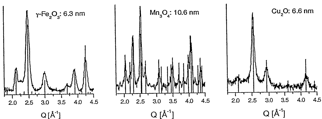
Figure 3 XRD patterns of \gamma\text{-Fe}_2\text{O}_3 (left), \text{Mn}_3\text{O}_4 (middle) and \text{Cu}_2\text{O} (right) nanocrystals and expected lattice reflections of the respective bulk phases.
