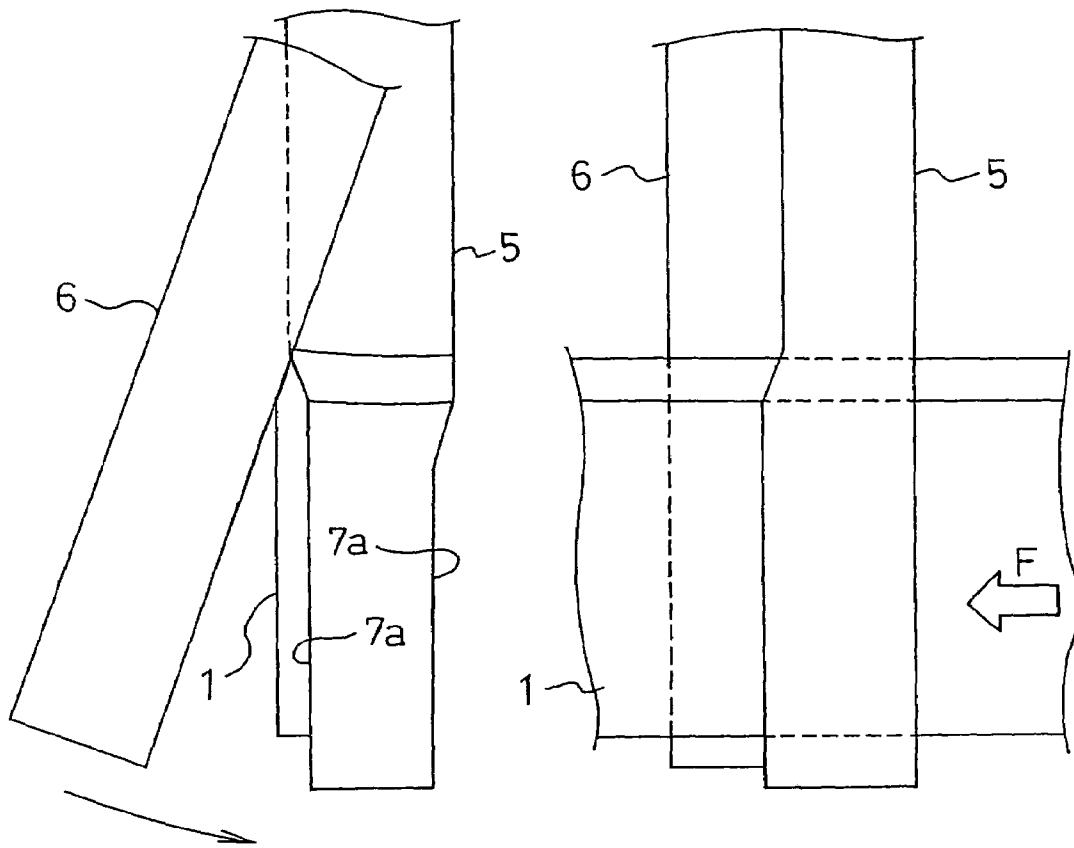
Fig. 55 (PRIOR ART) Fig. 56 (PRIOR ART)
