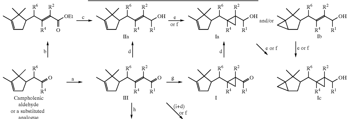
Scheme 1. Access to cyclopropanated campholenic aldehyde derivatives Ia-e
