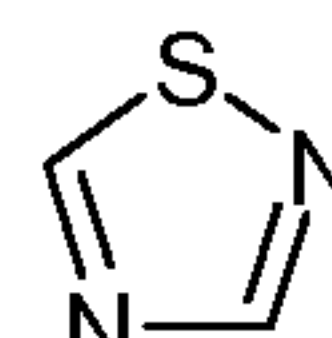
1-thia-2,4-diazole (1-thia-2,4-diazolyl)
