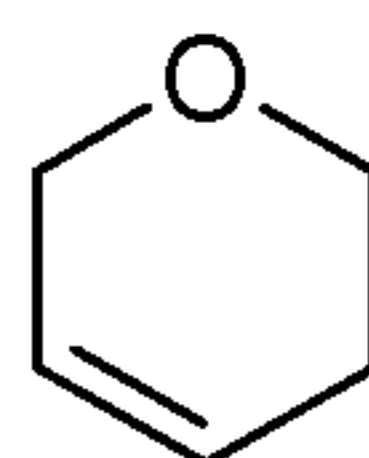
5,6-dihydro-2H-pyran (5,6-dihydro-2H-pyranyl)
