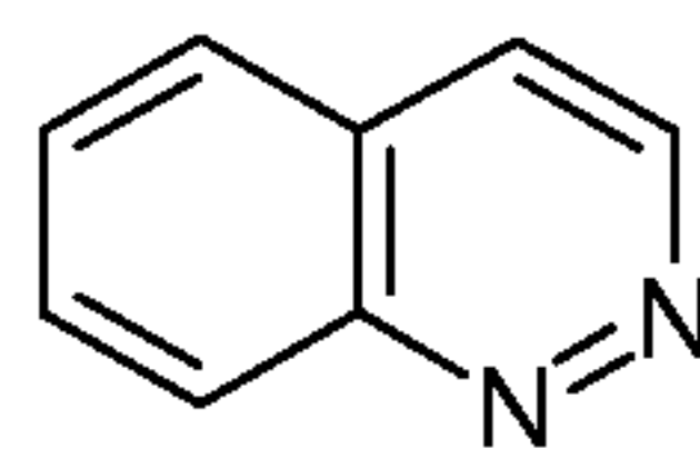
cinnoline (cinnolinyl)
