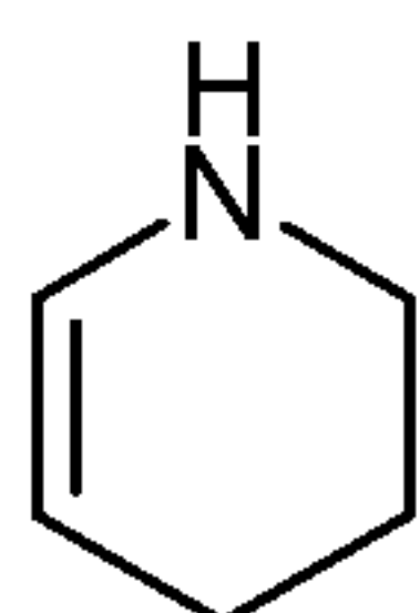
1,2,3,4-tetrahydropyridine (1,2,3,4-tetrahydropyridinyl)
