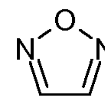
1-oxa-2,5-diazole (1-oxa-2,5-diazolyl)
