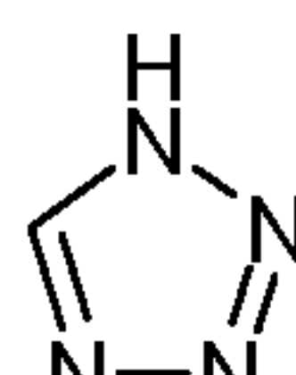
tetrazole (tetrazolyl)
