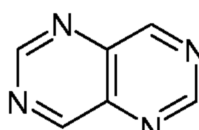
pyrimido[5,4-d]pyrimidine (pyrimido[5,4-d]pyrimidinyl)
