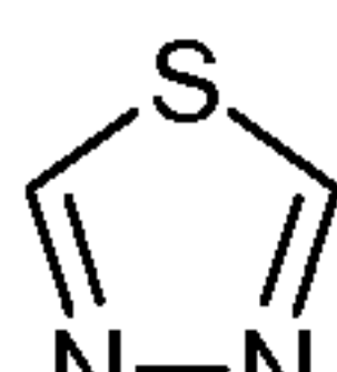
1-thia-3,4-diazole (1-thia-3,4-diazolyl)
