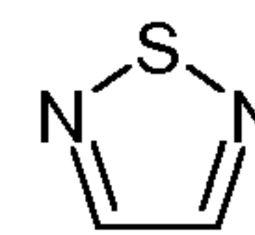
1-thia-2,5-diazole (1-thia-2,5-diazolyl)
