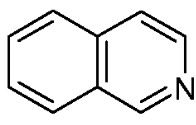
isoquinoline (isoquinolinyl)
