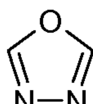
1-oxa-3,4-diazole (1-oxa-3,4-diazolyl)
