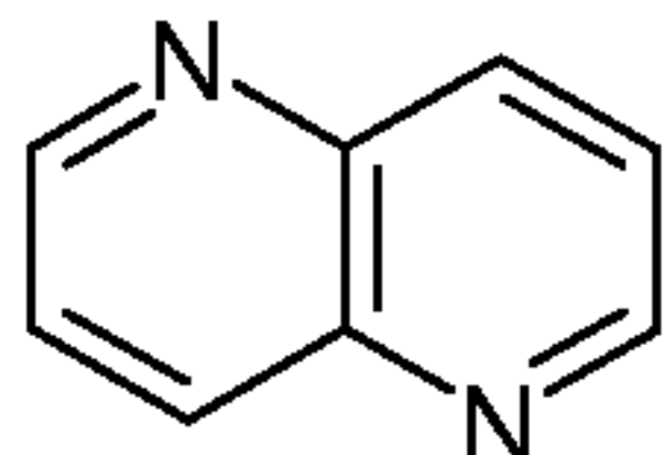
1,5-naphthyridine (1,5-naphthyridinyl)
