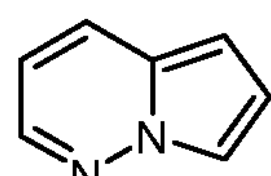
pyrrolo[1,2-b]pyridazine (pyrrolo[1,2-b]pyridazinyl)
