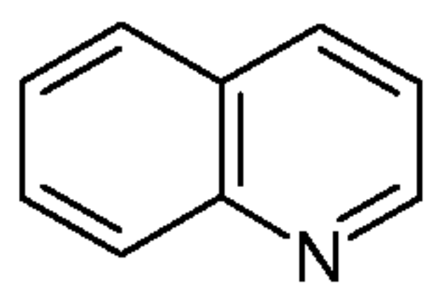
quinoline (quinolinyl)
