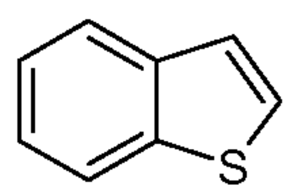
benzothiophene (benzothiophenyl)
