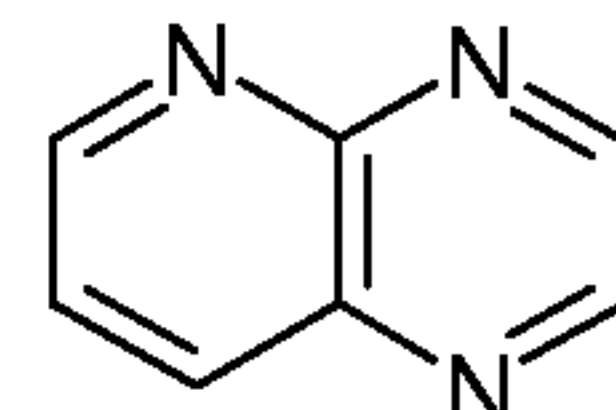
pyrido[2,3-b]pyrazine (pyrido[2,3-b]pyrazinyl)
