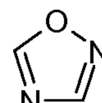
1-oxa-2,4-diazole (1-oxa-2,4-diazolyl)
