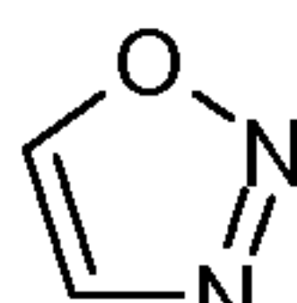
1-oxa-2,3-diazole (1-oxa-2,3-diazolyl)
