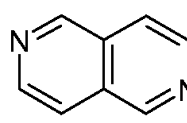
2,6-naphthyridine (2,6-naphthyridinyl)
