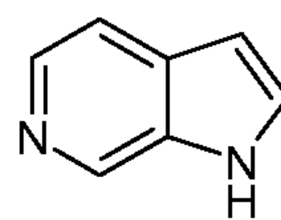
pyrrolo[2,3-c]pyridine (pyrrolo[2,3-c]pyridinyl)
