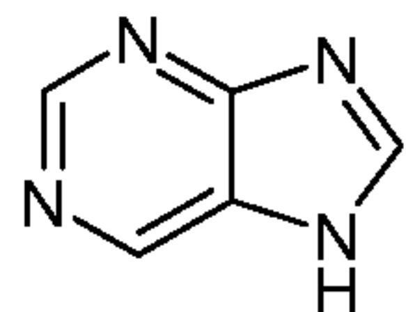
purine (purinyl)
