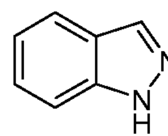
indazole (indazolyl)
