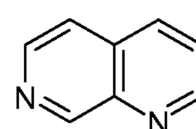
1,7-naphthyridine (1,7-naphthyridinyl)
