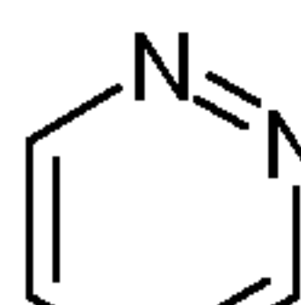
pyridazine (pyridazinyl)
