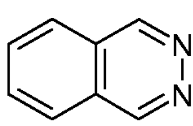
phthalazine (phthalazyl)
