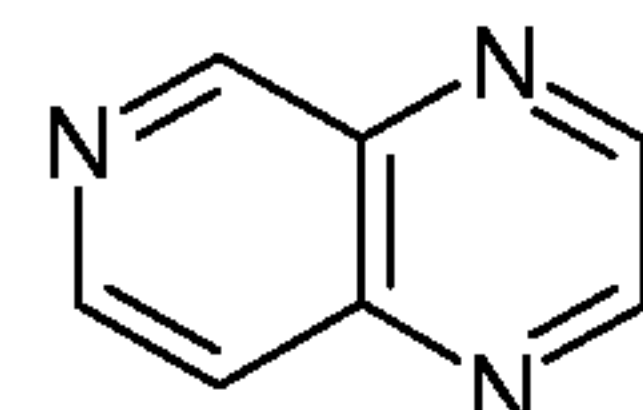
pyrido[3,4-b]pyrazine (pyrido[3,4-b]pyrazinyl)
