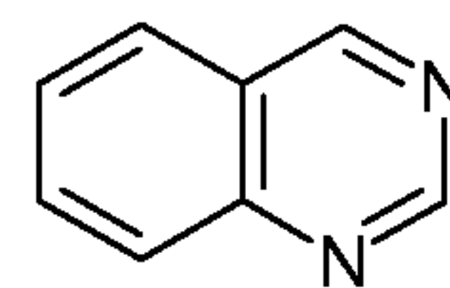
quinazoline (azaquinazoline)
