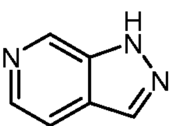
pyrazolo[3,4-c]pyridine (pyrazolo[3,4-c]pyridinyl)
