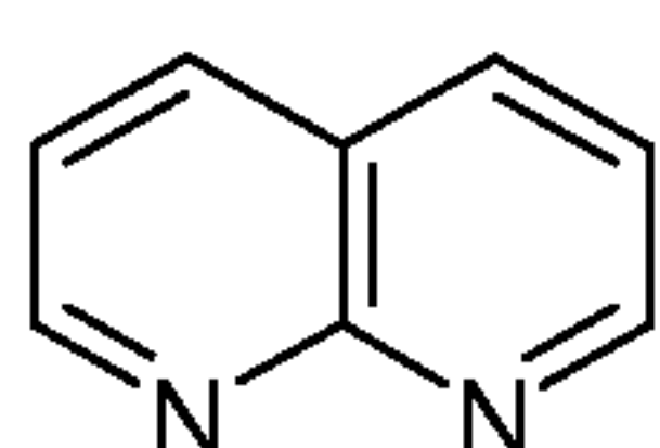
1,8-naphthyridine (1,8-naphthyridinyl)
