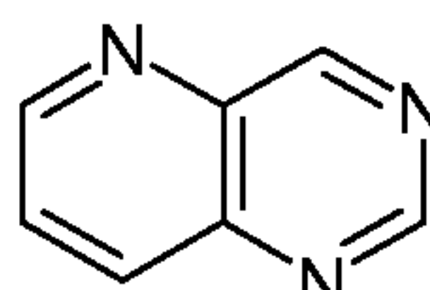
pyrido[3,2-d]pyrimidine (pyrido[3,2-d]pyrimidinyl)
