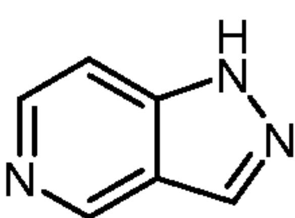
pyrazolo[4,3-c]pyridine (pyrazolo[4,3-c]pyridinyl)
