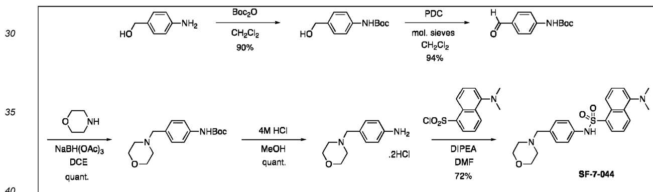
Scheme 5
