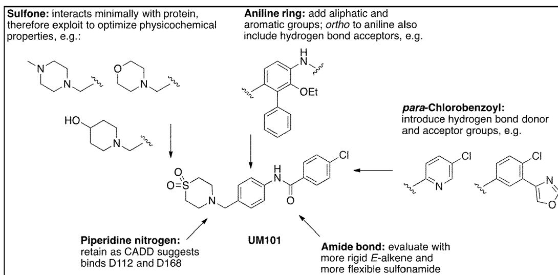
Scheme 2
