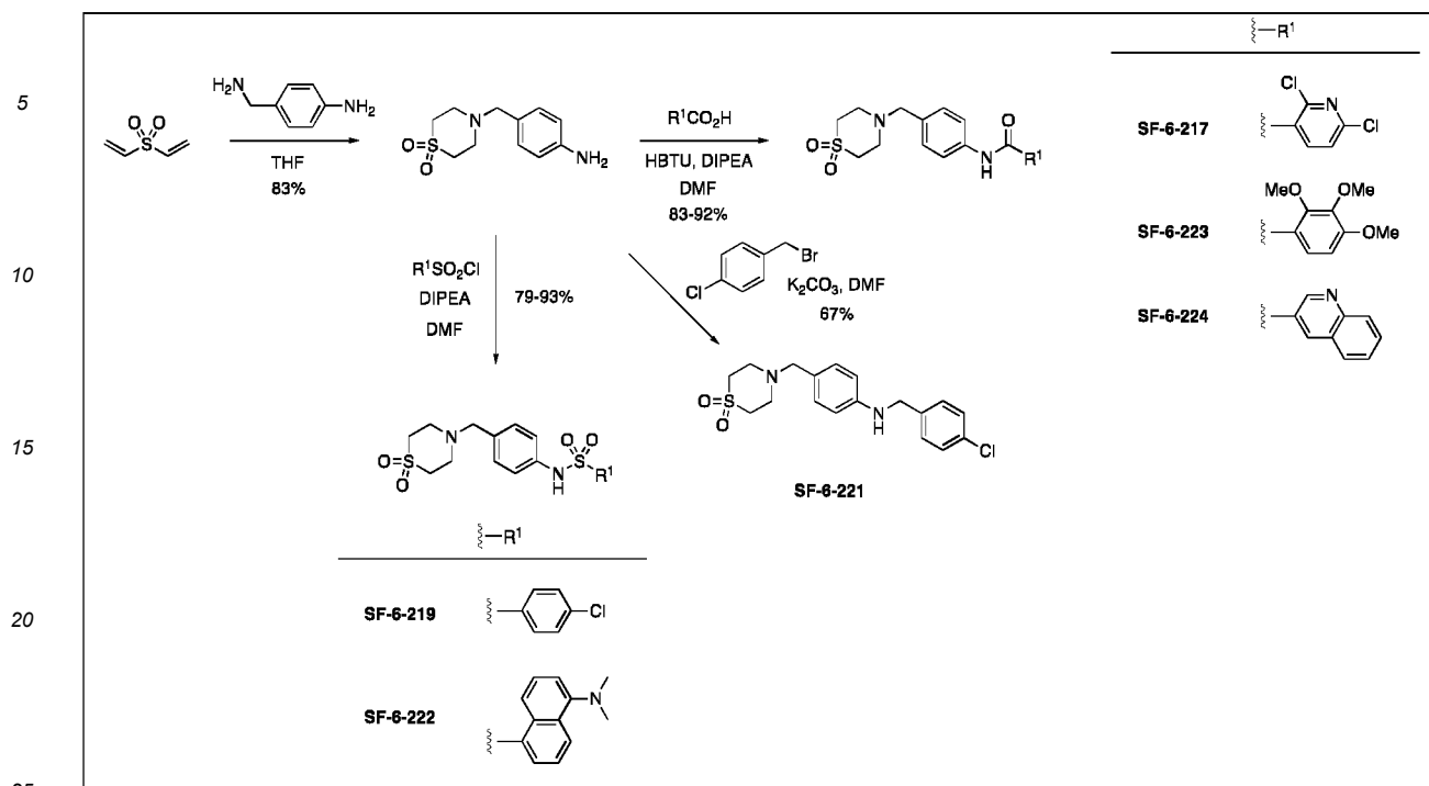
Scheme 4
