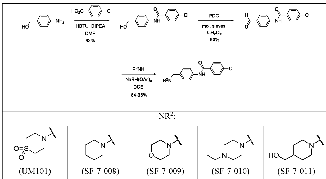
Scheme 3
