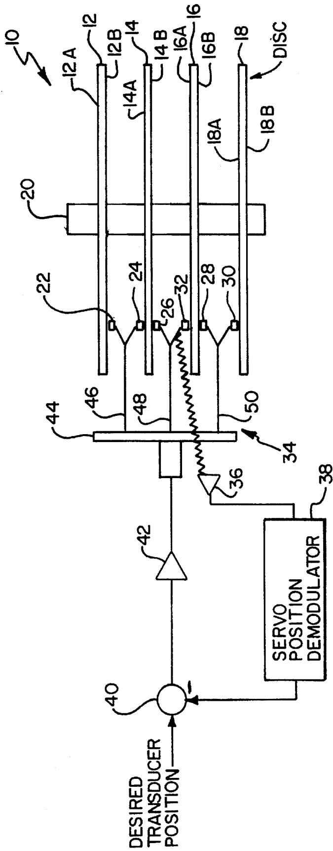
Fig. 1 PRIOR ART
