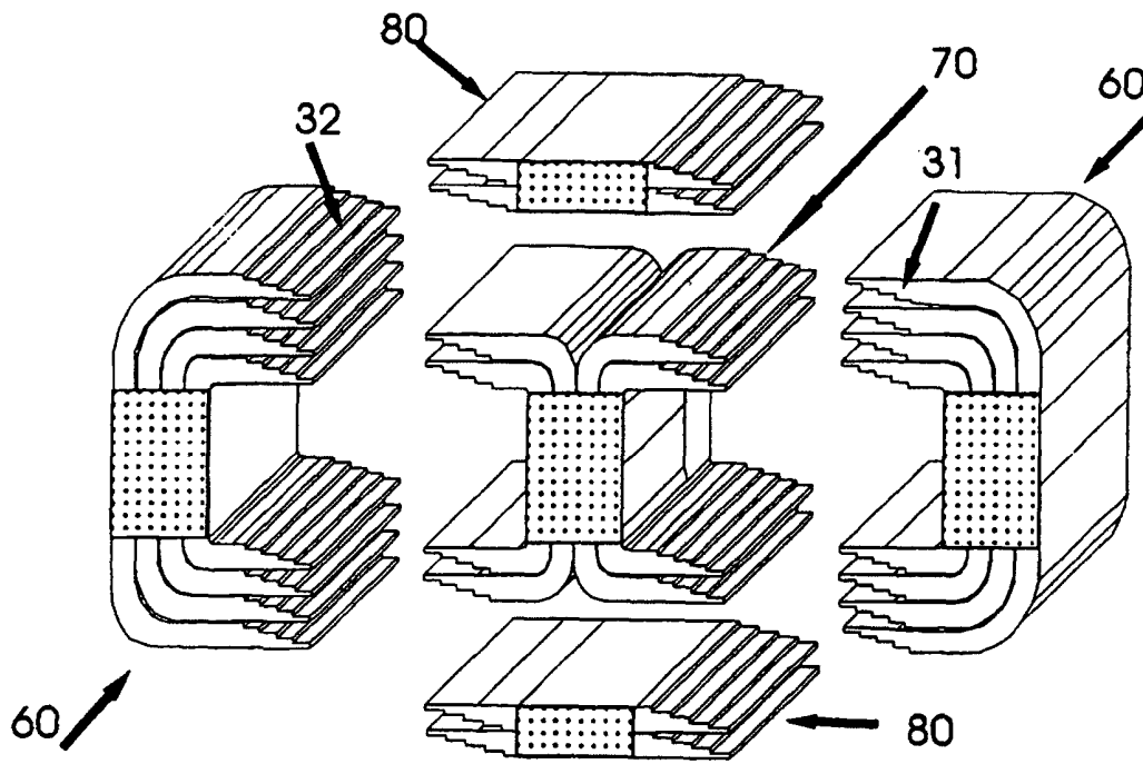
3 Phase / 3 Leg Transformer Core (110)
