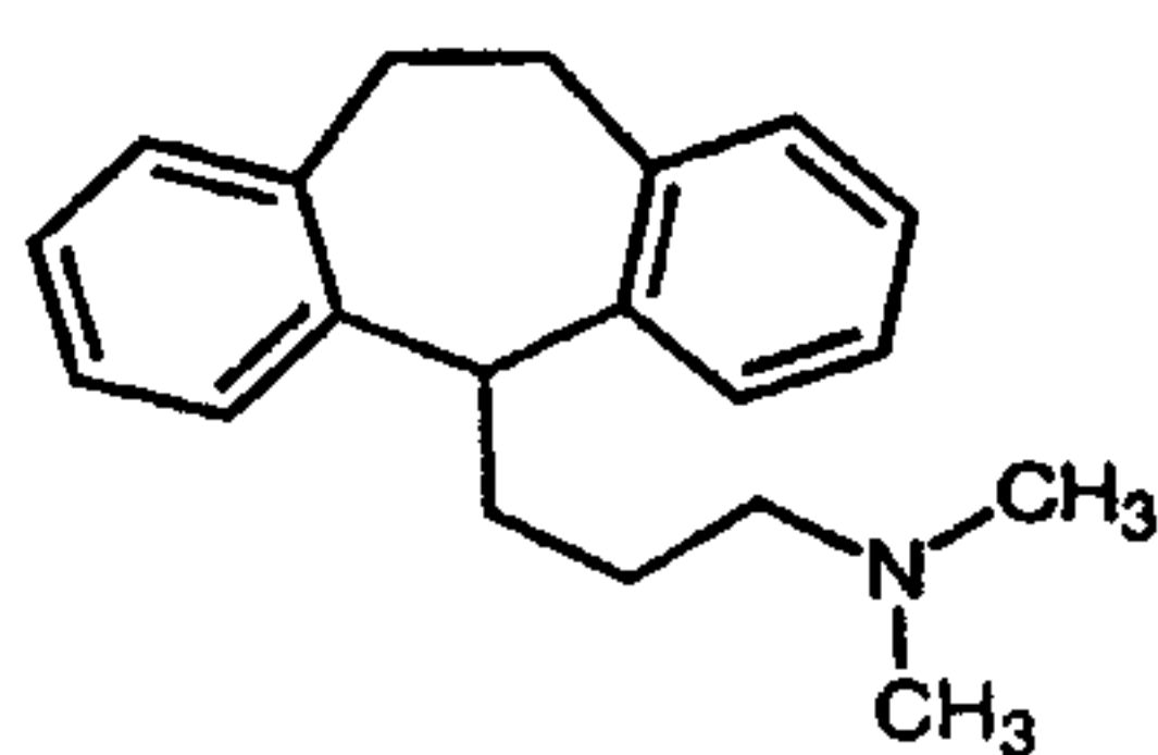
Imipramine (4c)
