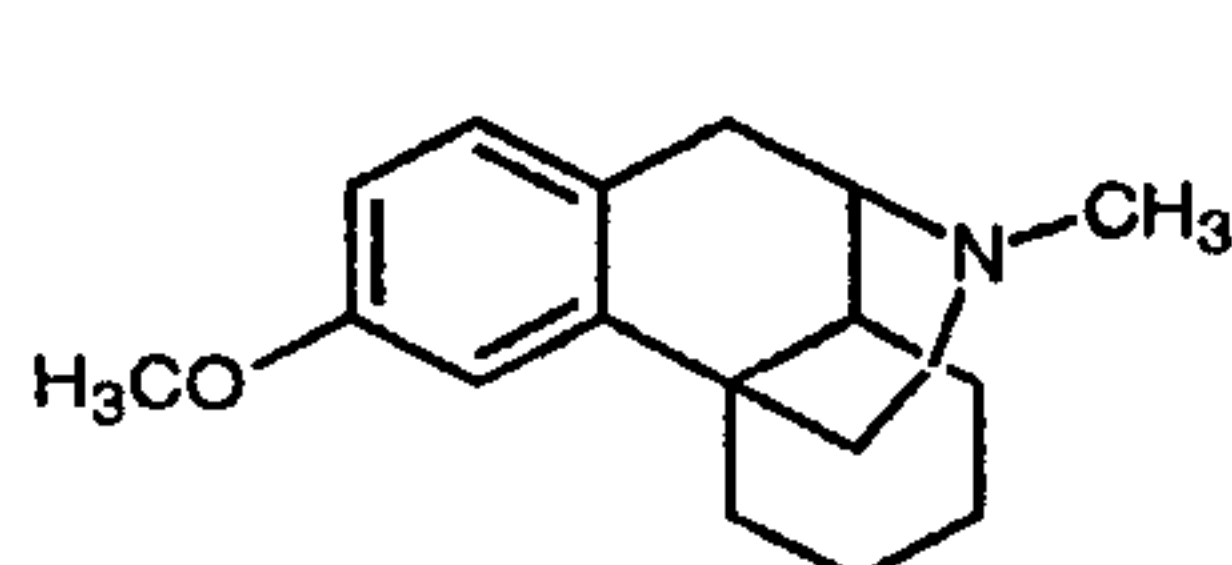
Dextromethorphan (8)
