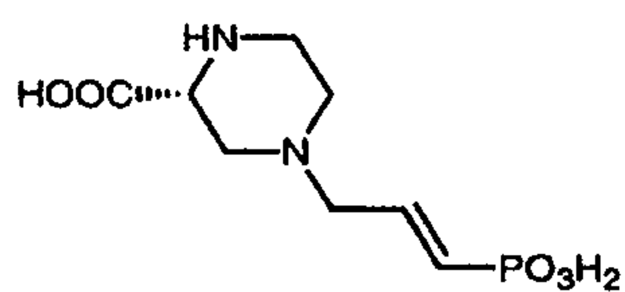
(R)-CPPene (3)
