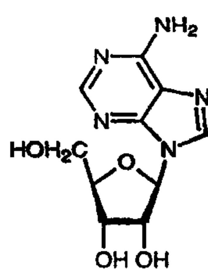
Adenosine (56a)
