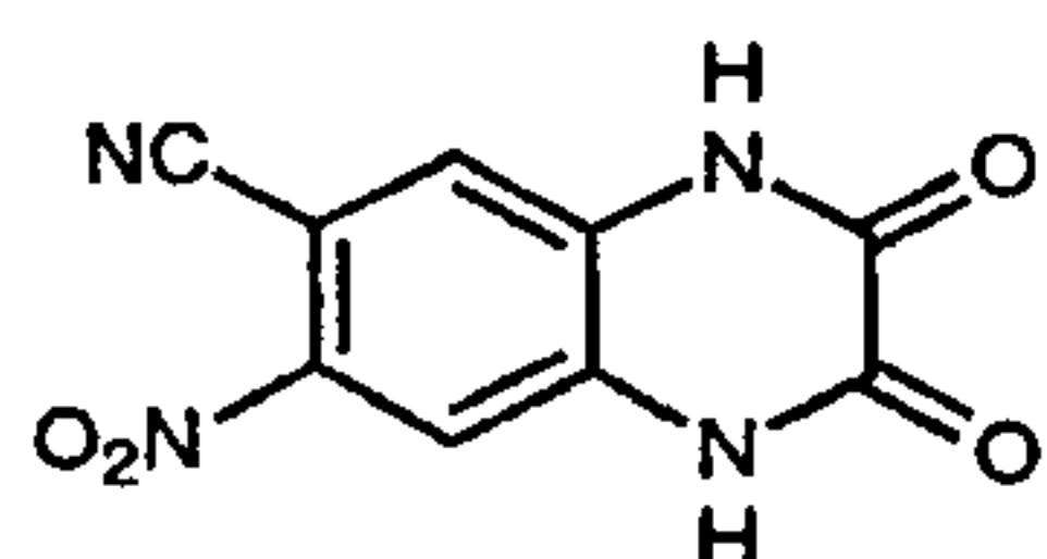
CNQX (19)
