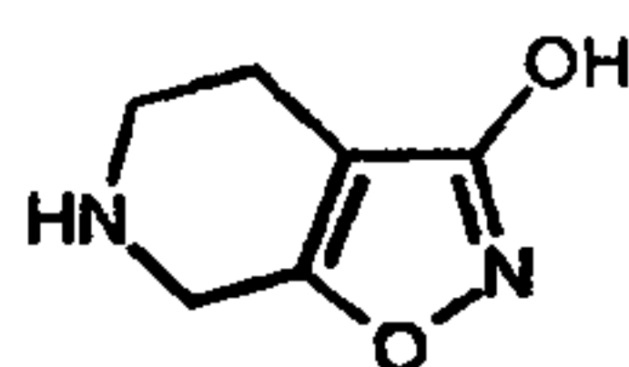
THIP (49)
