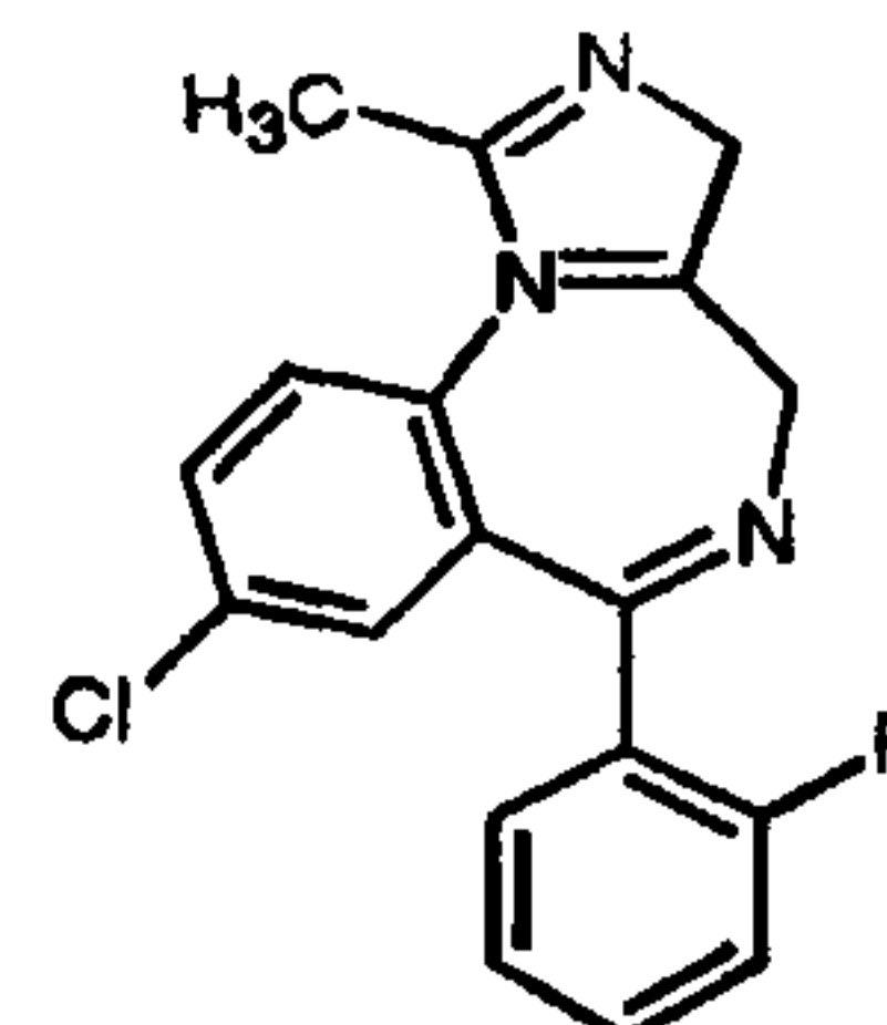
Midazolam (49a)
