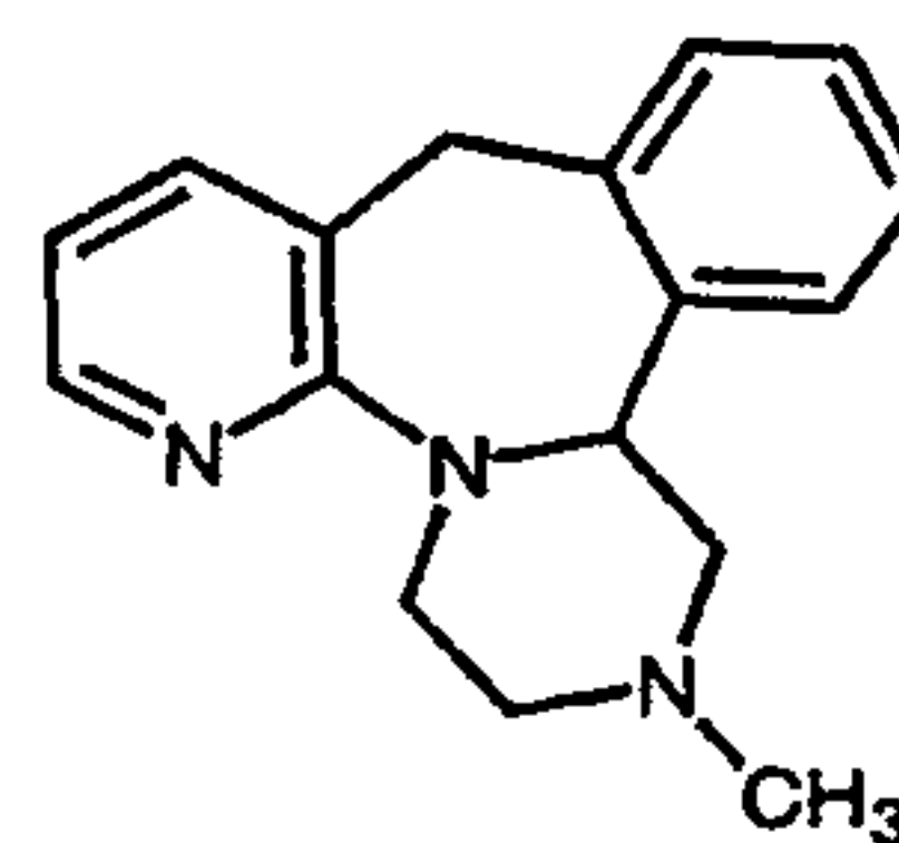
Mirtazapine (4e)
