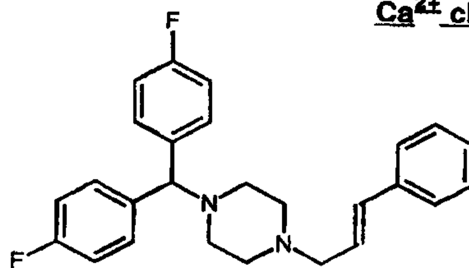
Flunarizine (74)
