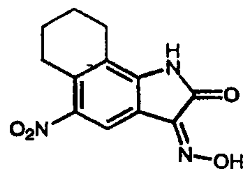
NS-102 (29)
