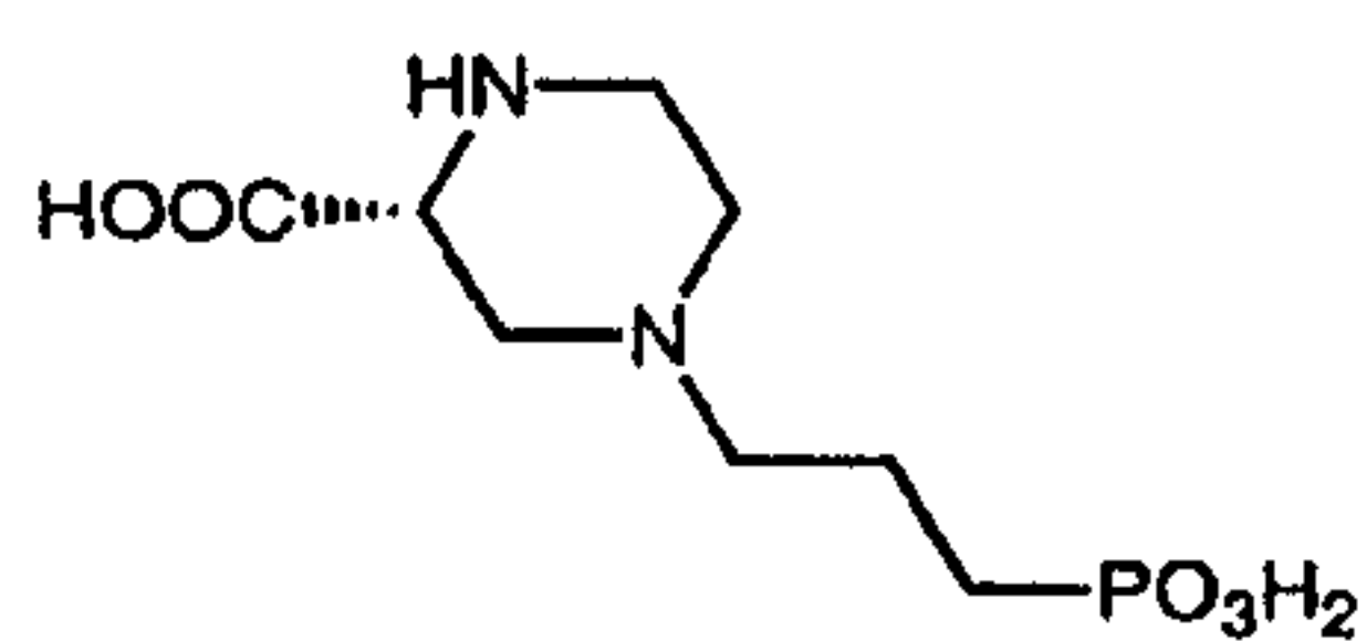
(R)-CPP (2)
