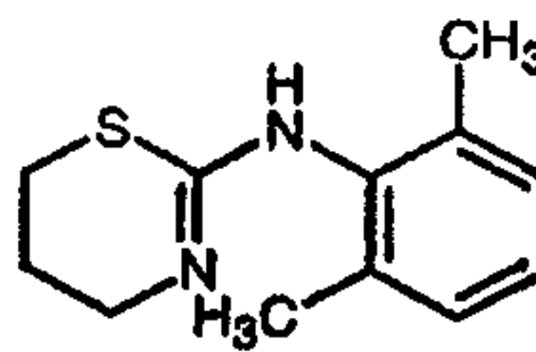
Xylazine (63)
