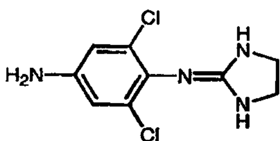
Apraclonidine (62)
