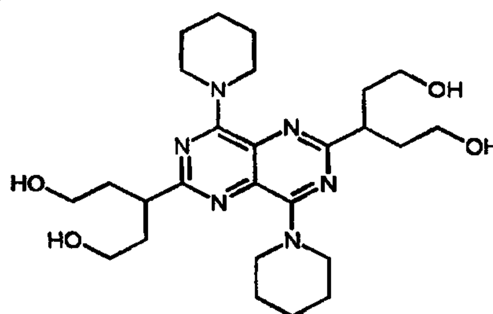
Dipyridamole (56b)
