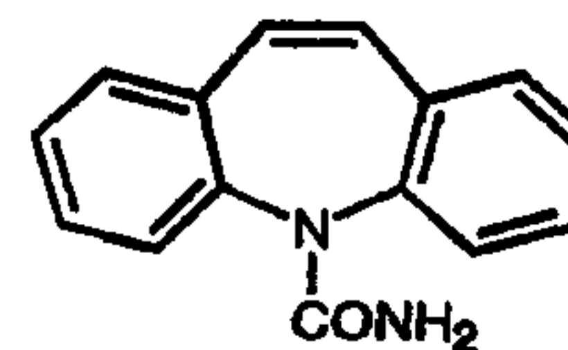
Carbamazepine (70)
