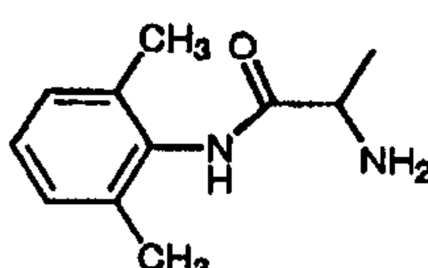
Tocainide (72)
