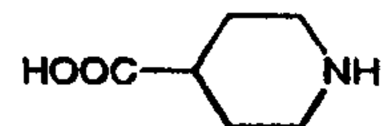
Isonipecotic acid (47)
