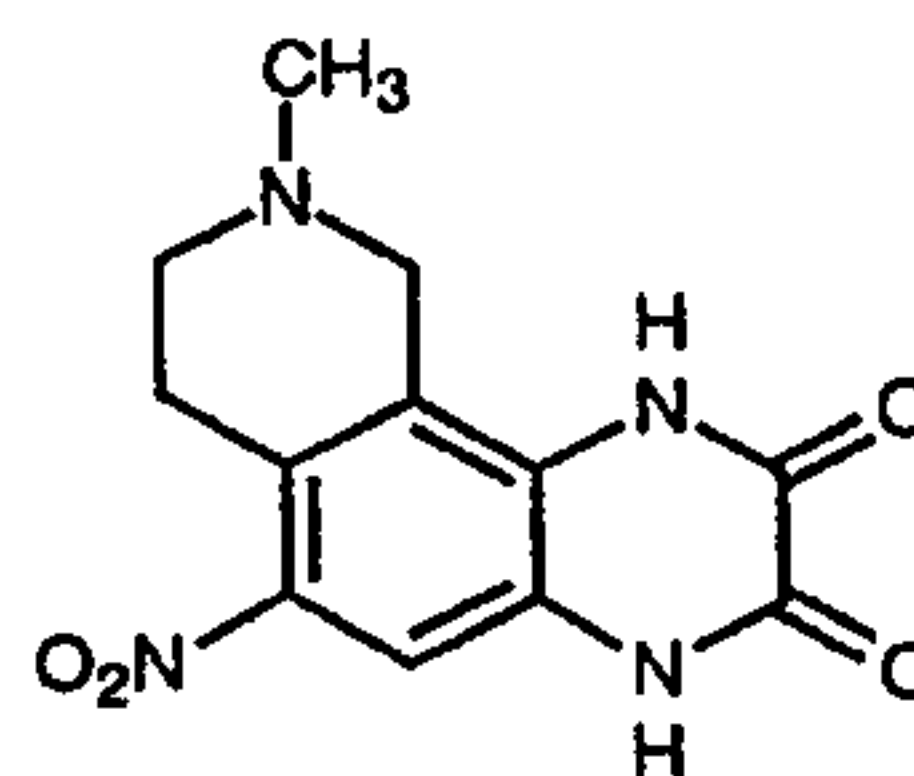
PNQX (21)
