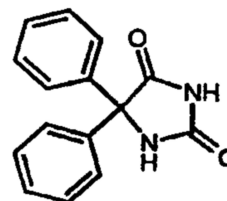
Phenytoin (67)
