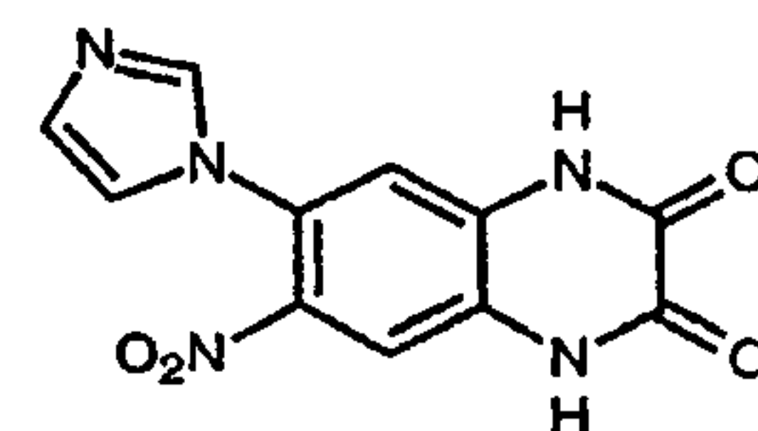
YM90K (22)
