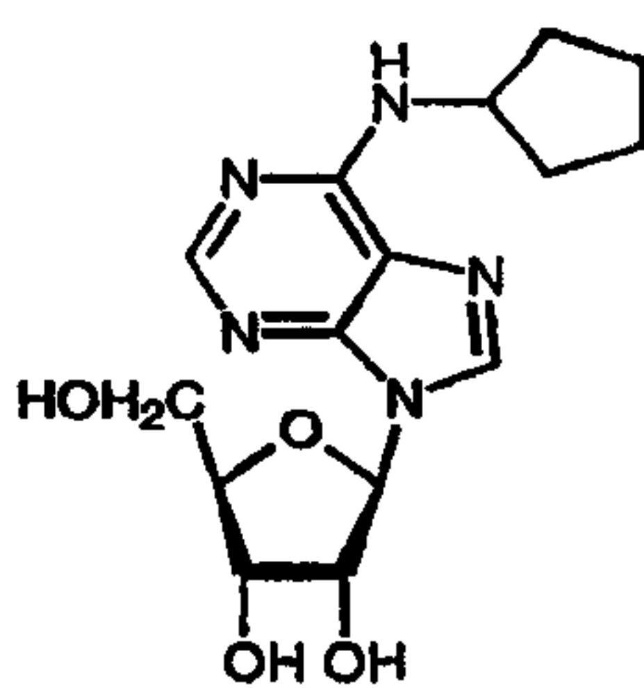
N 6 -Cyclopentyladenosine (56)
