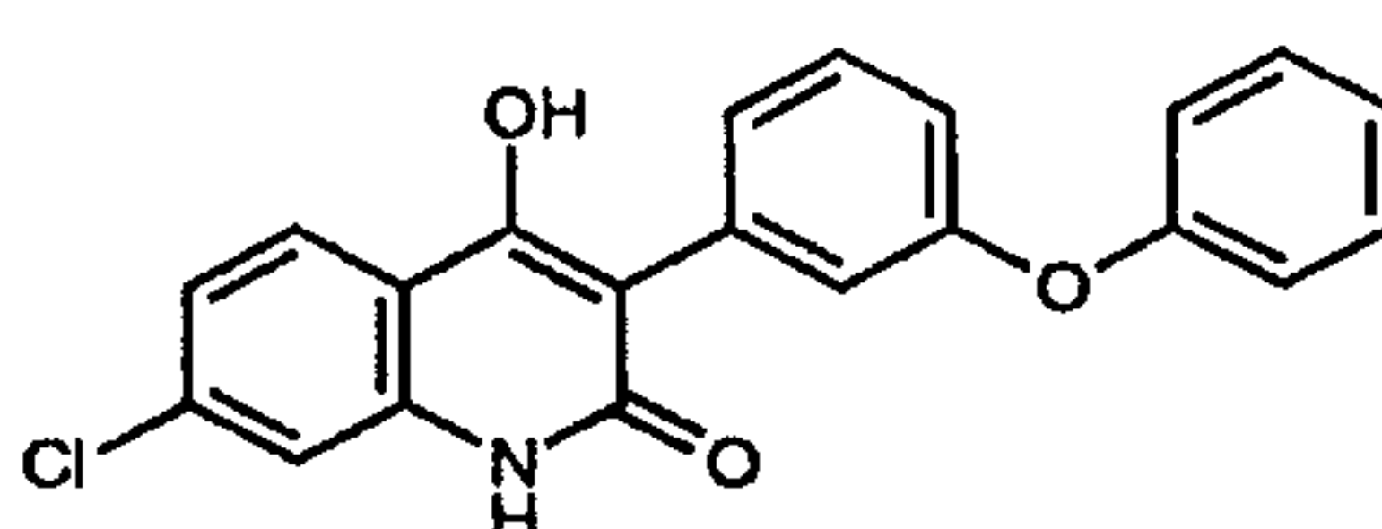
L-701,324 (14c)
