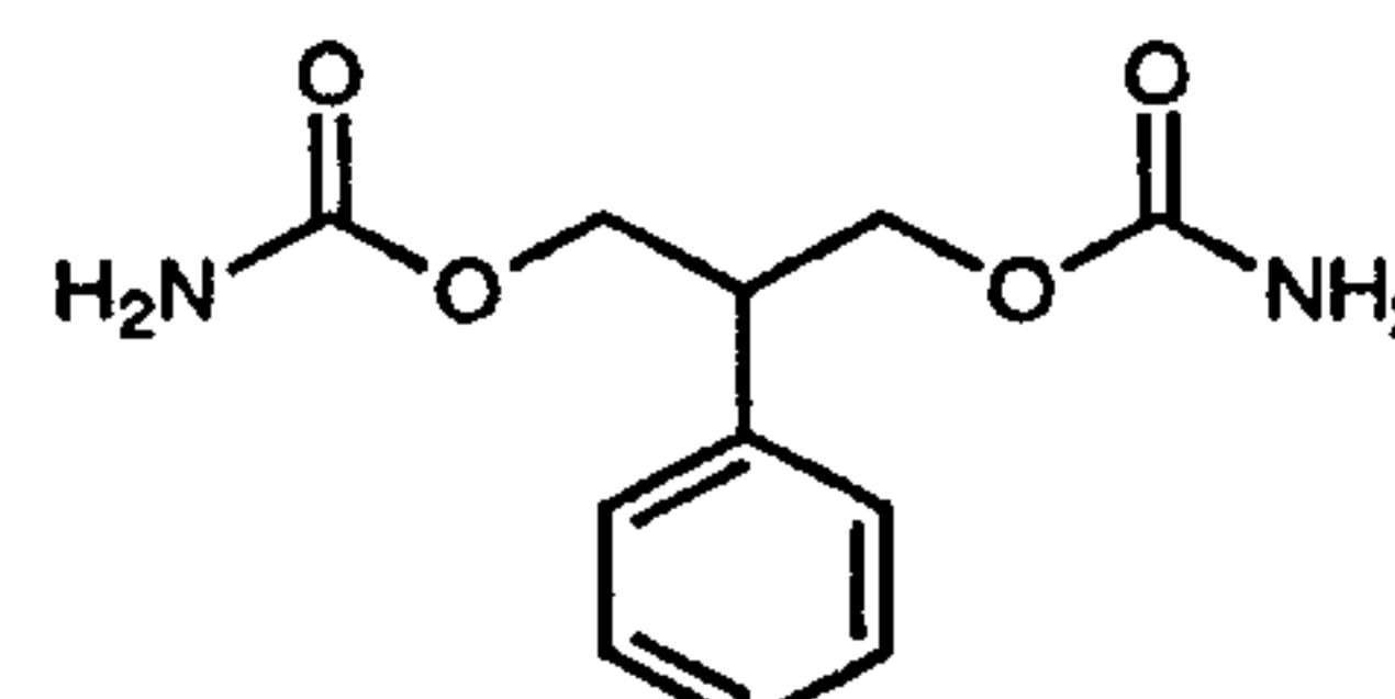
Felbamate (18)
