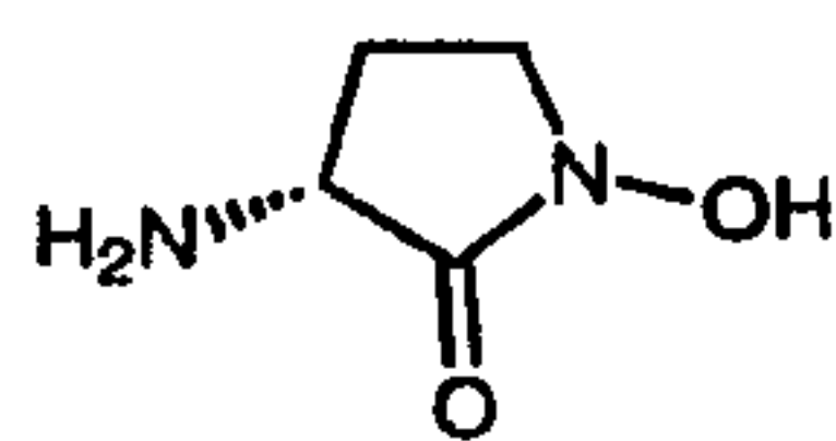
(R)-HA-966 (12)
