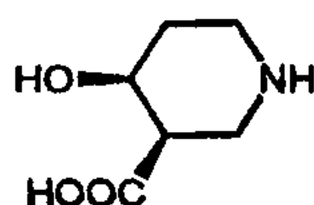
(±)-cis-4-Hydroxynipecotic acid (50)
