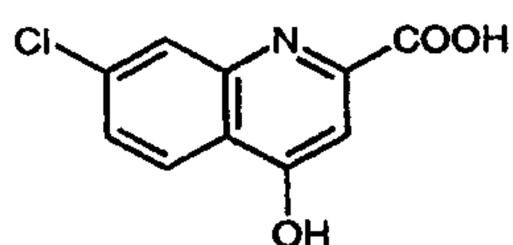
7-Cl-Kynurenic acid (13)
