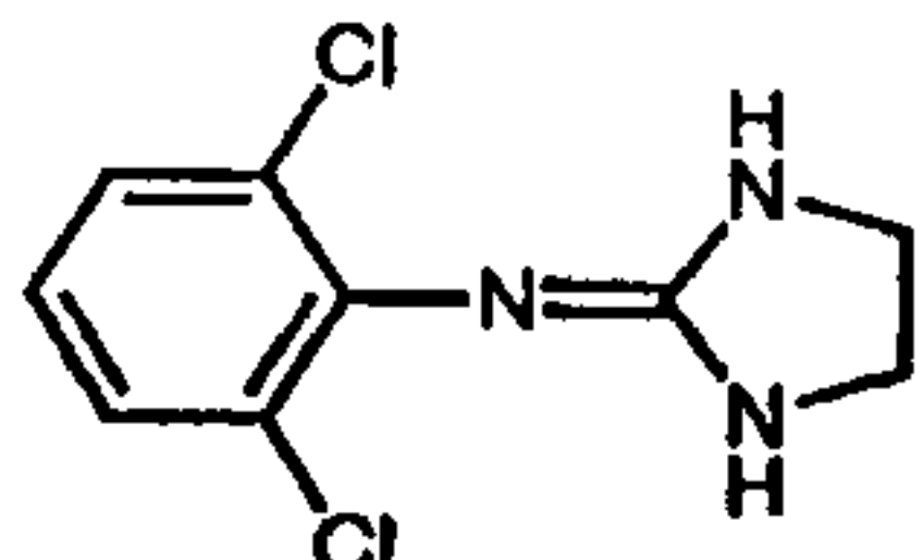
Clonidine (61)
