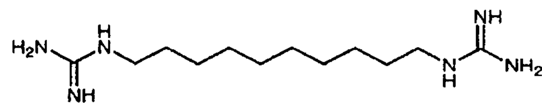
Synthalin (11a)
