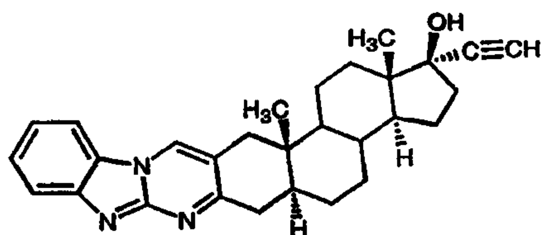
WIN 51,708 (33)
