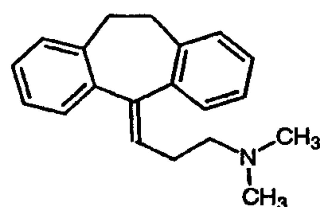
Amitriptyline (4b)
