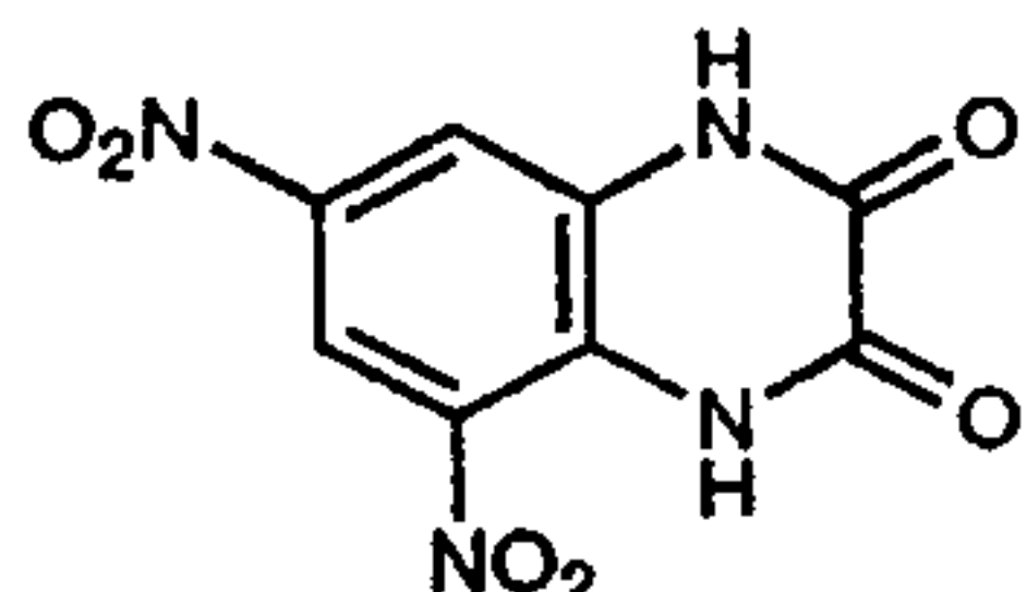
MNQX (16)
