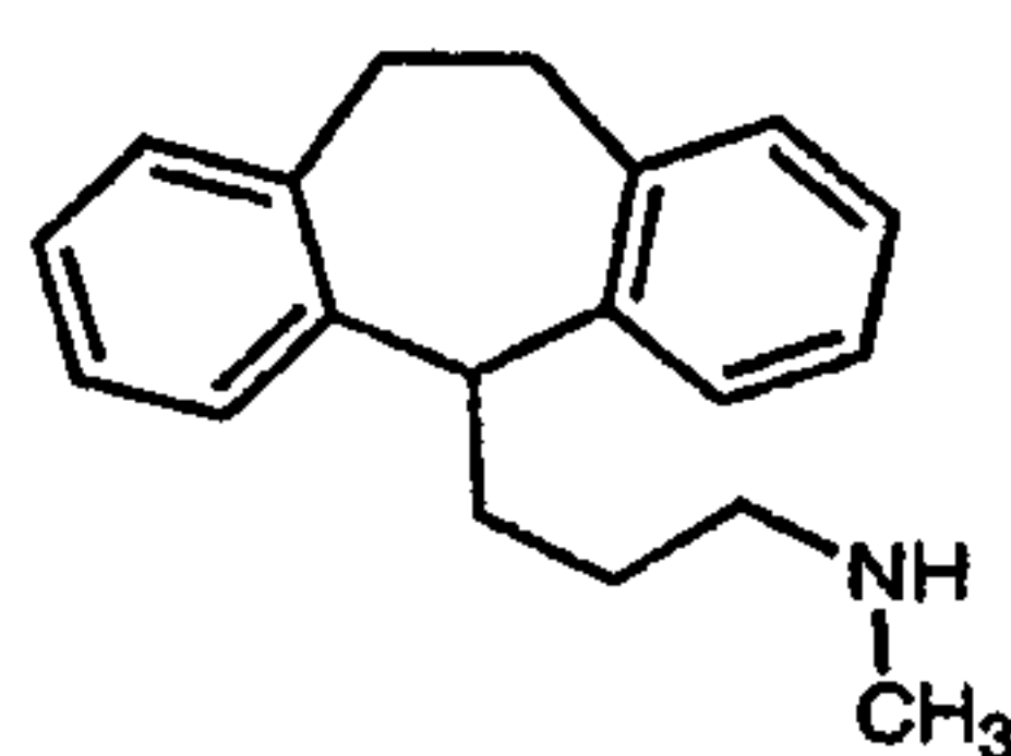
Desipramine (4d)
