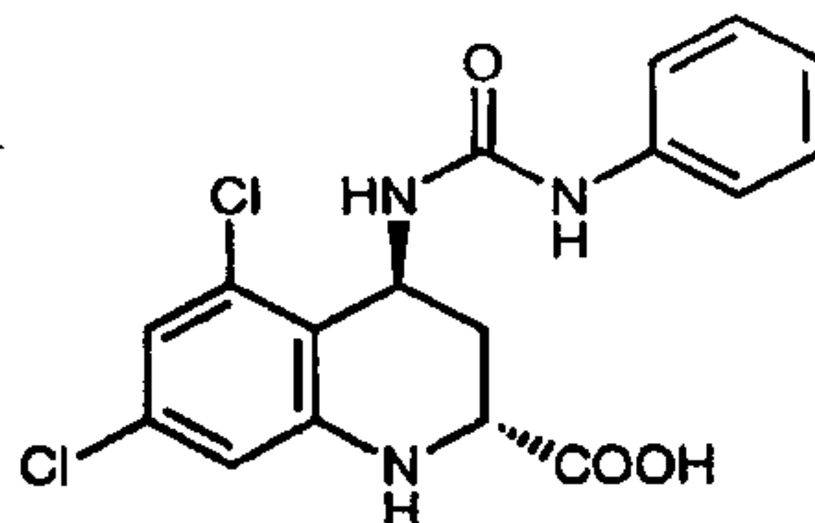
L-689,560 (14)
