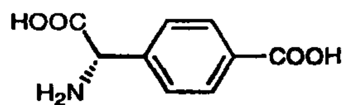
4CPG (30)
