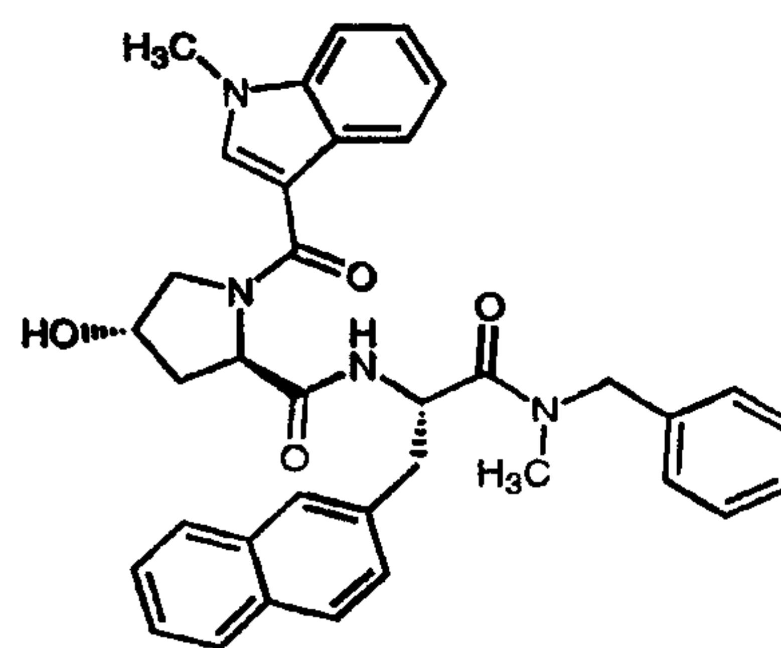
FK 888 (36)
