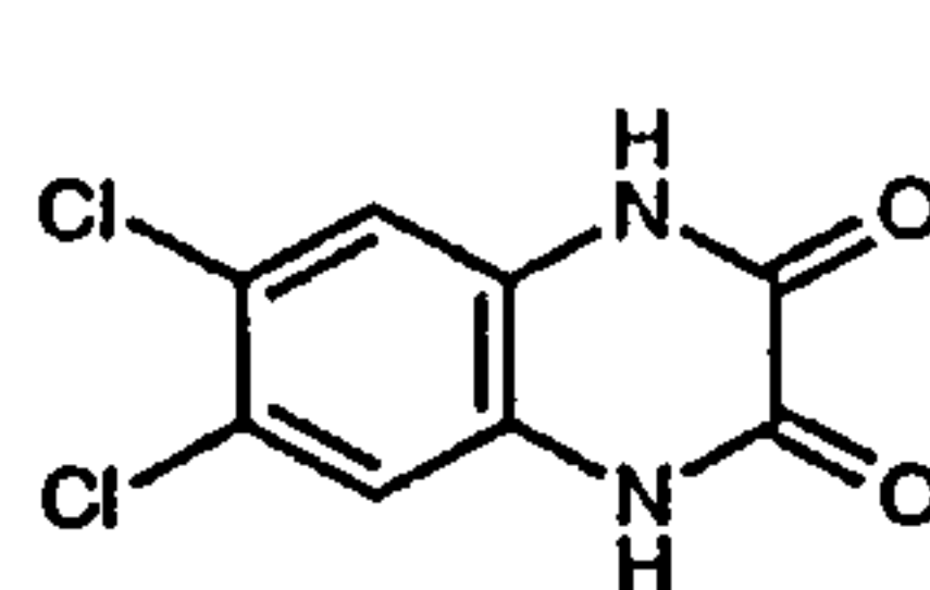
DCQX (17a)
