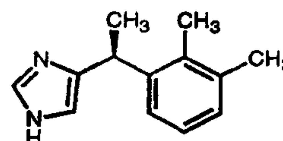
Dexmedetomidine (64)
