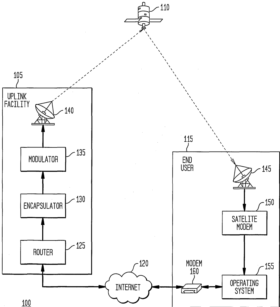
FIG. 1 (PRIOR ART)
