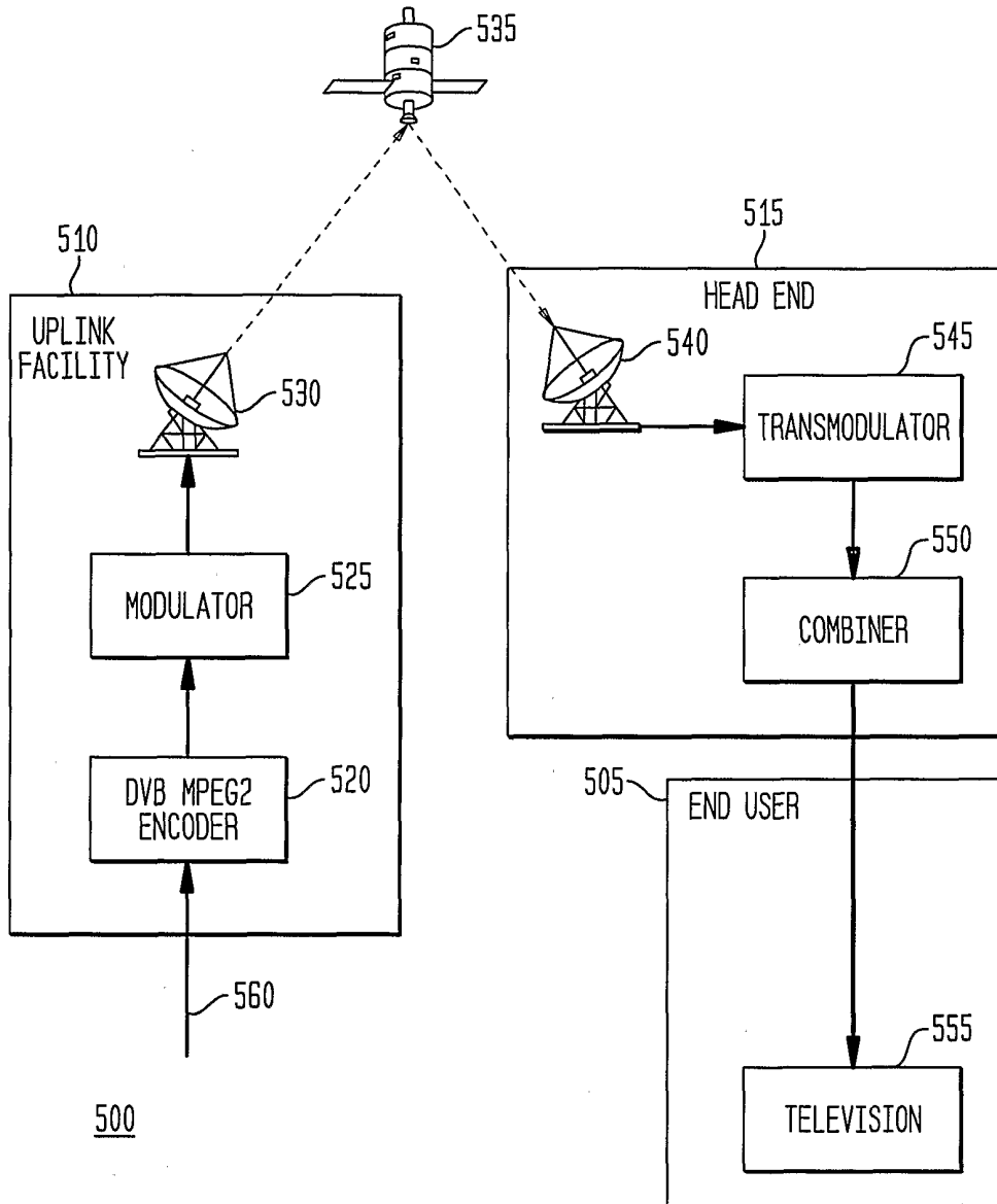
FIG. 5 (PRIOR ART)
