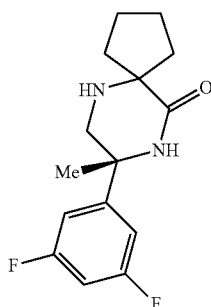
(8R)-8-(3,5-Difluorophenyl)-8-methyl-6,9-diazaspiro[4.5]decan-10-one
