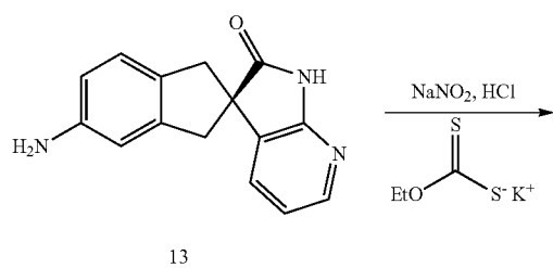
SCHEME 6
