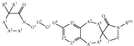
Ib
