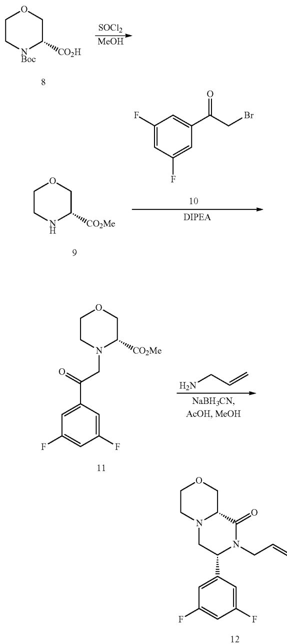
SCHEME 4
