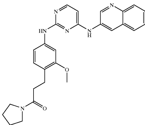
3-{2-Methoxy-4-[4-(quinolin-3-ylamino)-pyrimidin-2-ylamino]-phenyl}-1-pyrrolidin-1-yl-propanone
