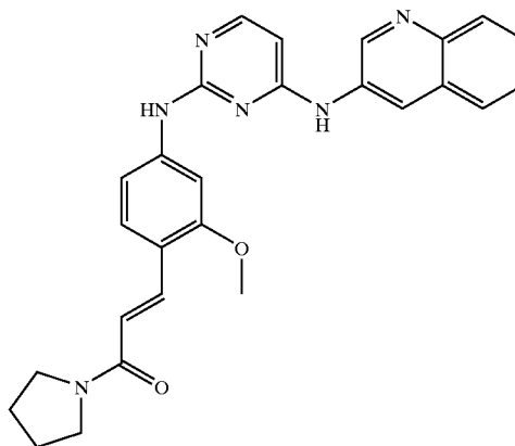
3-{2-Methoxy-4-[4-(quinolin-3-ylamino)-pyrimidin-2-ylamino]-phenyl}-1-pyrrolidin-1-yl-propenone
