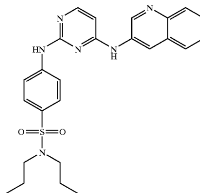
N,N -Dipropyl-4-((4-(3-quinolinylamino)-2-pyrimidinyl)amino)benzenesulfonamide
