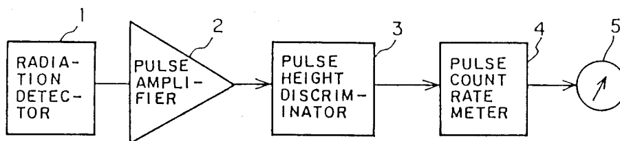
FIG. 1 (PRIOR ART)
