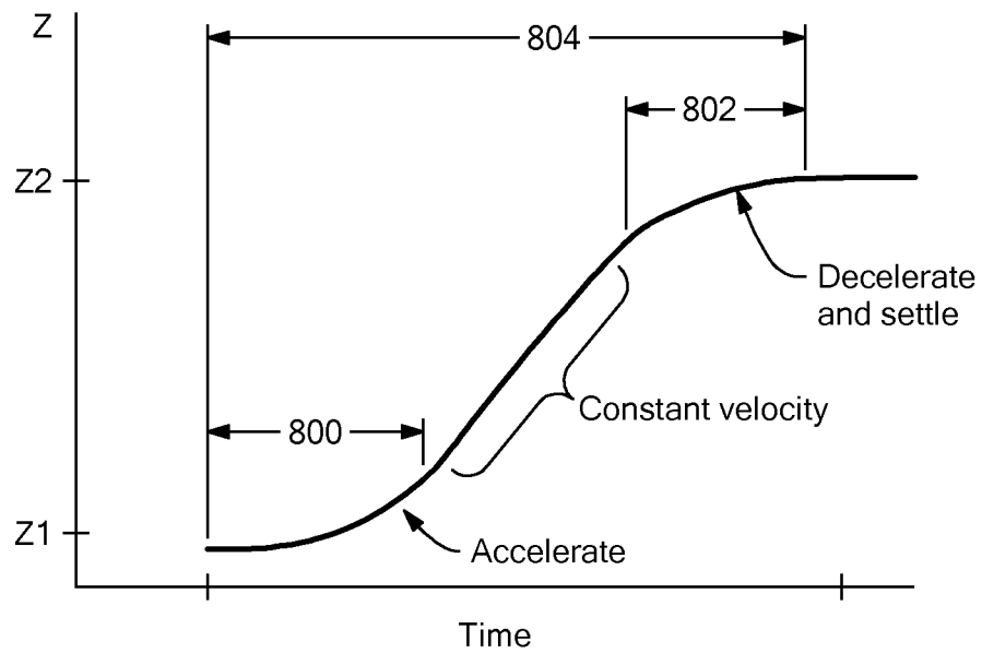
FIG. 8 PRIOR ART
