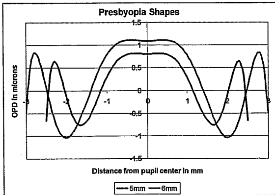
Fig. 42 Examples of Presbyopia Shapes for a 5mm and a 6mm pupil.
