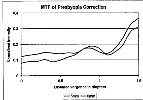
Fig. 43 Examples of Modulation Transfer Function (MTF) for a 5mm and a 6mm pupil.
