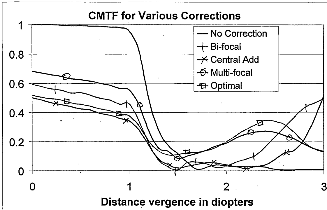
Compound MTF (CMTF) with different corrections.
