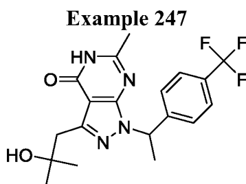
3-(2-Hydroxy-2-methylpropyl)-6-methyl-1-(1-(4-(trifluoromethyl)phenyl)ethyl)-1H-pyrazolo[3,4-d]pyrimidin-4(5H)-one (Scheme 31)
