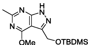
3-(((tert-Butyldimethylsilyl)oxy)methyl)-4-methoxy-6-methyl-1H-pyrazolo[3,4-d]pyrimidine (Scheme 16)
