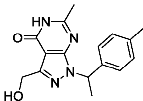
3-(Hydroxymethyl)-6-methyl-1-(1-p-tolylethyl)-1H-pyrazolo[3,4-d]pyrimidin-4(5H)-one (Scheme 17)
