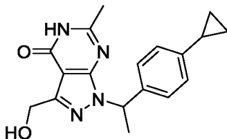
1-(1-(4-Cyclopropylphenyl)ethyl)-3-(hydroxymethyl)-6-methyl-1H-pyrazolo[3,4-d]pyrimidin-4(5H)-one (Scheme 17)
