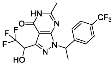
6-Methyl-3-(2,2,2-trifluoro-1-hydroxyethyl)-1-{1-[4-(trifluoromethyl)phenyl]ethyl}-1,5-dihydro-4H-pyrazolo[3,4-d]pyrimidin-4-one (Scheme 55)
