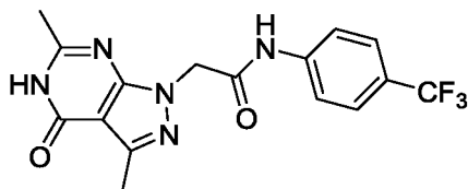
2-(3,6-Dimethyl-4-oxo-4,5-dihydropyrazolo[3,4-d]pyrimidin-1-yl)-N-(4-(trifluoromethyl)phenyl)acetamide (Scheme 63)
