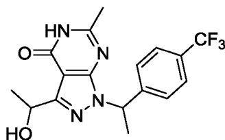
3-(1-Hydroxyethyl)-6-methyl-1-{1-[4-(trifluoromethyl)phenyl]ethyl}-1,5-dihydro-4H-pyrazolo[3,4-d]pyrimidin-4-one (Scheme 35).
