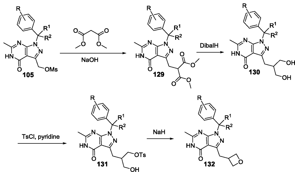
Scheme 47.
