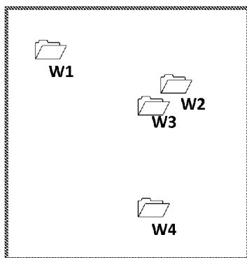
Figure 11. Initial locations of wells(W1-W4)
