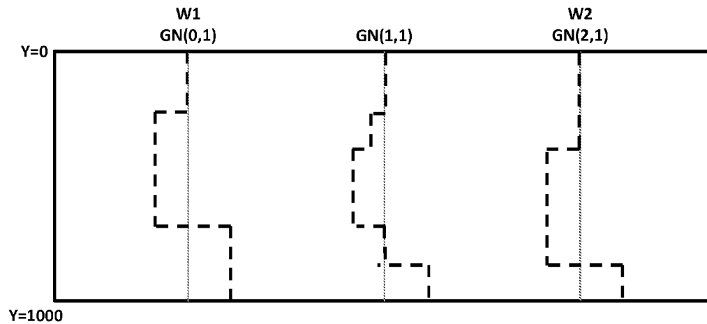
Figure 18. Generated well log for node GN(1,1) if stratigraphic correlations A and B are not used.
