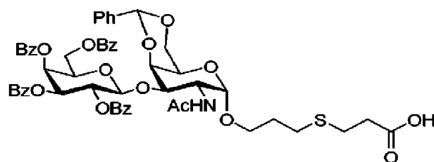
Compound 10
