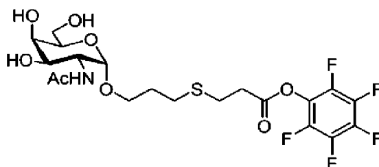
Compound 9
