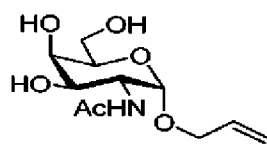
Allyl Tn
