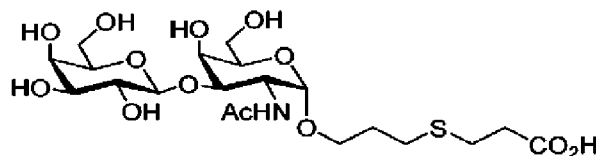
Compound 12
