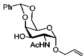
Compound 4
