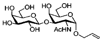
Allyl TF
