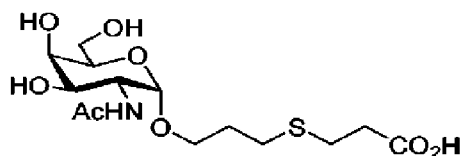
Compound 8
