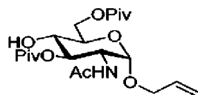
Compound 2
