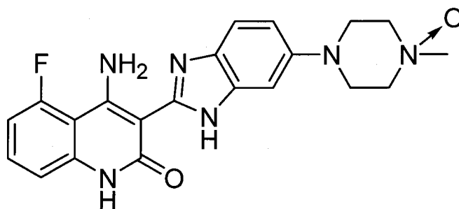
Compound 2
