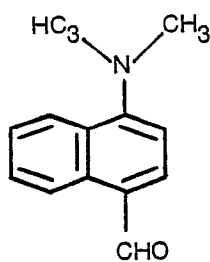
1-dimethylamino-4-formyl naphthalene
