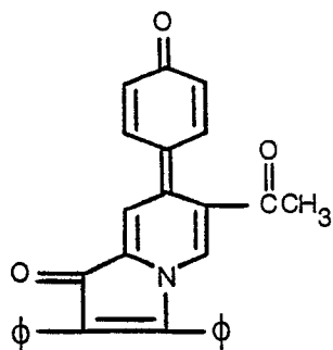
6-acetyl-2,3-diphenyl-7-(4-oxo-phenylidene)- 1(7H)-indolizinone
