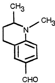
1,2-dimethyl-6-formyl-1,2,3-tetrahydroquinoline
