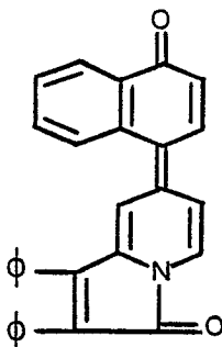
1,2-diphenyl-7-(4-oxo-1-naphthylidene)- 3-(7H)-indolizinone
