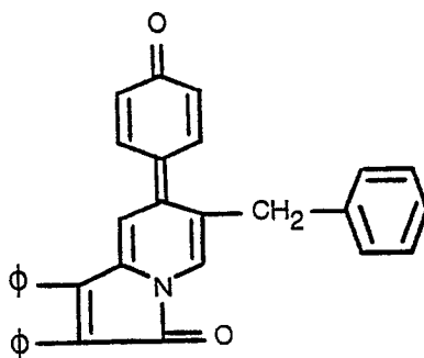
6-chloro-1,2-diphenyl-7-(4-oxo-1-phenylidene)- 3(7H)-indolizinone
