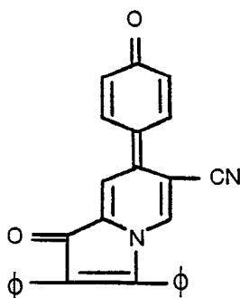
6-cyano-2,3-diphenyl-7-(4-oxo-1-phenylidene)- 1(7H)-indolizinone
