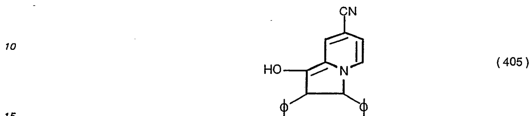
5 7-cyano-2,3-diphenyl-1-indolizinol
