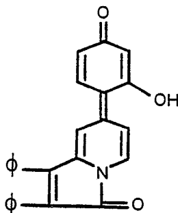
1,2-diphenyl-7-(4-oxo-2-hydroxy-1-phenylidene)- 3-(7H)-indolizinone
