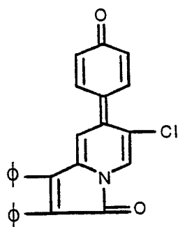
6-chloro-1,2-diphenyl-7-(4-oxo-1-phenylidene)- 3(7H)-indolizinone
