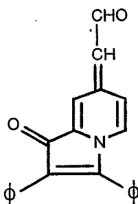
7-formylmethylidene-2,3-diphenyl-1(7H)-indolizinone
