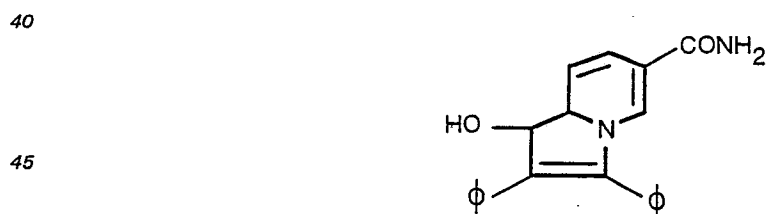
40 6-aminocarbonyl-2,3-diphenyl-1-indolizinol
