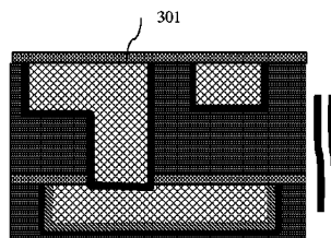
An Interconnect Containing 2 Different Cap Materials
