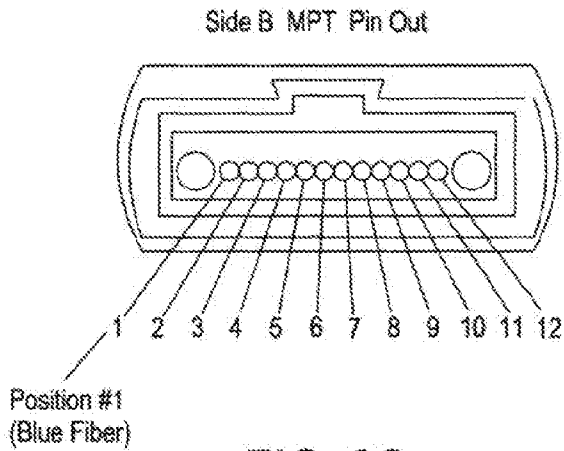
FIG. 2C PRIOR ART METHOD B POLARITY
