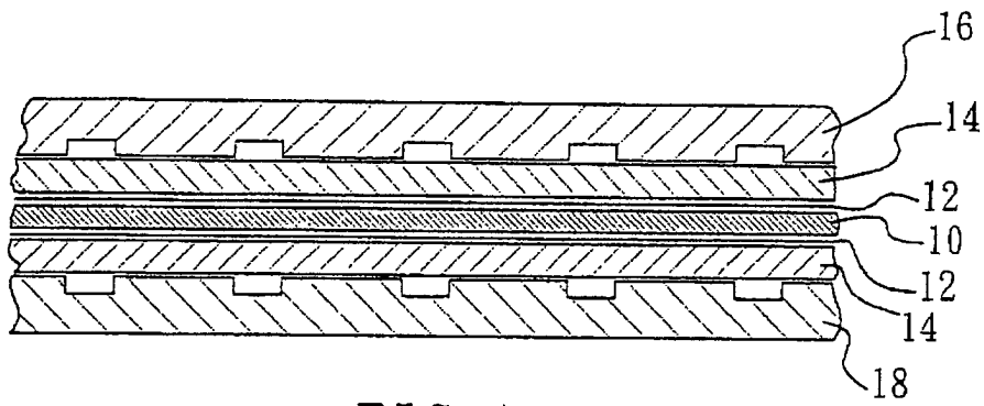
FIG. 1 (PRIOR ART)
