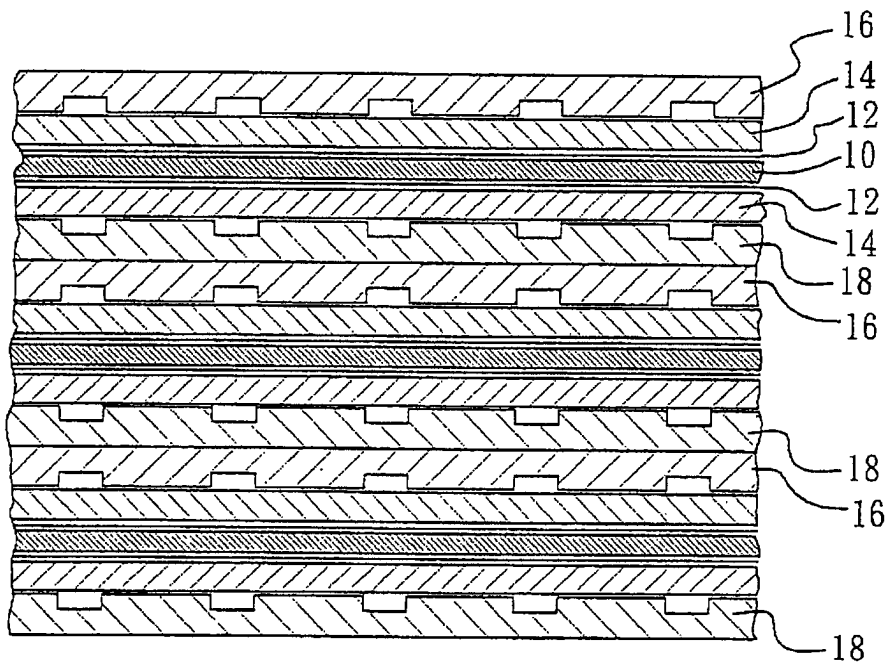
FIG. 2 (PRIOR ART)
