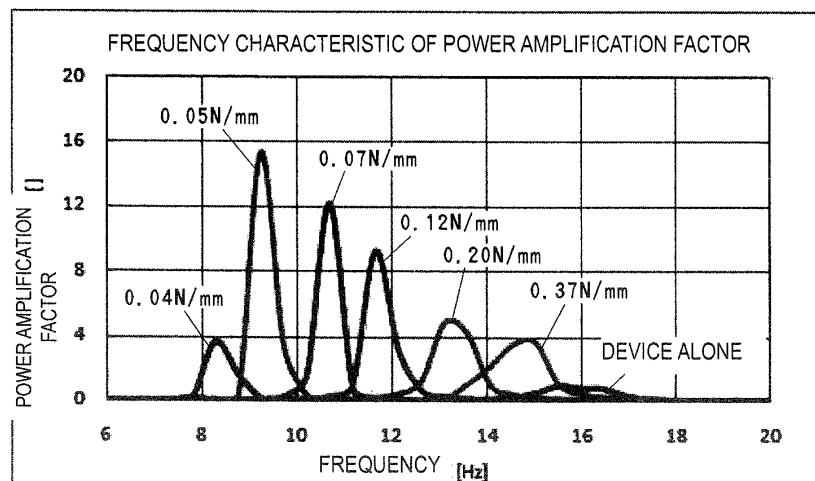
(b) FREQUENCY CHARACTERISTIC OF POWER AMPLIFICATION FACTOR
