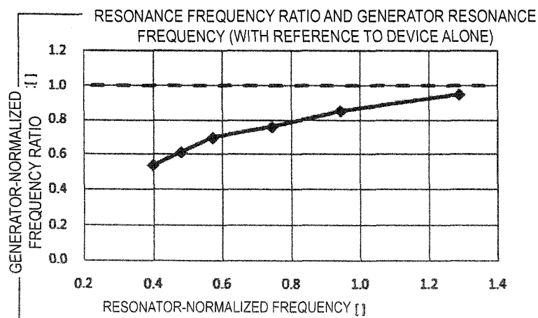
(c) GENERATOR-NORMALIZED FREQUENCY
