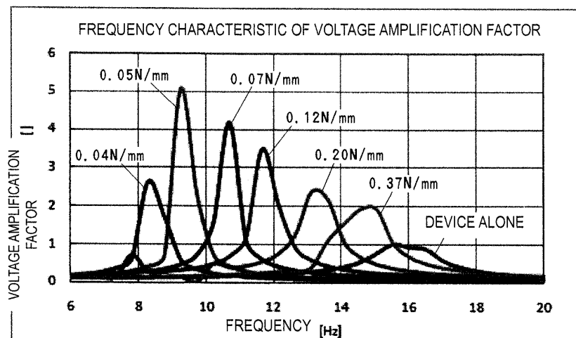
(a) FREQUENCY CHARACTERISTIC OF VOLTAGE AMPLIFICATION FACTOR
