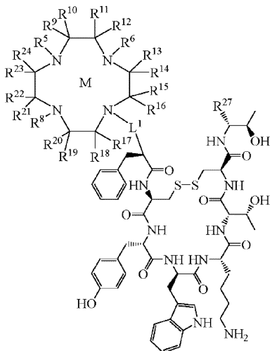
Formel (VII),
