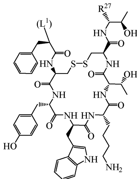
Formula (VI),
