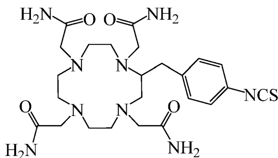
"TCMC" (AKA "TCMC-Bz-NCS"),
