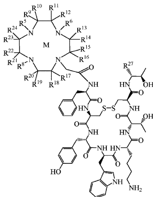
Formel (IX),
