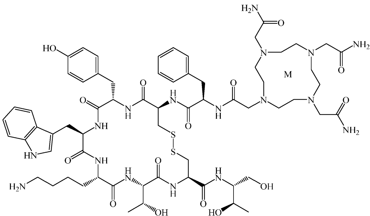
“DOTAMTOC”
