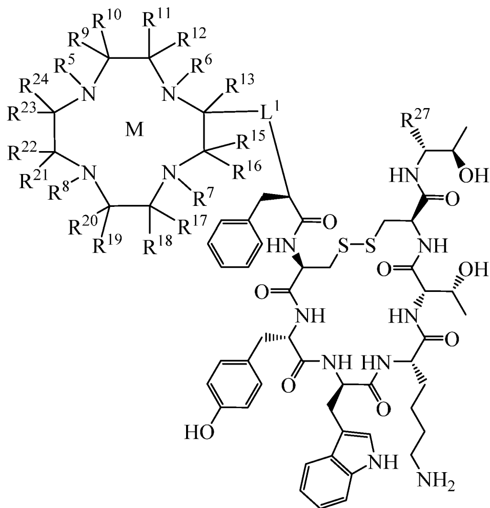
Formula (VIII),
