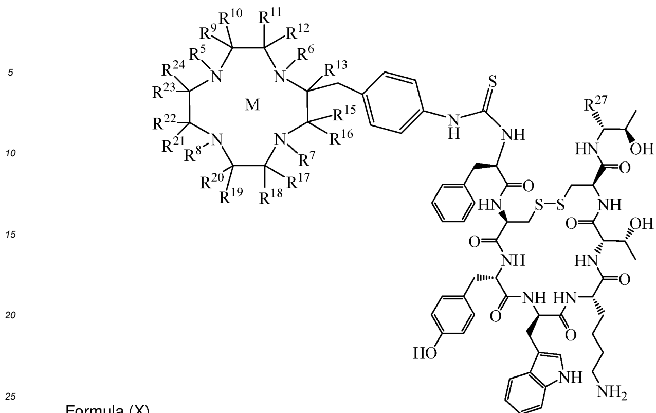
Formula (X)
