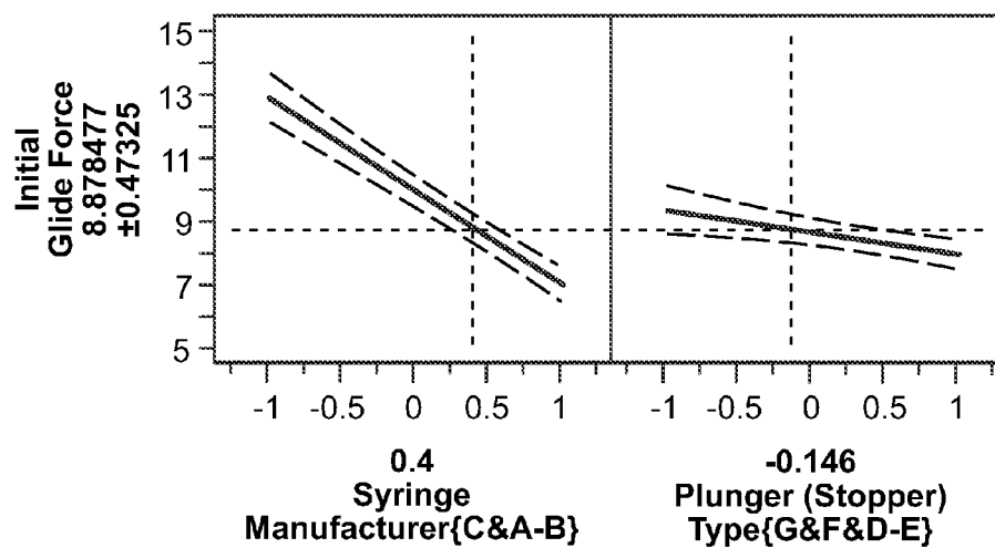
Prediction Profiler: Initial Glide Force
