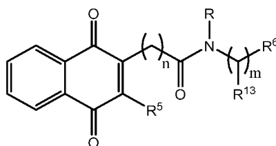
Formula (Ib)
