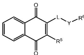
Formula (Ia)
