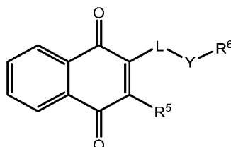
Formula (Ia)
