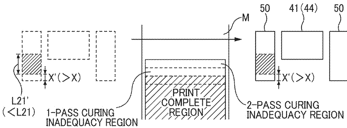
FIG. 16B (FIRST TERMINAL PASS)
