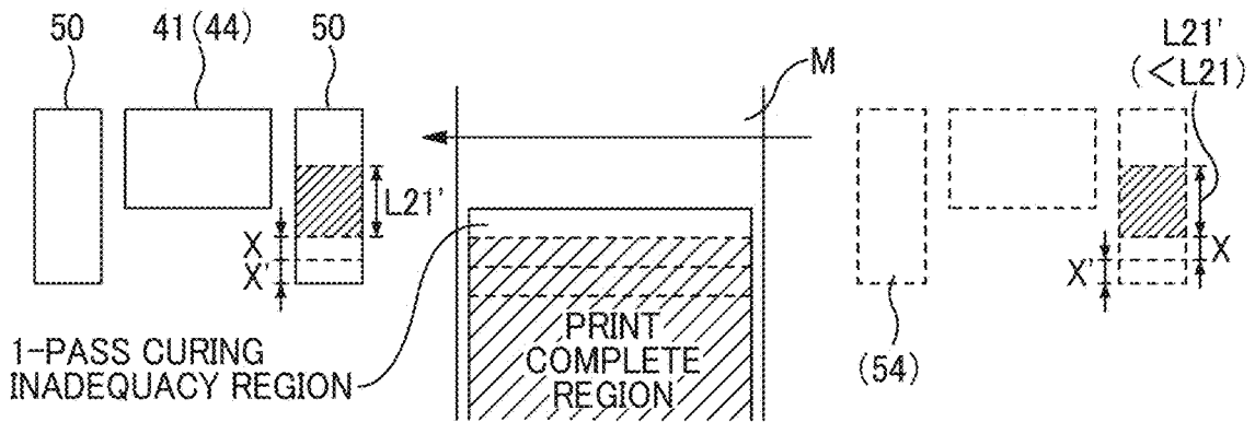
FIG. 16C (SECOND TERMINAL PASS)
