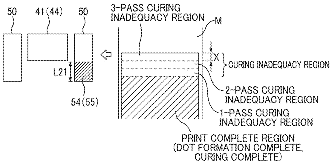
FIG. 16A (PASS FOR LAST DOT FORMATION)
