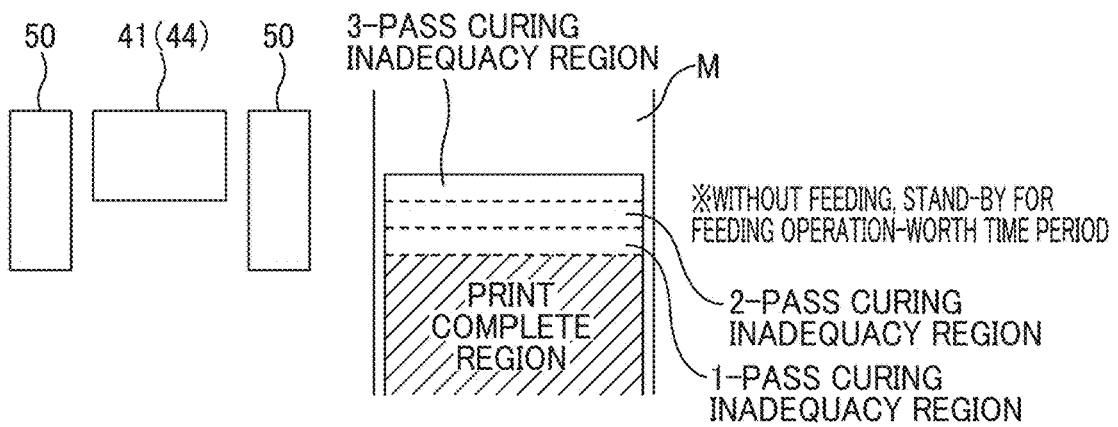
FIG. 15B (THIS PREFERRED EMBODIMENT)
