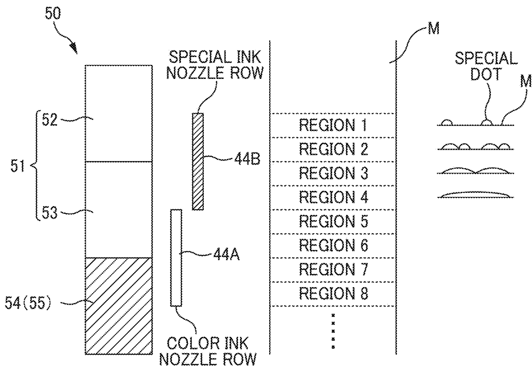
FIG. 20B (SPECIAL PRINTING MODE)
