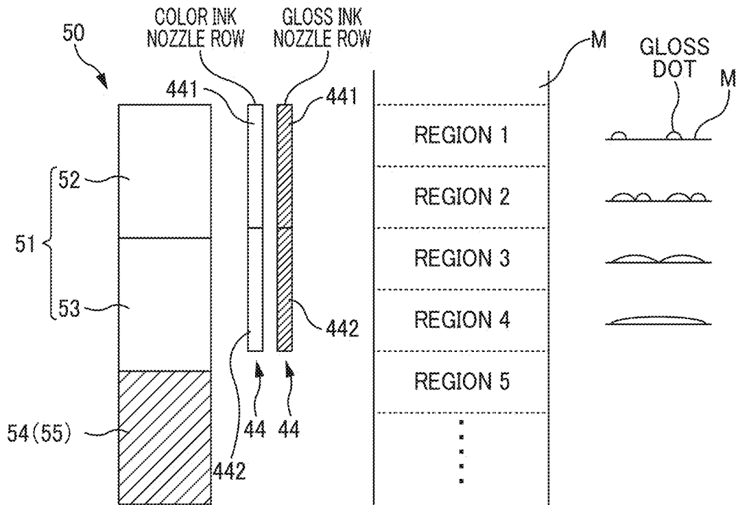
FIG. 10B (GLOSS PRINTING MODE)
