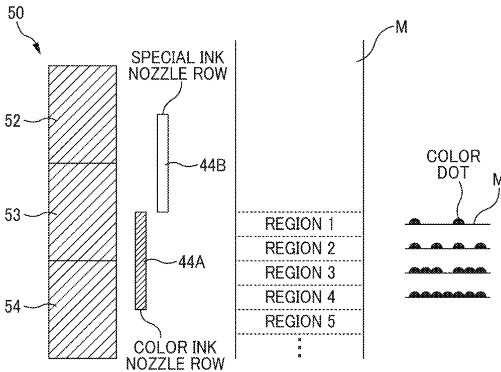
FIG. 20A (COLOR PRINTING MODE)
