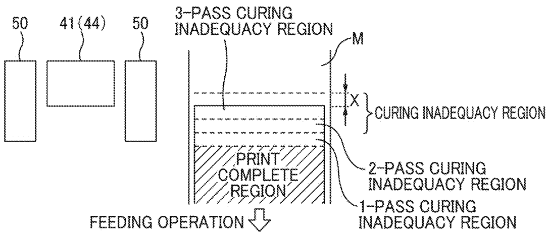
FIG. 14B (REFERENCE EXAMPLE)
