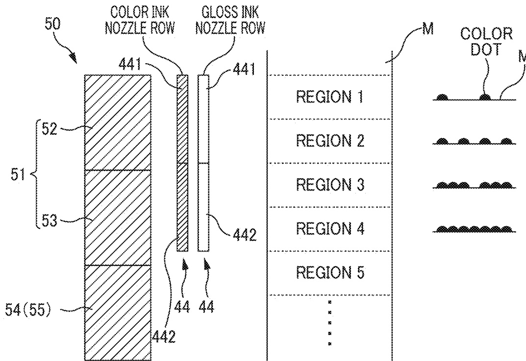
FIG. 10A (COLOR PRINTING MODE)
