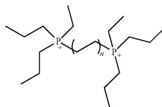
Phosphonium
