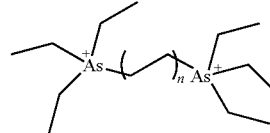
Arsonium
