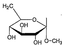
Ranimustine
