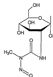
Streptozocin
