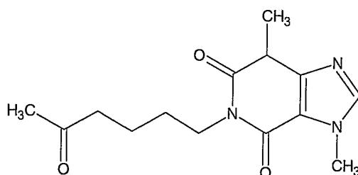
Pentoxifylline
