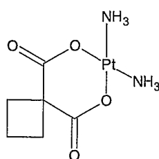
Carboplatin
