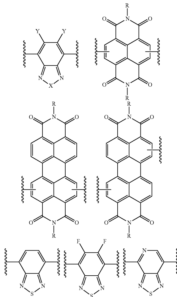
(XIIIa)
