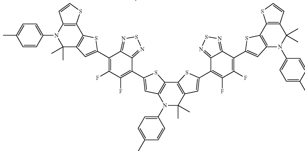
Model Compound 2
