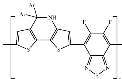
Polymer Example 1
