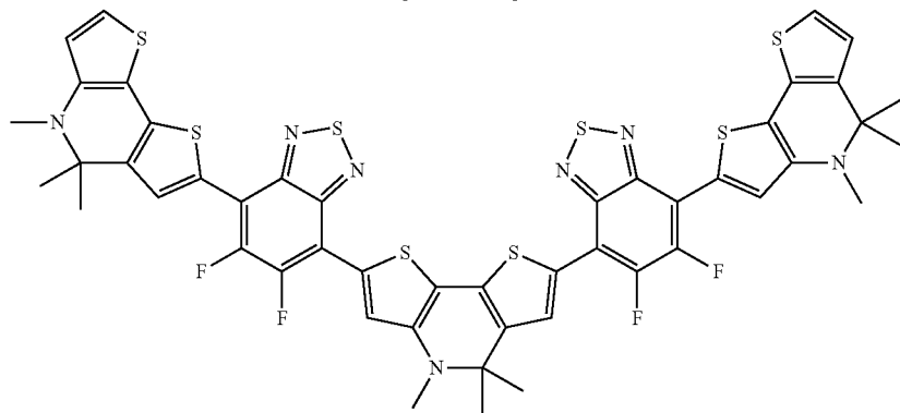
Model Compound 1
