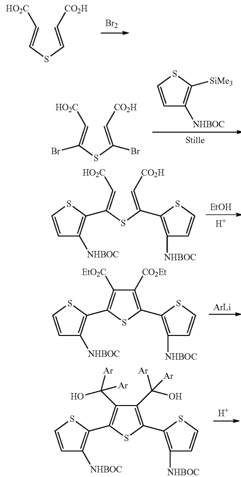
Scheme 3
