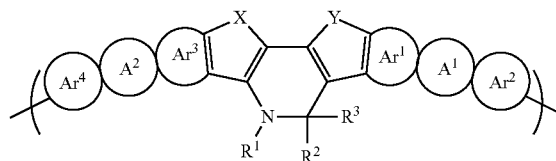
formula (Id)
