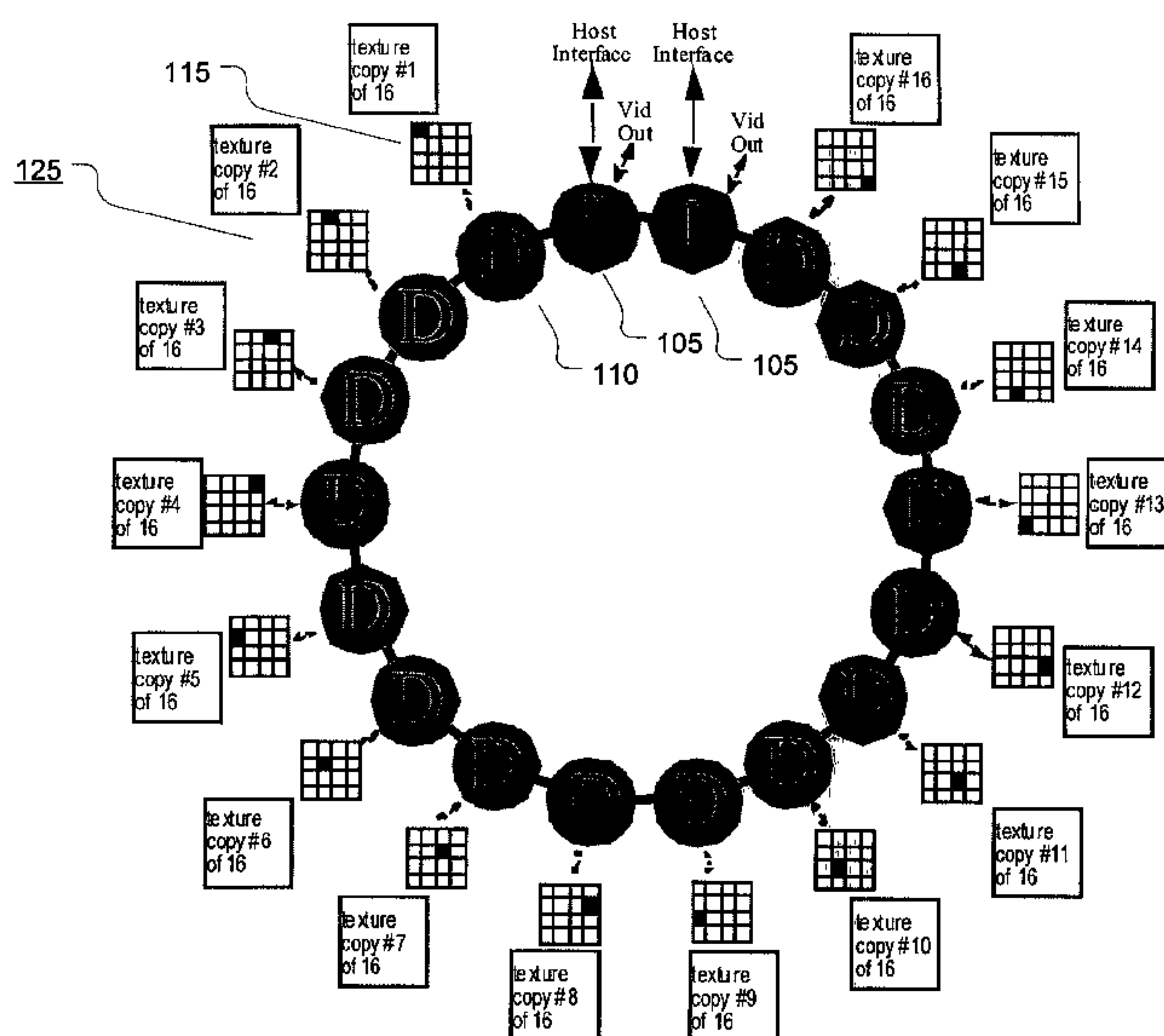
Texture and Frame Buffer Memory Allocation and Partitioning
