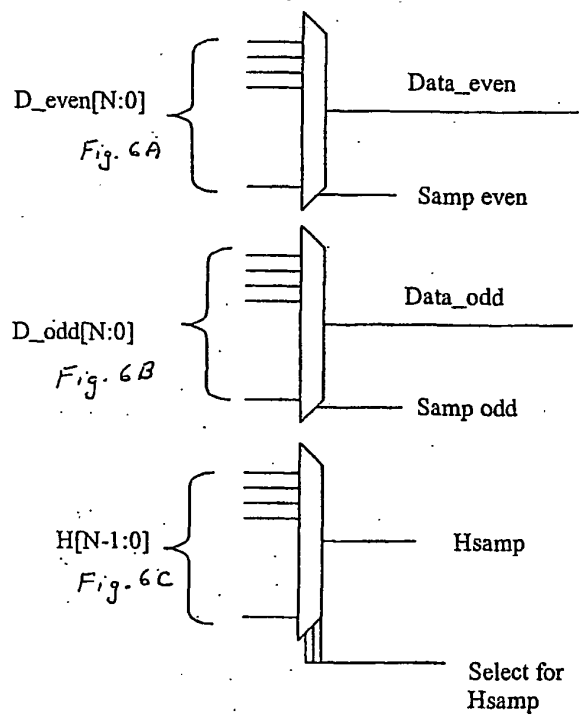
Figure 6 Data and History Sample Muxes
