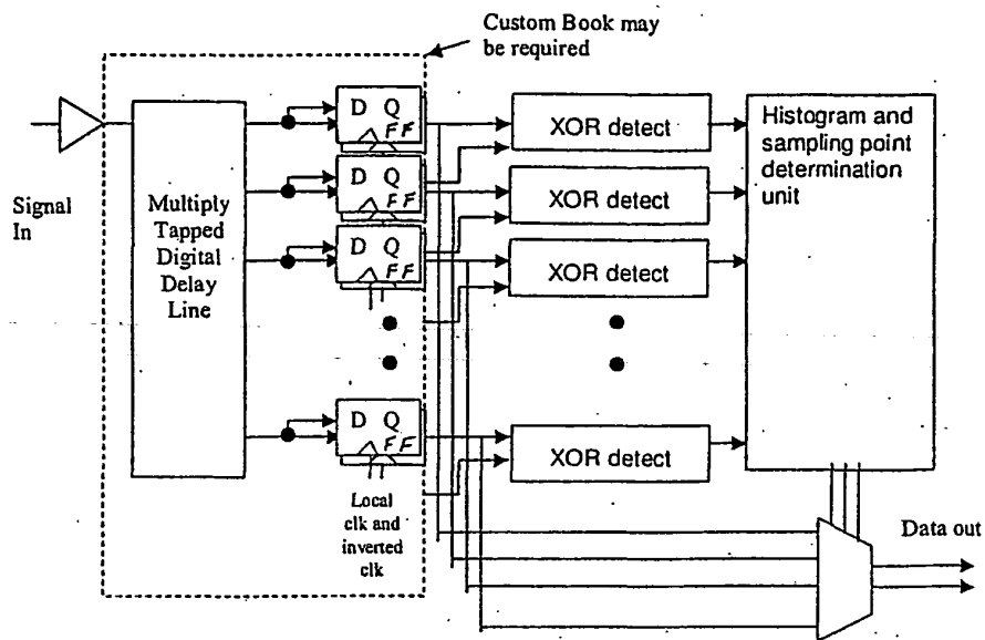
Figure 3 Instage, 2-bit Macro Block
