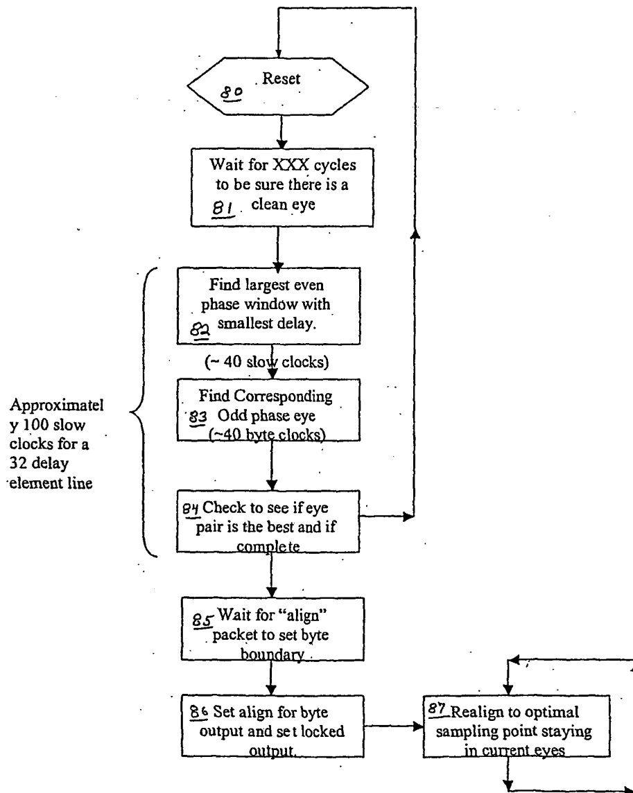
Figure 8 Eye Detection Flow Diagram
