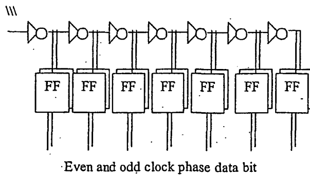
Figure 4 Clocked Delay Line
