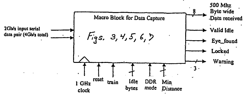
Figure 1 Data Receive Macro Block
