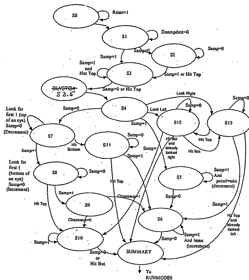
Figure 9 Two Bit Macro State Diagram 1 of 2
