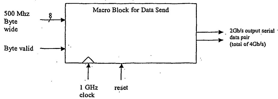
Figure 2 Data Send Macro Block
