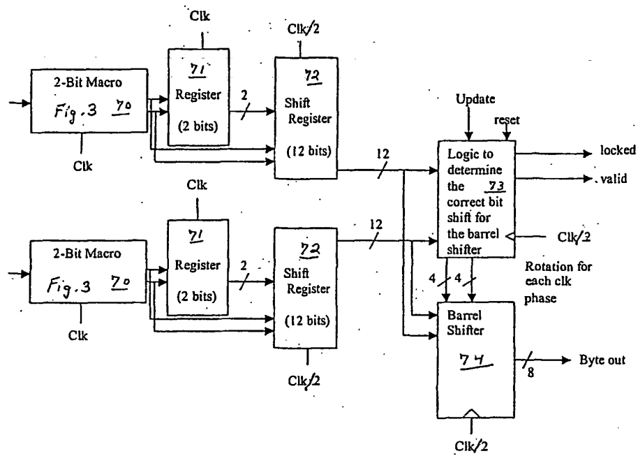
Figure 7 Serial Bit Combining and Byte Align Logic
