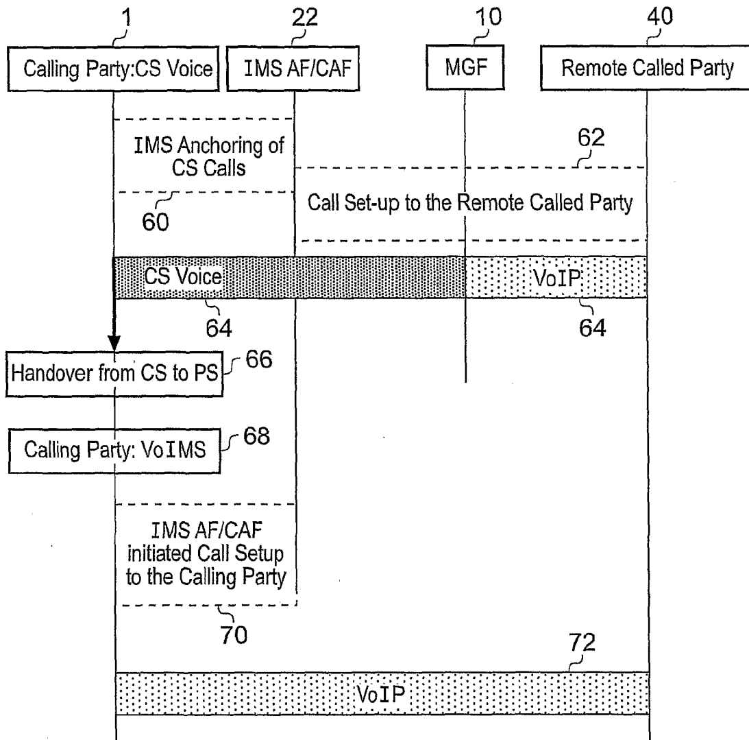
Handover procedures: CS domain to the PS Domain FIG. 5
