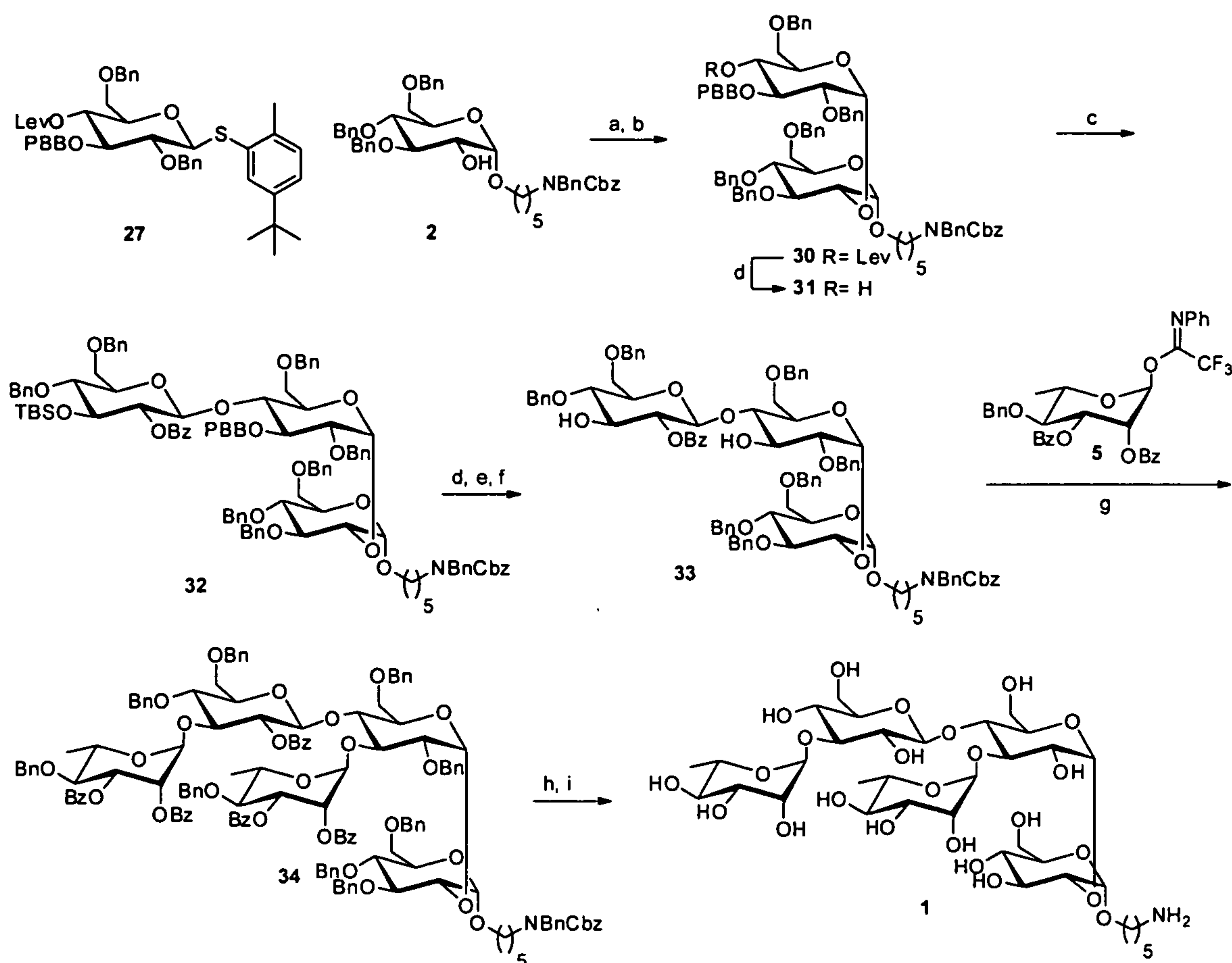
Scheme 8. Synthesis of pentasaccharide 1 (method B). Reagents and conditions: a) NIS/TfOH, Et 2 O, -20°C to 0°C, 69%; b) N 2 H 4 ·H 2 O, AcOH/Pyridine, DCM, 96%; c) 29 , NIS/TfOH, DCM, -30°C to -10°C, 92%; d) cat. Pd(OAc) 2 , (3,4-dimethoxyphenyl)boronic acid, TBABr, K 3 PO 4 , EtOH, 92%; e) DDQ, aq. NaHCO 3 , H 2 O, DCM; f) TBAF·3H 2 O, AcOH, DMF, 50°C, 68% over 2 steps; g) TMSOTf, DCM, 4Å MS, -30 °C to -15 °C, 88%; h) NaOMe, THF/MeOH, rt; i) H 2 , 10% Pd/C, MeOH, H 2 O, AcOH, 59% over 2 steps.
