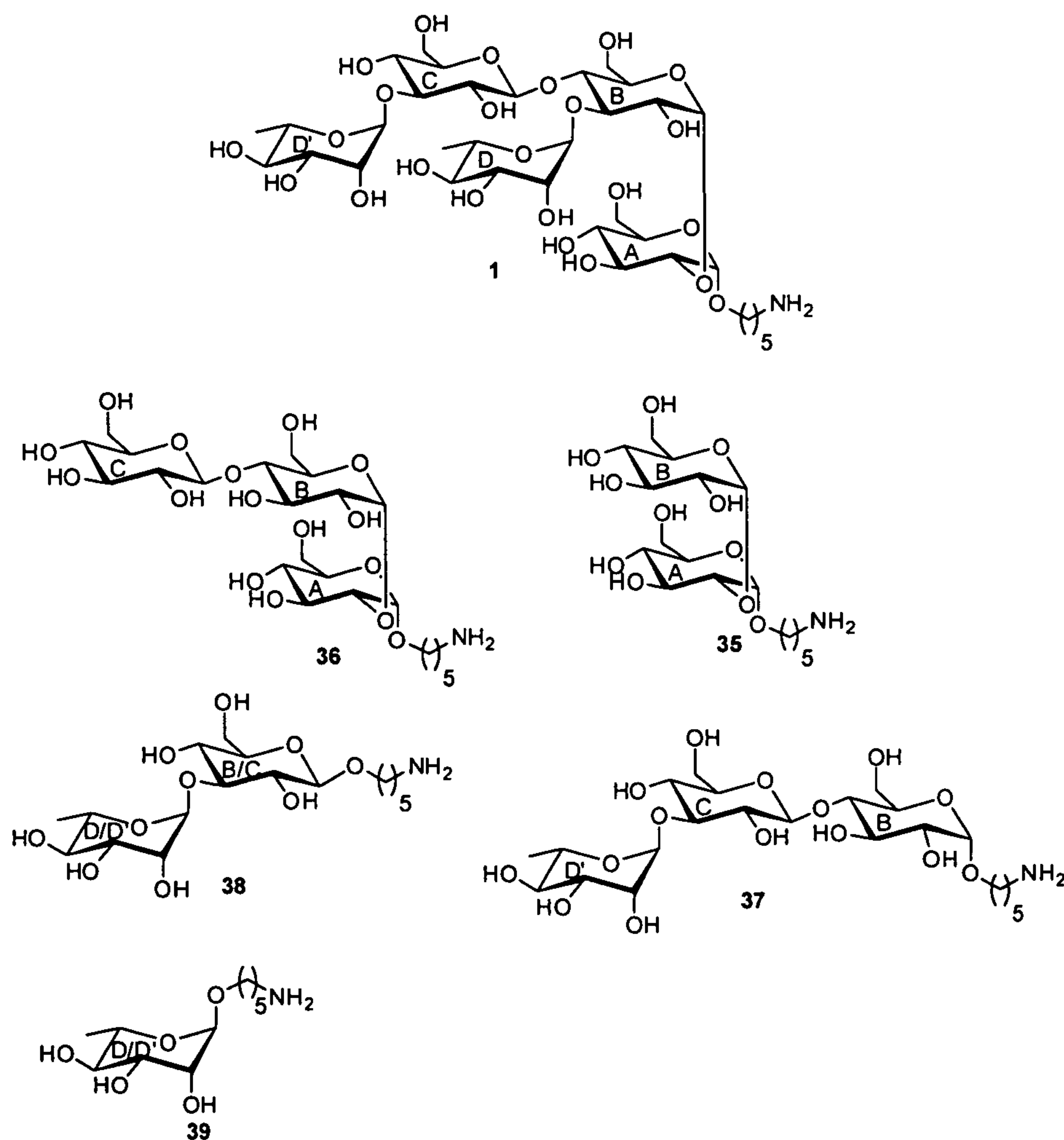
Scheme 9. Pentasaccharide 1 and comprehensive set of substructures 35–39 .
