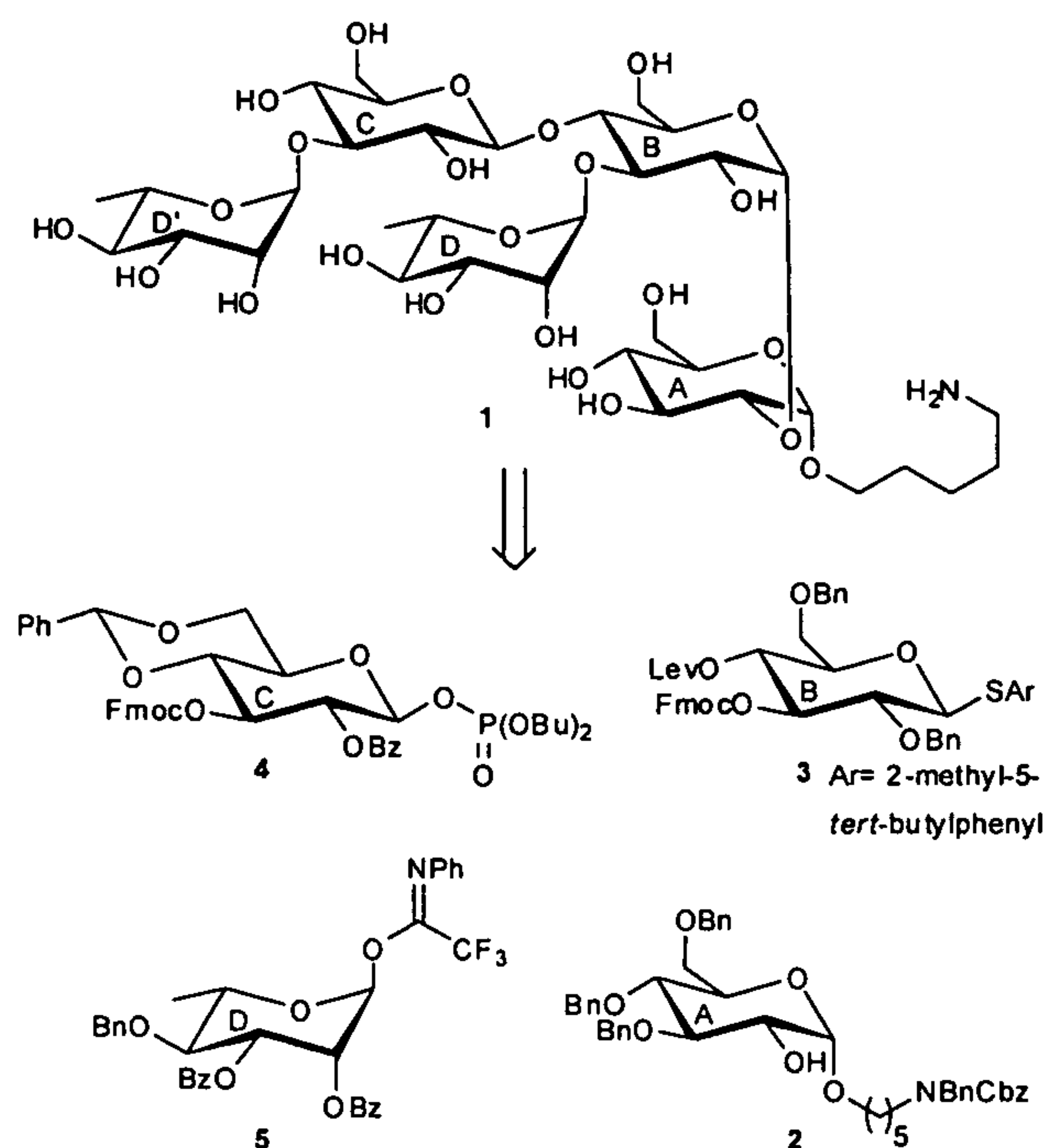
Scheme 1. Retrosynthetic analysis of pentasaccharide 1 .
