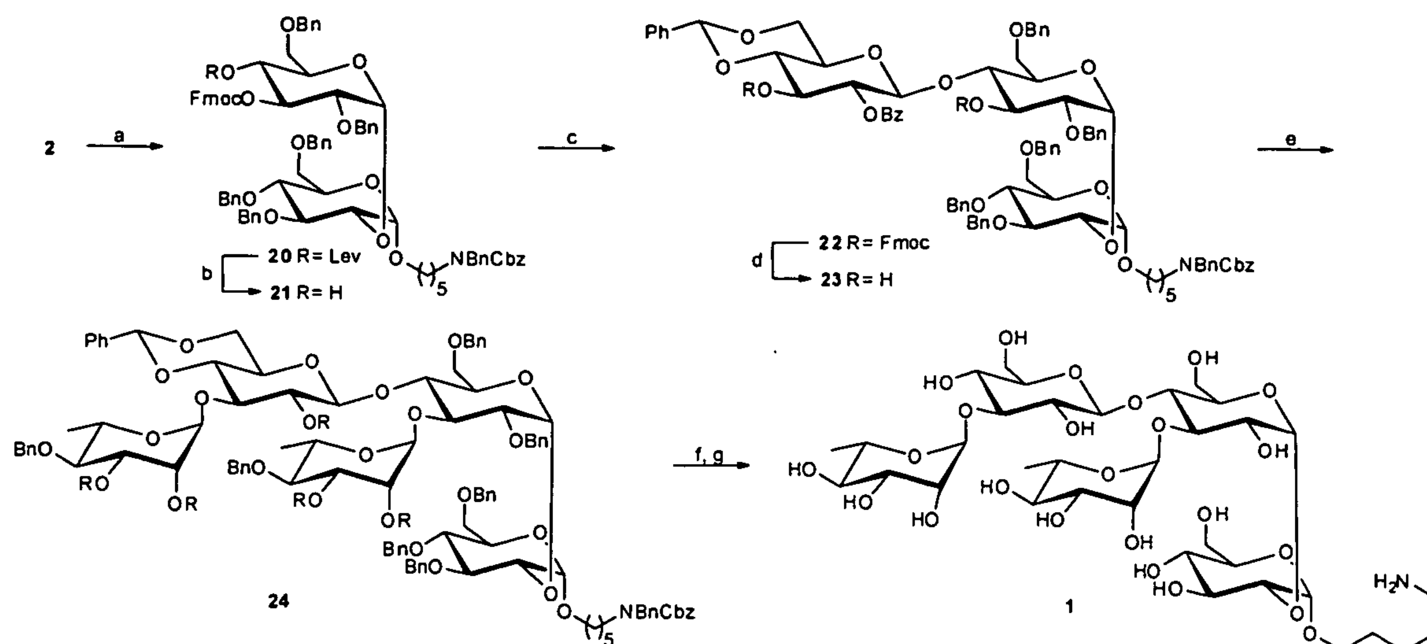
Scheme 5. Synthesis of 1 according to method A. Reagents and conditions: a) 3 , NIS/TfOH, Et 2 O, -35 °C to -10°C, 70%; b) N 2 H 4 ·H 2 O, AcOH/pyridine, DCM, 94%; c) 4 , TMSOTf, DCM, 4Å MS, -35 °C to -7 °C; d) NEt 3 , DCM, rt, 38% over 2 steps; e) 5 , TMSOTf, DCM, 4Å MS, -30 °C to -15 °C, 81%; f) NaOMe, THF/MeOH, 50 °C; g) H 2 , 10% Pd/C, MeOH, H 2 O,
