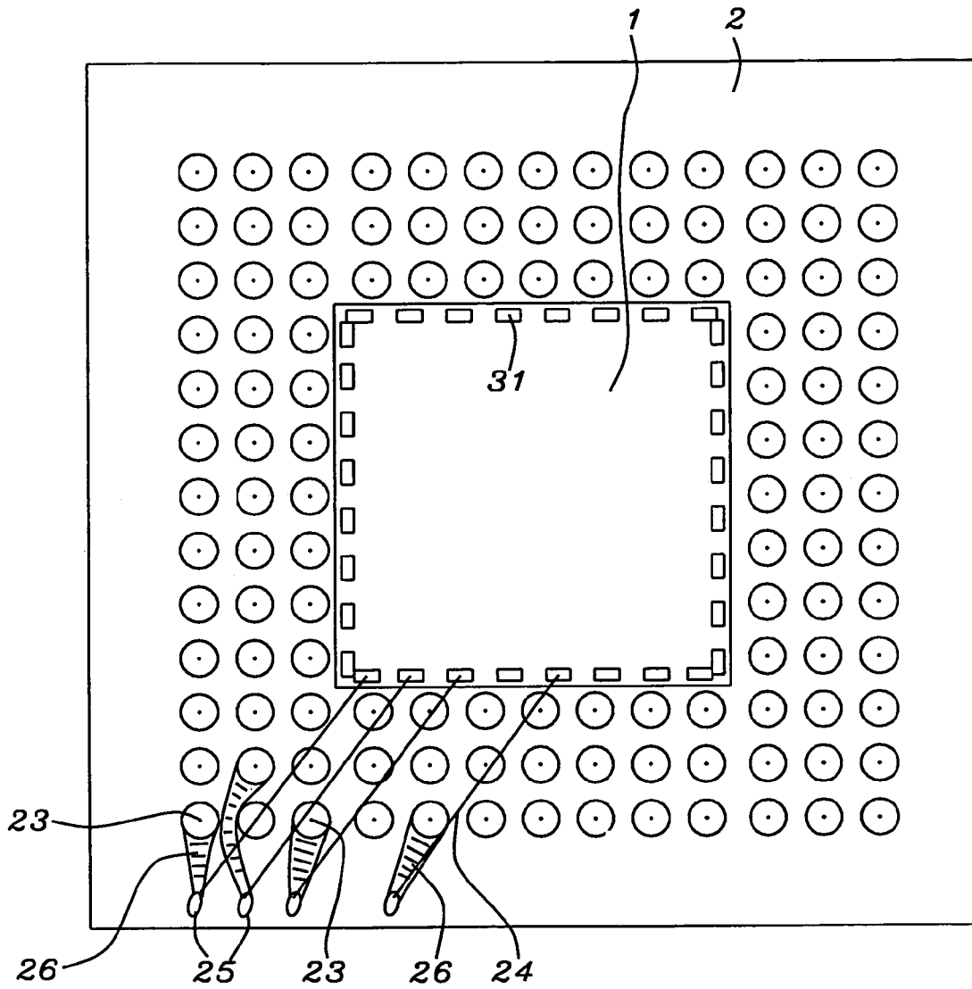
FIG. 3 - Prior Art
