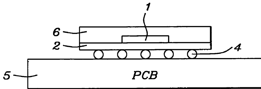
FIG. 1 - Prior Art
