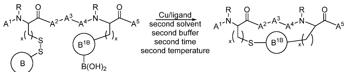
Scheme 2c
