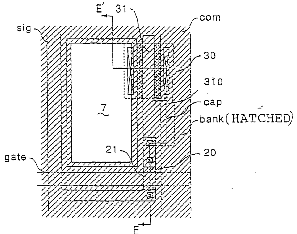
(B) SECTION E-E'
