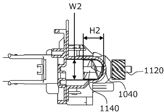
B1-B2 CROSS-SECTION
