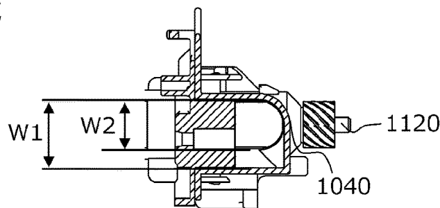
B1-B2 CROSS-SECTION
