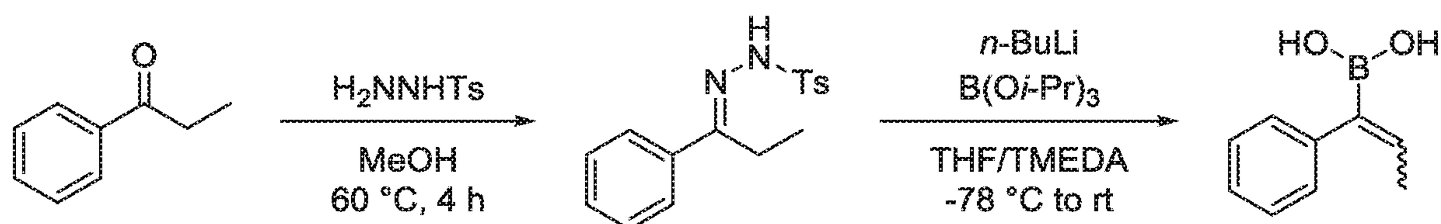
Scheme 3
