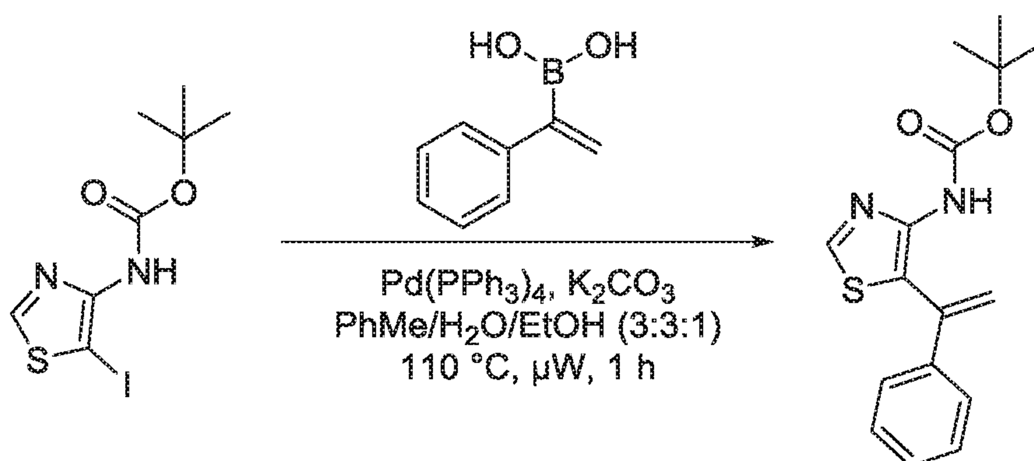
Scheme 4
