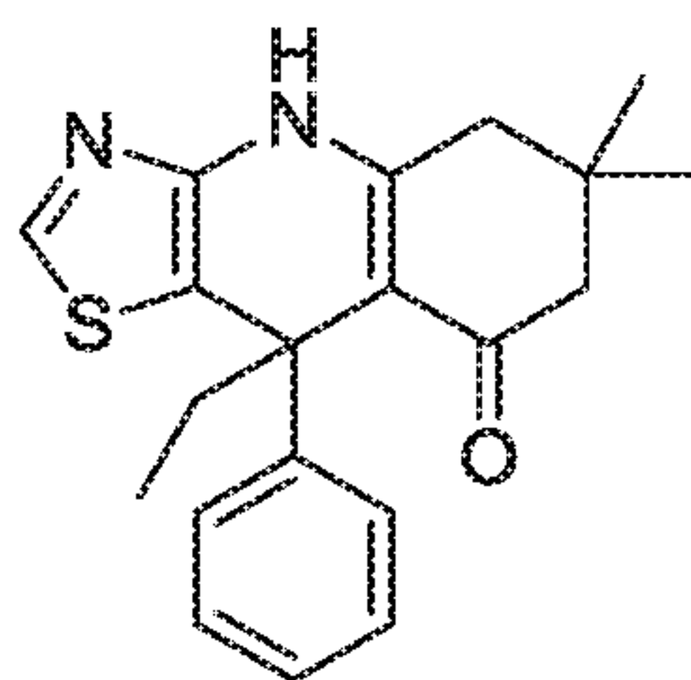
(1-rac),
