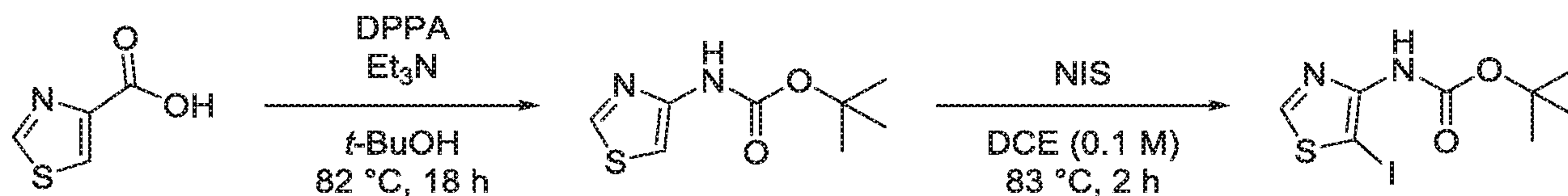
Scheme 2
