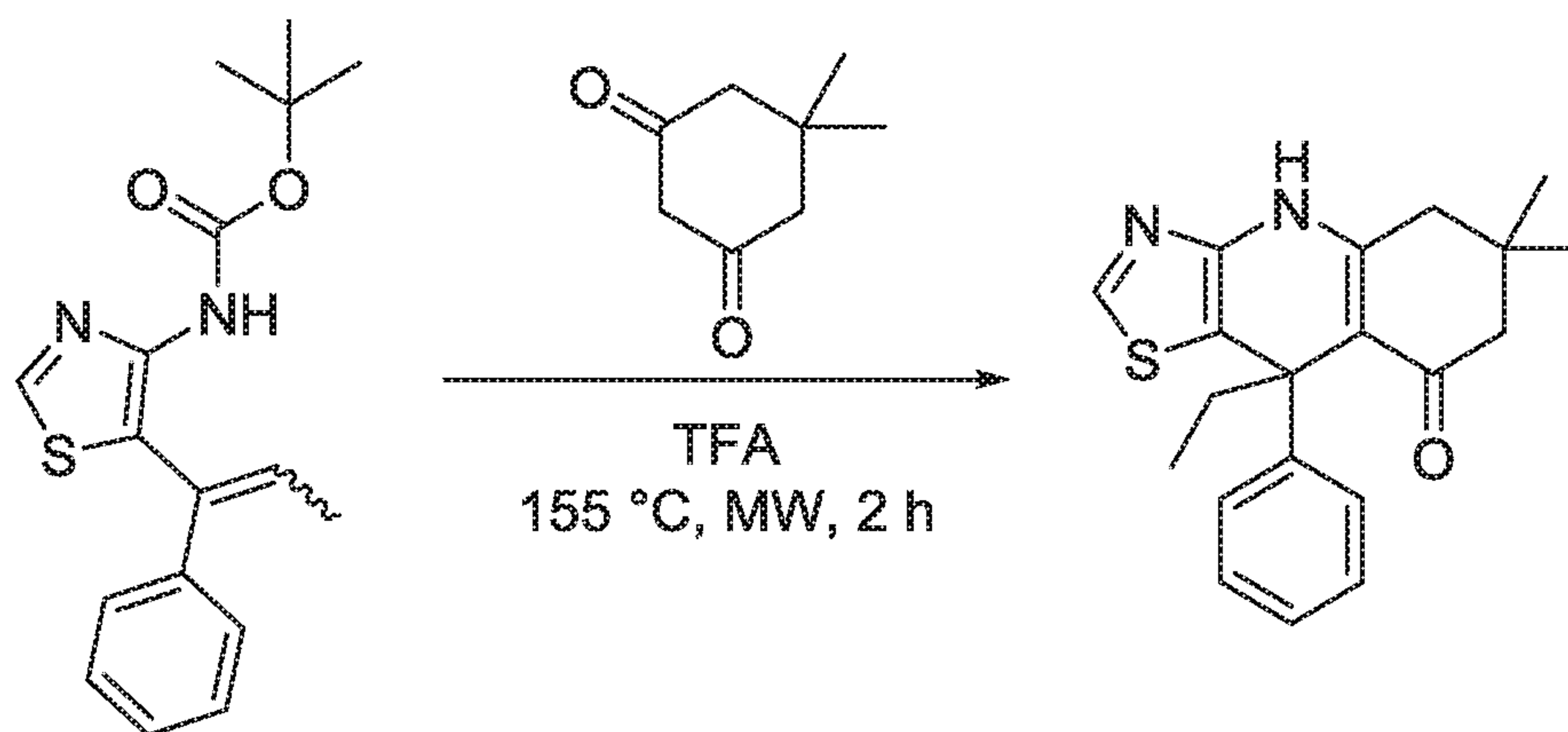
Scheme 6
