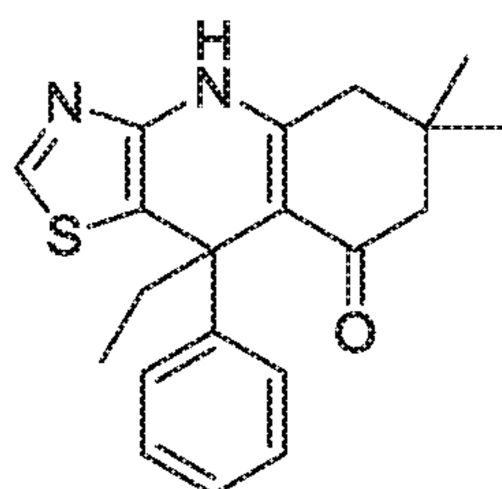
(1-rac),
