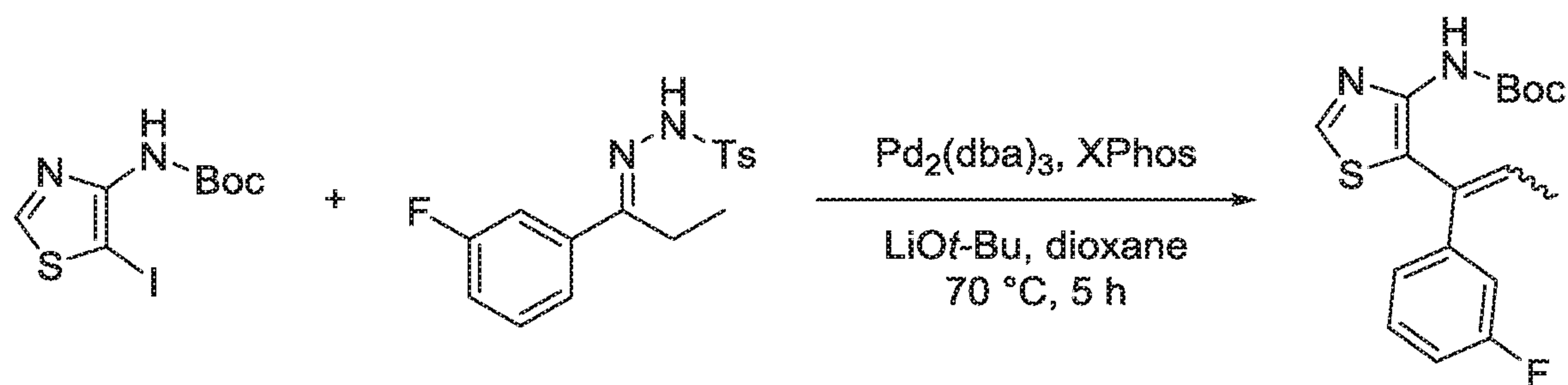
Scheme 5
