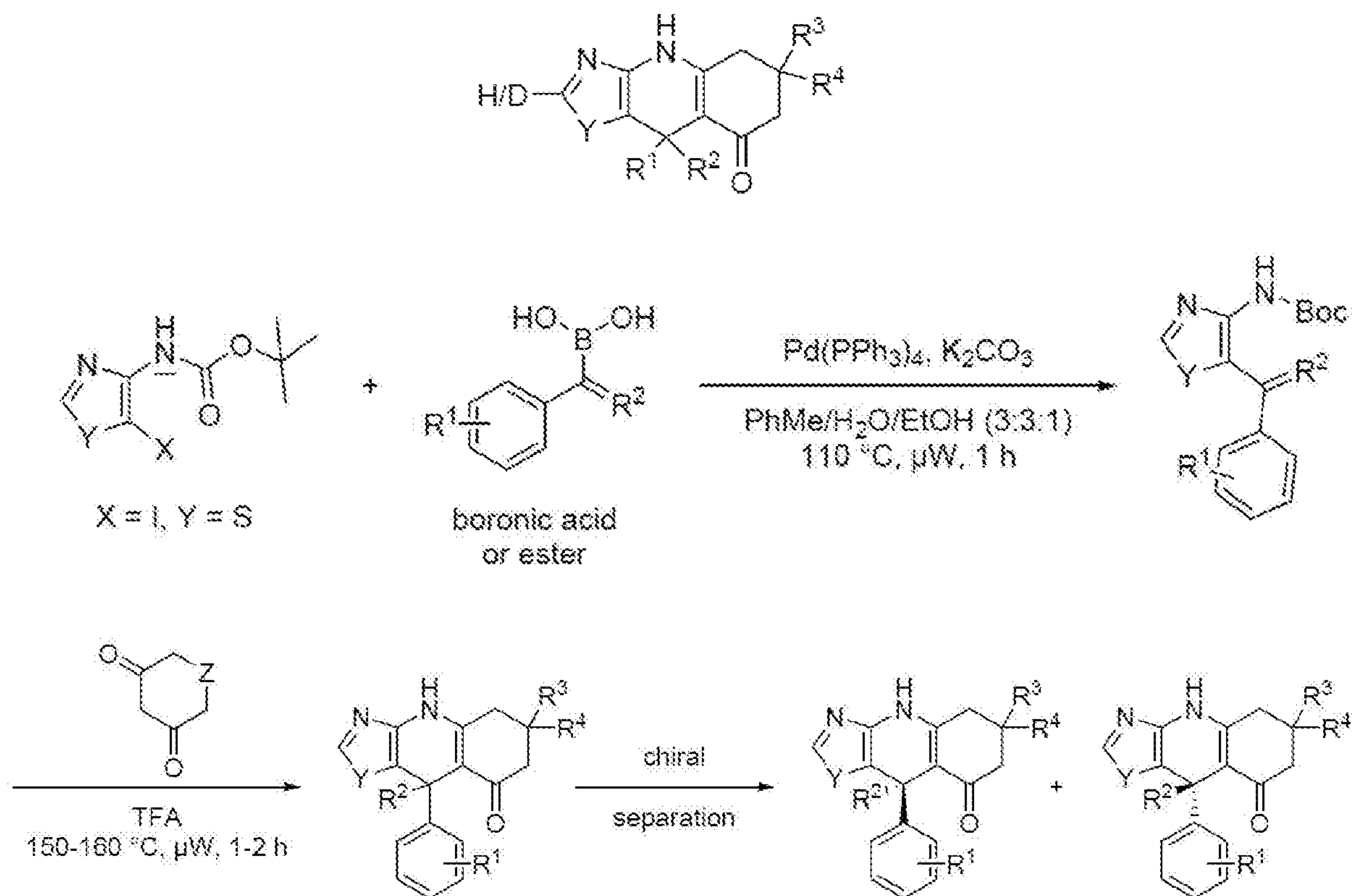
Scheme 1
