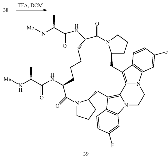
Scheme XIX
