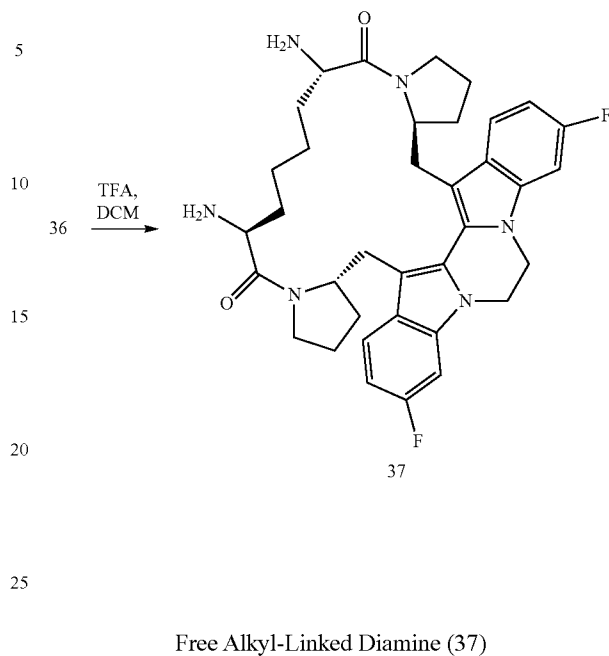
Scheme XVII
