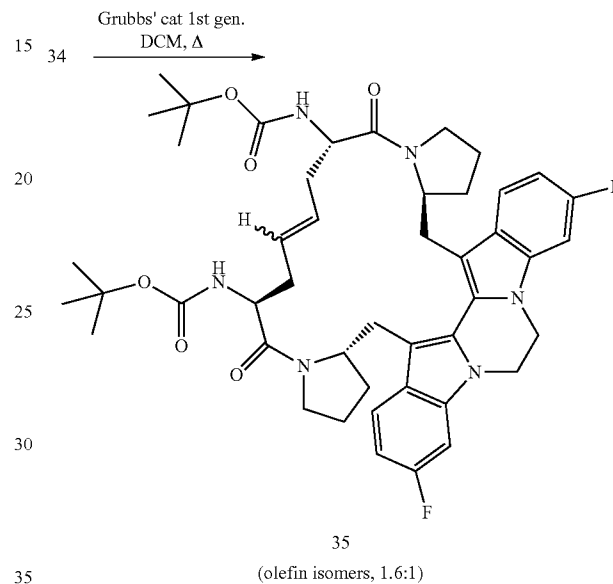
Scheme XV
