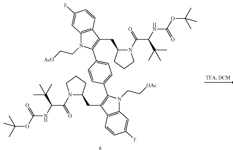
Scheme IV
