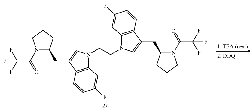
Scheme X
