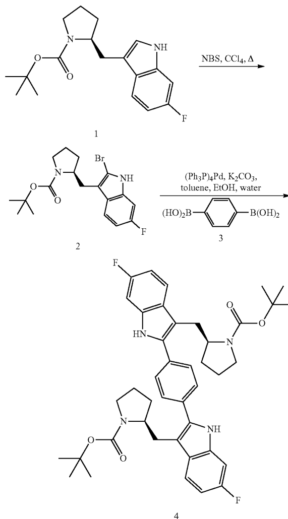
Scheme I
