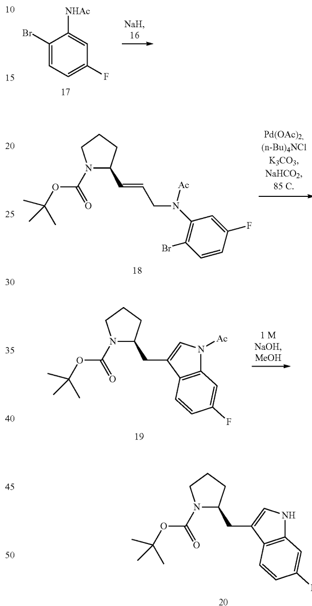
Scheme VII
