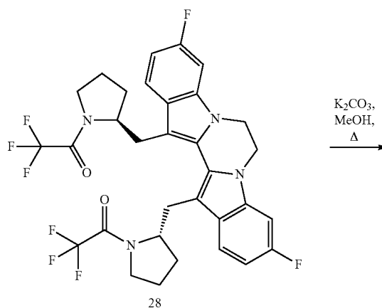
Scheme XI
