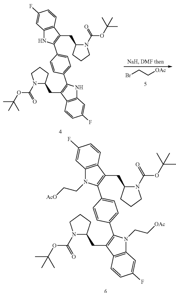
Scheme II
