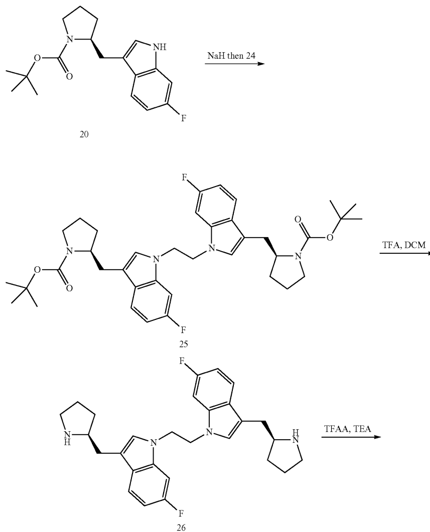
Scheme IX
