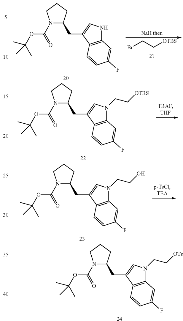
Scheme VIII
