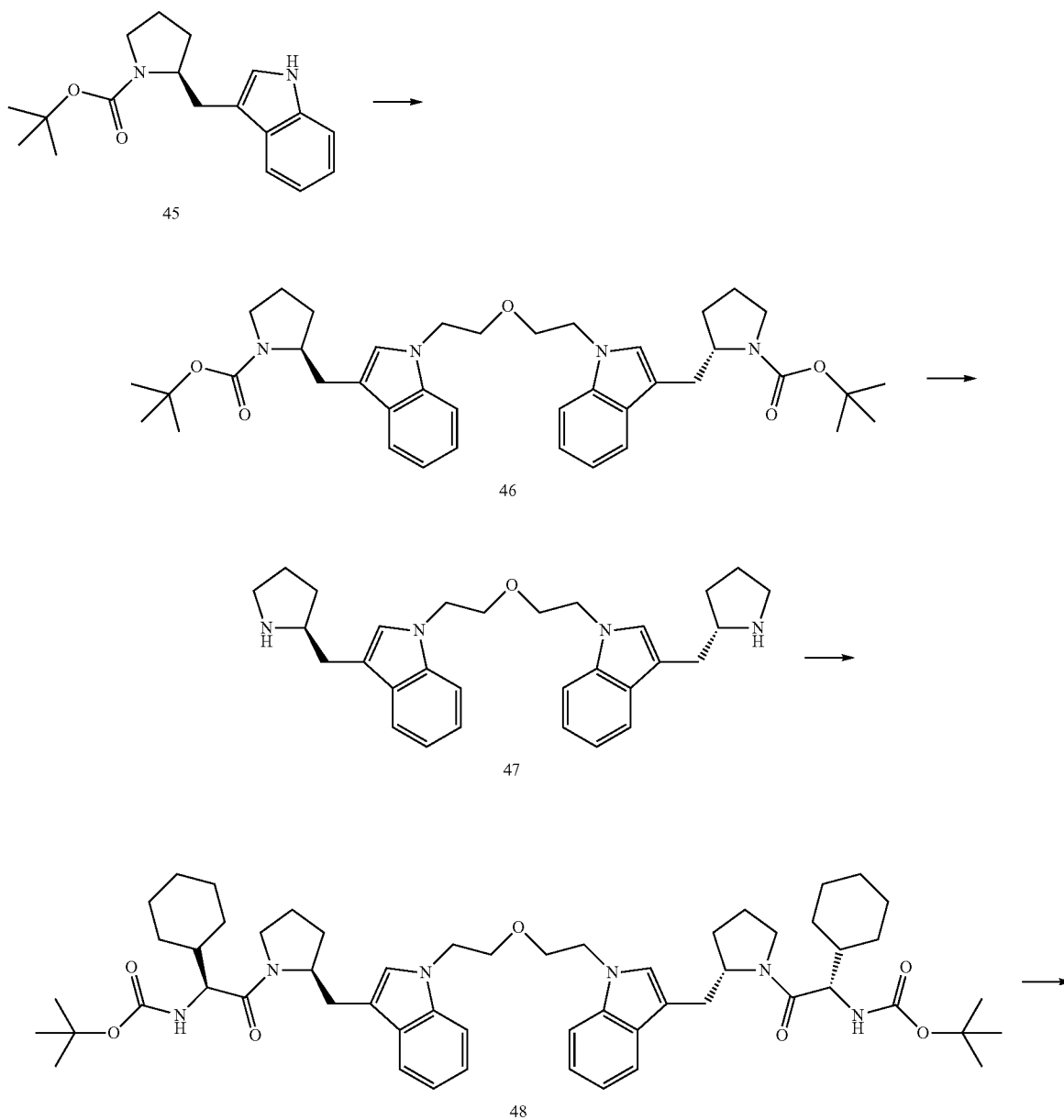
Scheme XXI
