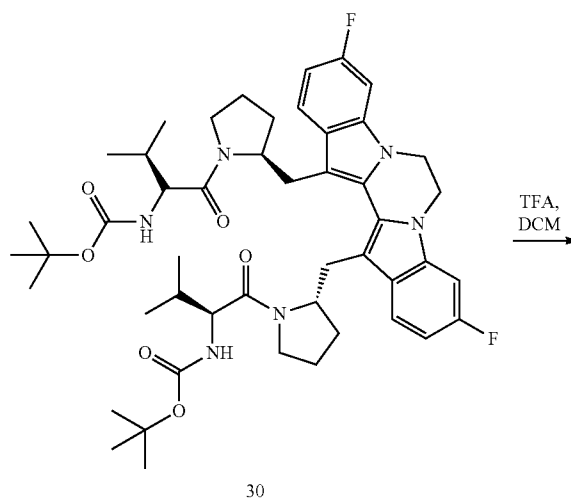
Scheme XII
