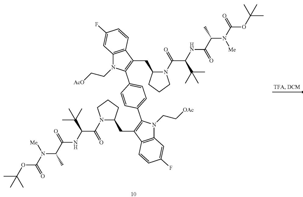
Scheme V
