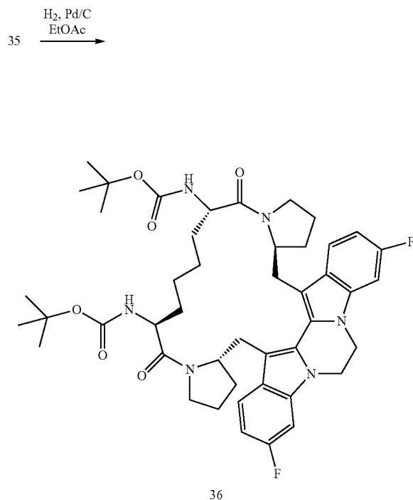
Scheme XVI
