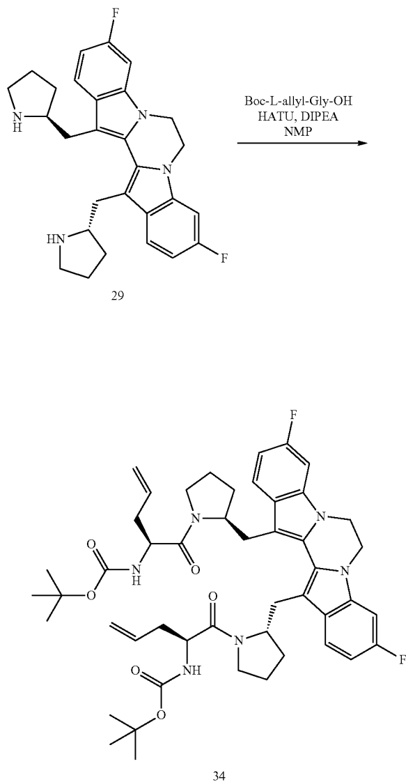
Scheme XIV
