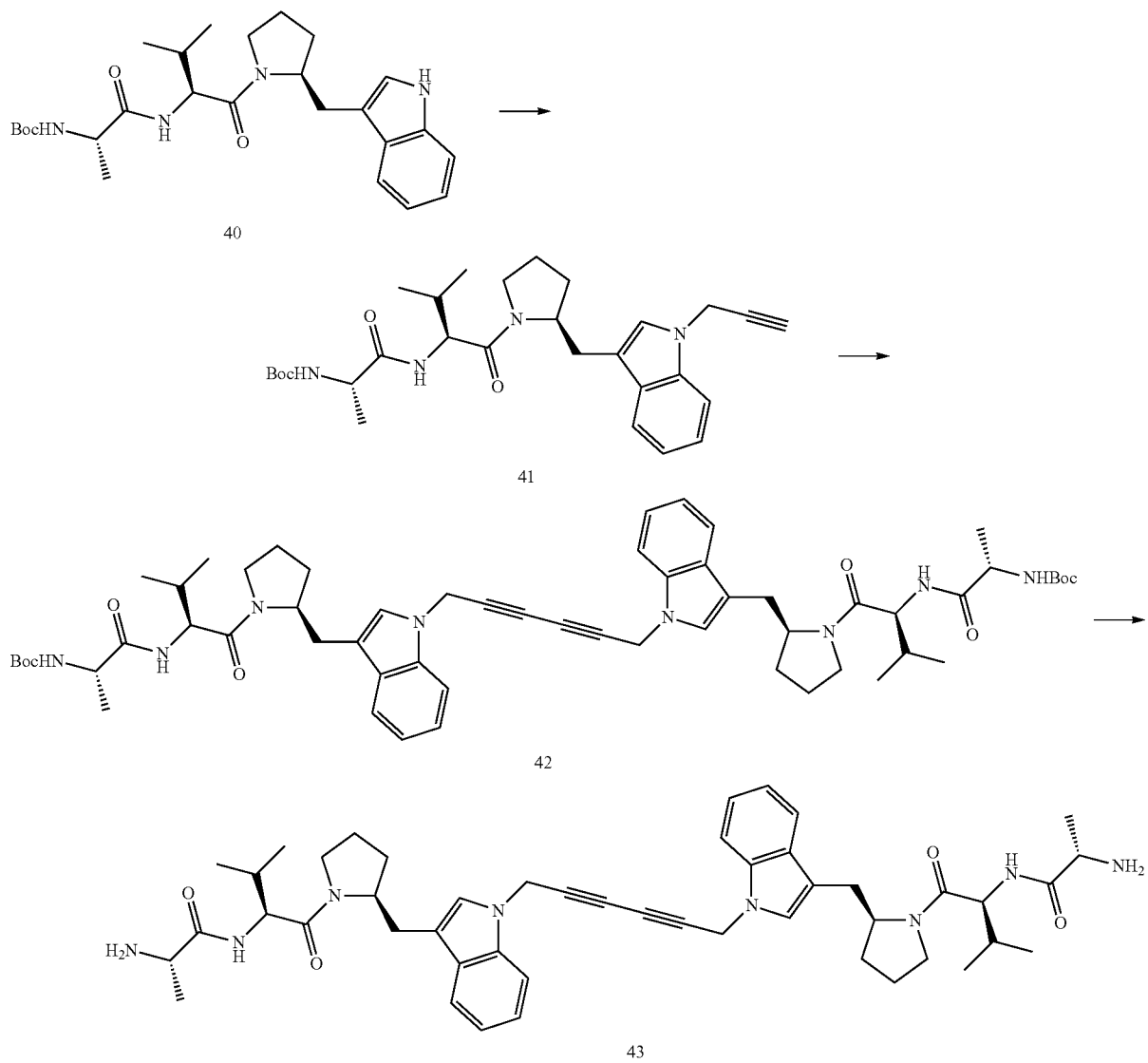
Scheme XX
