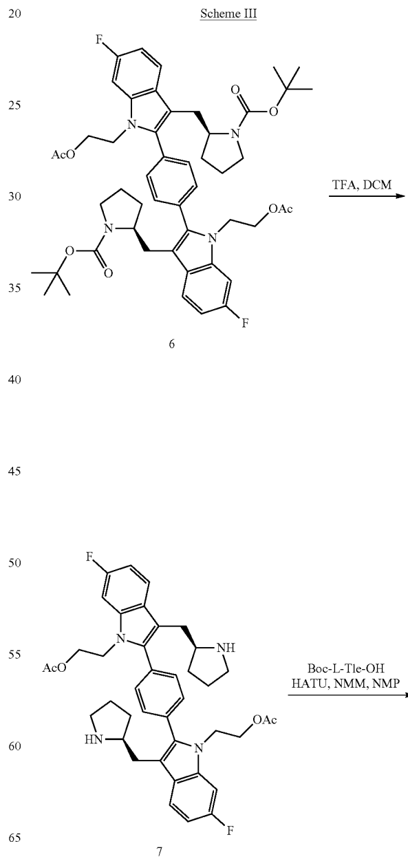
Scheme III
