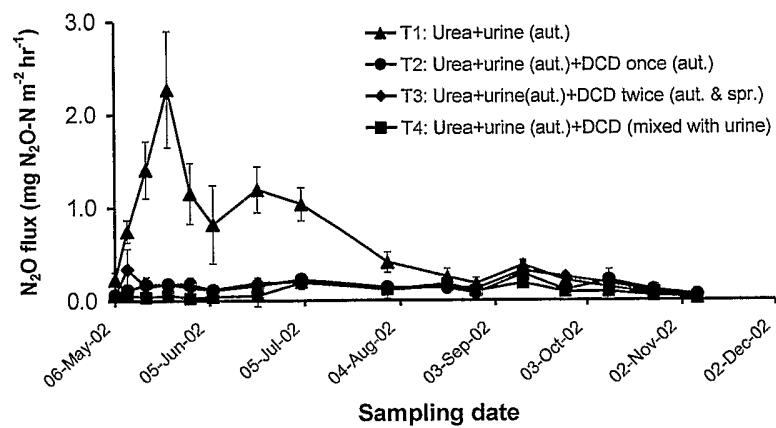
Figure 4. Nitrous oxide emissions from animal urine patches as affected by the treatments measured on the lysimeters, with and without a nitrification inhibitor (DCD).
