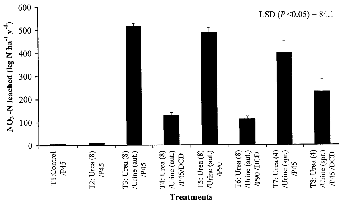
Figure 1. Total annual \text{NO}_3^- -N leached from the treatments as measured on the lysimeters, with and without a nitrification inhibitor (DCD).
