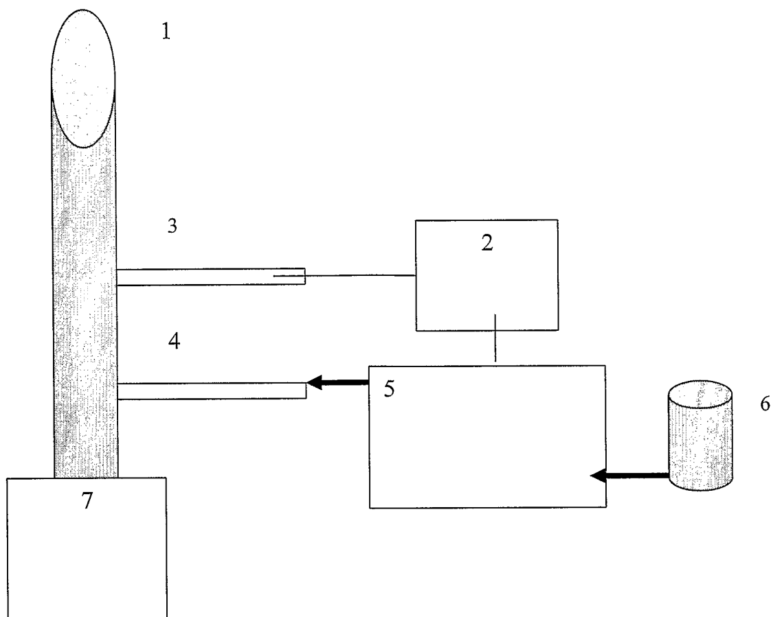
Figure 8. Pumping System for delivery of a nitrification inhibitor through an irrigation system
