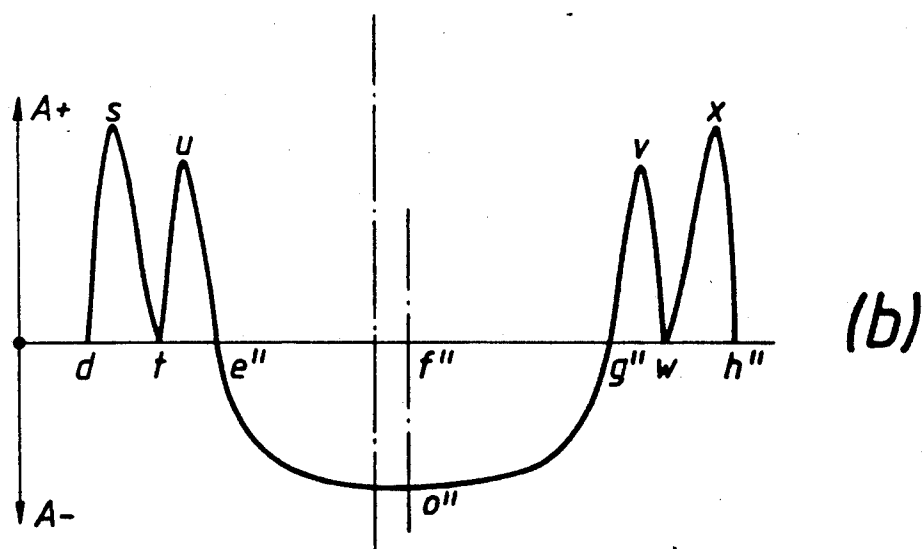
Fig. 5. PRIOR ART
