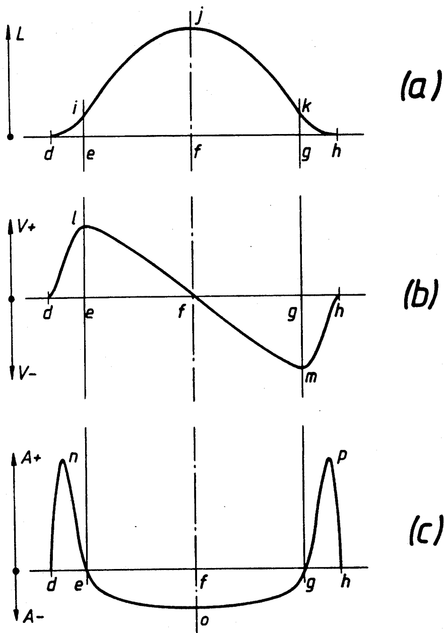
Fig.4. PRIOR ART
