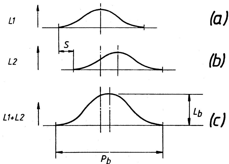
Fig. 3. PRIOR ART
