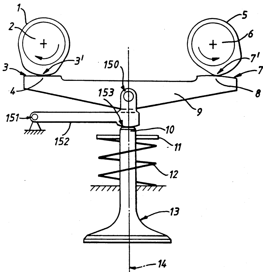
Fig.1. PRIOR ART
