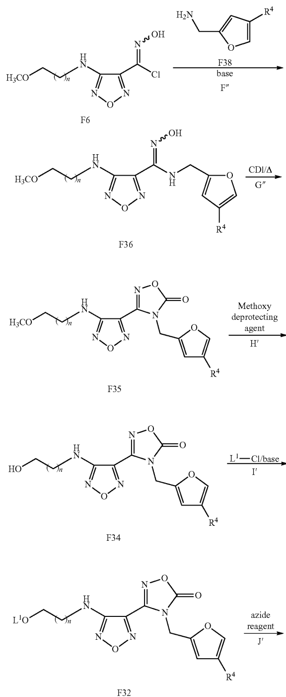
Scheme 9
