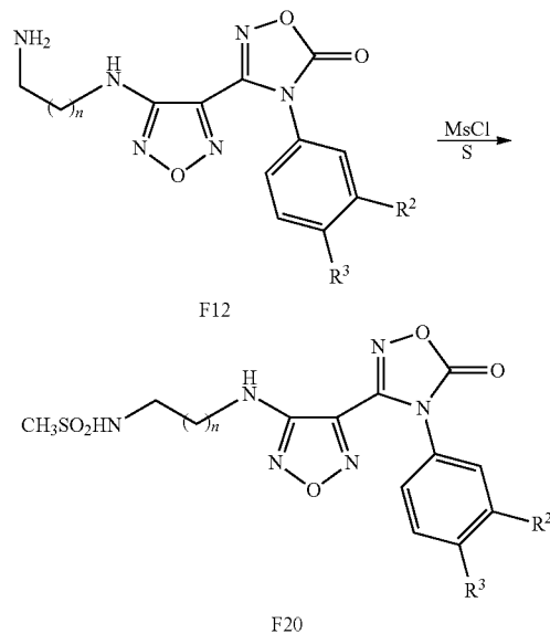
Scheme 7
