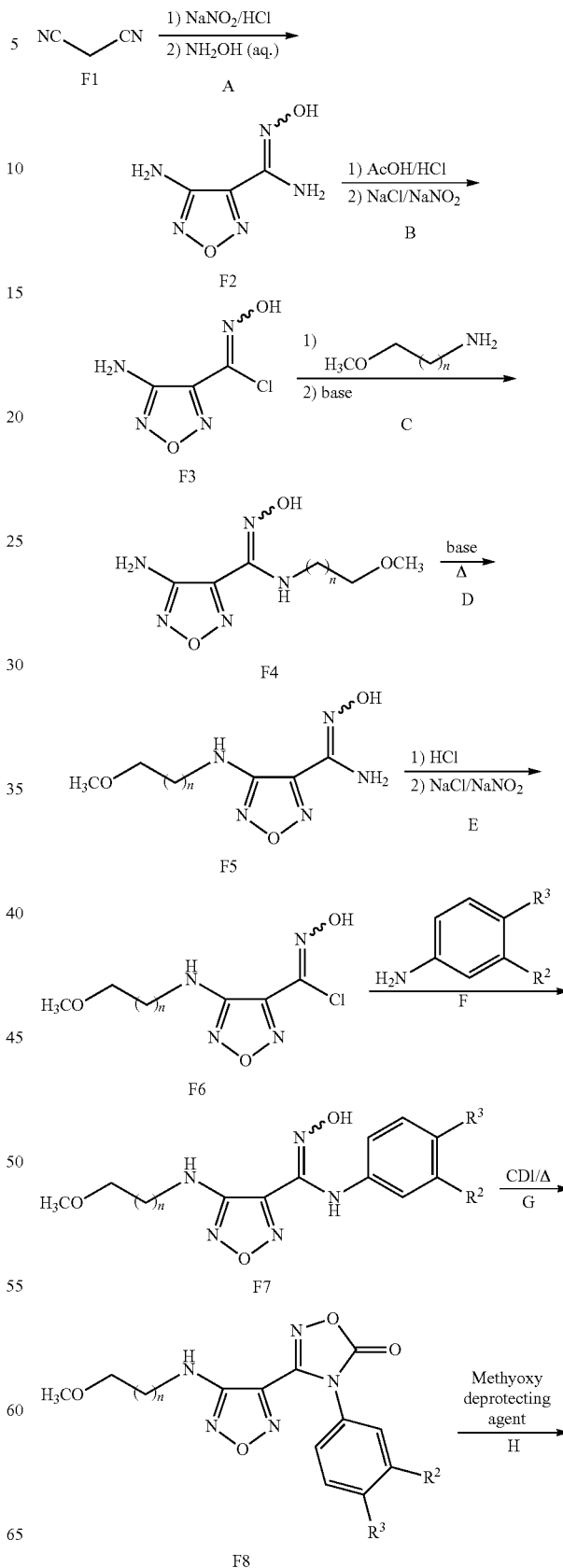
Scheme 3
