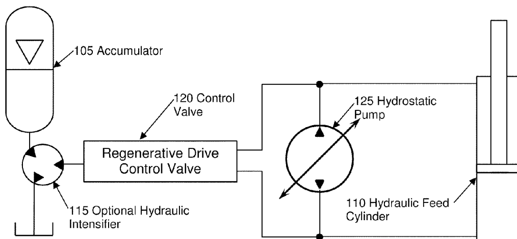
FIG. 2 PARALLEL HYDROSTATIC DRIVE UTILIZING FEED CYLINDER
