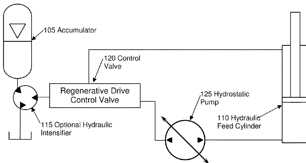
FIG. 3 SERIES HYDROSTATIC DRIVE UTILIZING FEED CYLINDER
