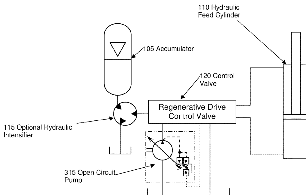
FIG. 4 OPEN CIRCUIT DRIVE UTILIZING FEED CYLINDER
