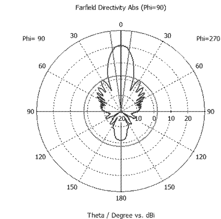
Antenna Gain Pattern
